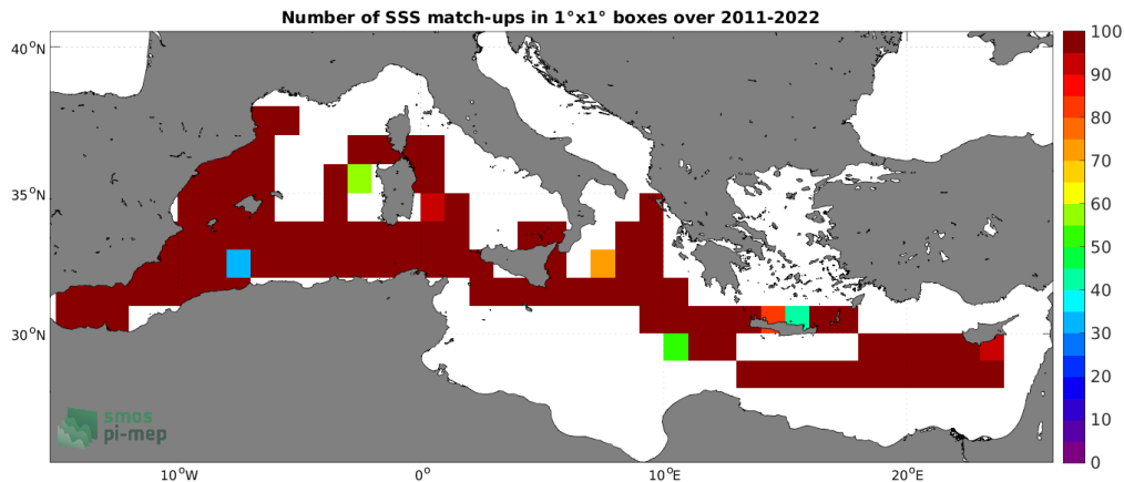
Figure 4: Number of SSS match-ups between TSG (CSIC-UTM) SSS and the SMOS SSS L4 OI v342 - Weekly (CMEMS-CATDS-LOPS) SSS product for the Mediterranean Sea Pi-MEP region over 1^\circ \times 1^\circ boxes and for the full satellite product period.
