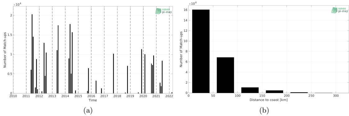
Figure 1: Number of match-ups between TSG (CSIC-UTM) and SMOS SSS L4 OI v342 - Weekly (CMEMS-CATDS-LOPS) SSS as a function of time (a) and as function of the distance to coast (b) over the Mediterranean Sea Pi-MEP region and for the full satellite product period.
