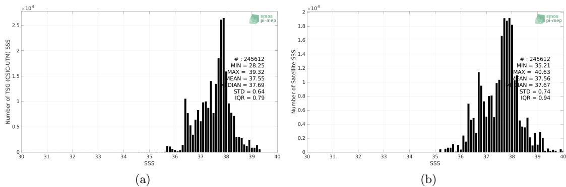
Figure 2: Histograms of SSS from TSG (CSIC-UTM) (a) and SMOS SSS L4 OI v342 - Weekly (CMEMS-CATDS-LOPS) (b) considering all match-up pairs per bins of 0.1 over the Mediterranean Sea Pi-MEP region and for the full satellite product period.
