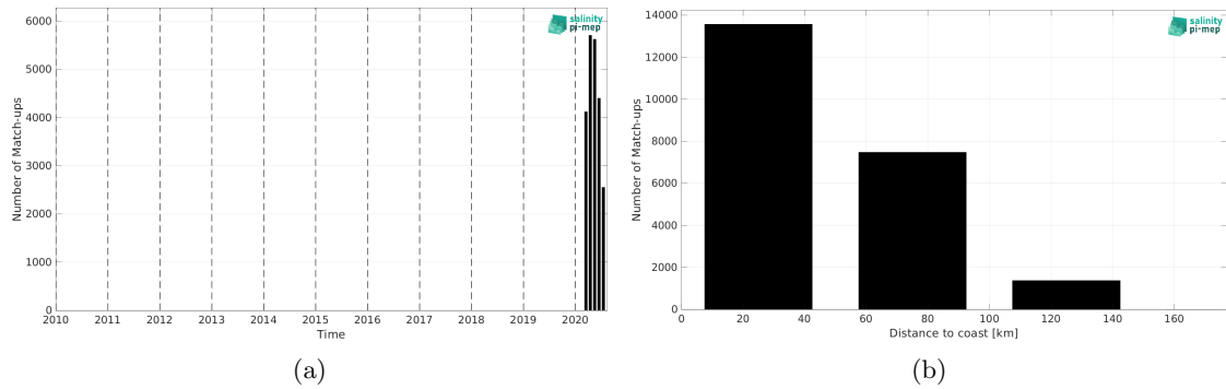
Figure 1: Number of match-ups between Saildrone and SMOS SSS L4 OI v342 - Weekly (CMEMS-CATDS-LOPS) SSS as a function of time (a) and as function of the distance to coast (b) over the Mediterranean Sea Pi-MEP region and for the full satellite product period.
