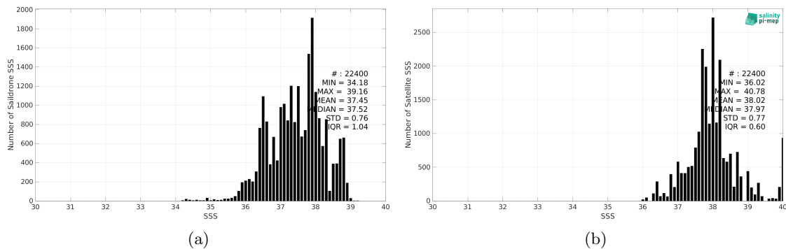
Figure 2: Histograms of SSS from Saildrone (a) and SMOS SSS L4 OI v342 - Weekly (CMEMS-CATDS-LOPS) (b) considering all match-up pairs per bins of 0.1 over the Mediterranean Sea Pi-MEP region and for the full satellite product period.
