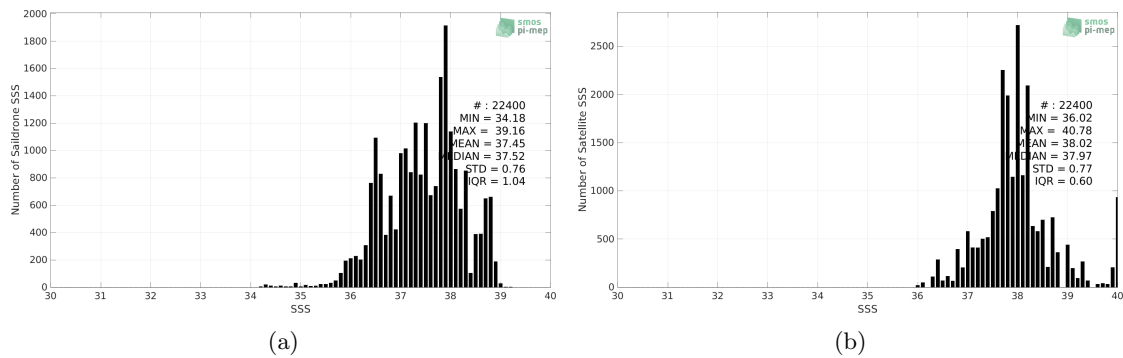
Figure 2: Histograms of SSS from Sairdrone (a) and SMOS SSS L4 OI v342 - Weekly (CMEMS-CATDS-LOPS) (b) considering all match-up pairs per bins of 0.1 over the Mediterranean Sea Pi-MEP region and for the full satellite product period.
