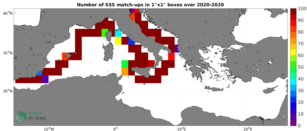
Figure 4: Number of SSS match-ups between Saildrone SSS and the SMOS SSS L4 OI v342 - Weekly (CMEMS-CATDS-LOPS) SSS product for the Mediterranean Sea Pi-MEP region over 1^\circ \times 1^\circ boxes and for the full satellite product period.
