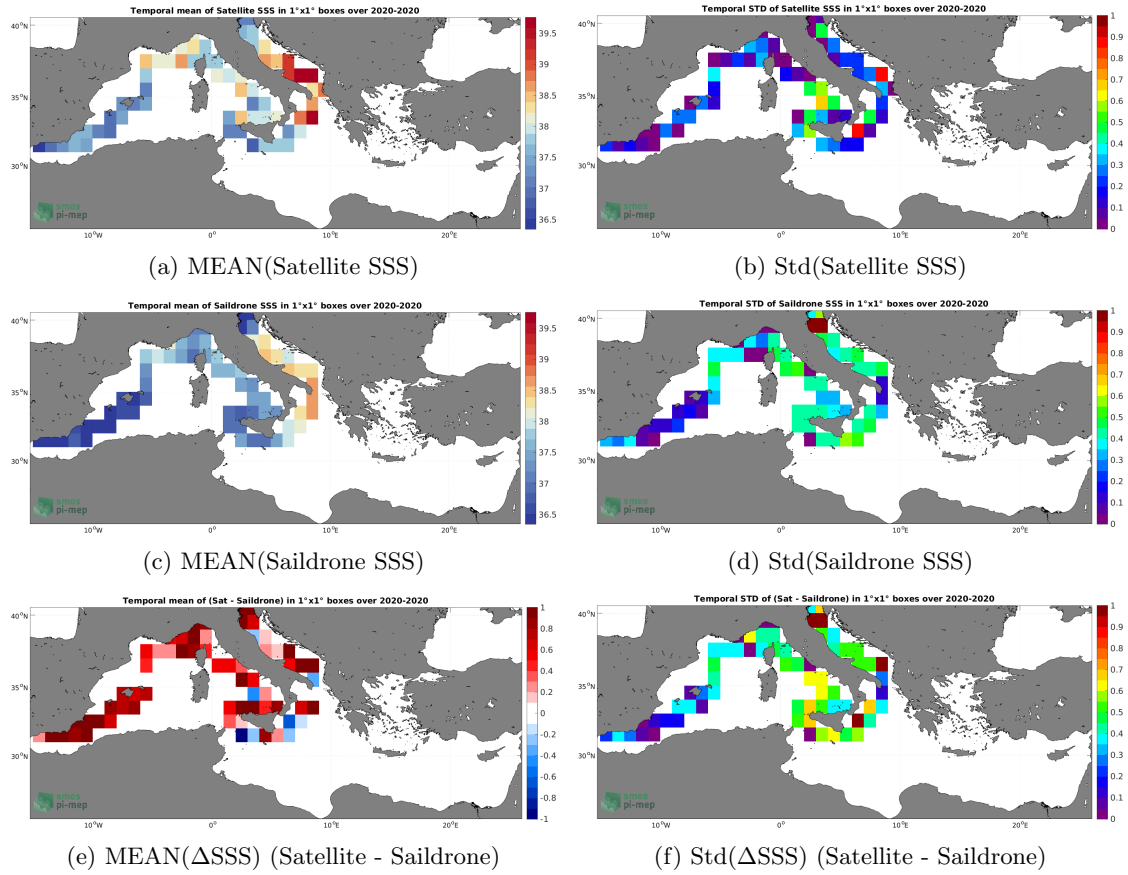
Figure 6: Temporal mean (left) and Std (right) of SSS from SMOS SSS L4 OI v342 - Weekly (CMEMS-CATDS-LOPS) (top), Saildrone (middle), and of \Delta SSS (Satellite - Saildrone). Only match-up pairs are used to generate these maps.
