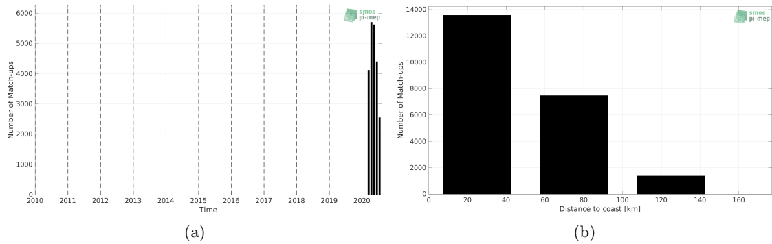
Figure 1: Number of match-ups between Sairdrone and SMOS SSS L4 OI v342 - Weekly (CMEMS-CATDS-LOPS) SSS as a function of time (a) and as function of the distance to coast (b) over the Mediterranean Sea Pi-MEP region and for the full satellite product period.
