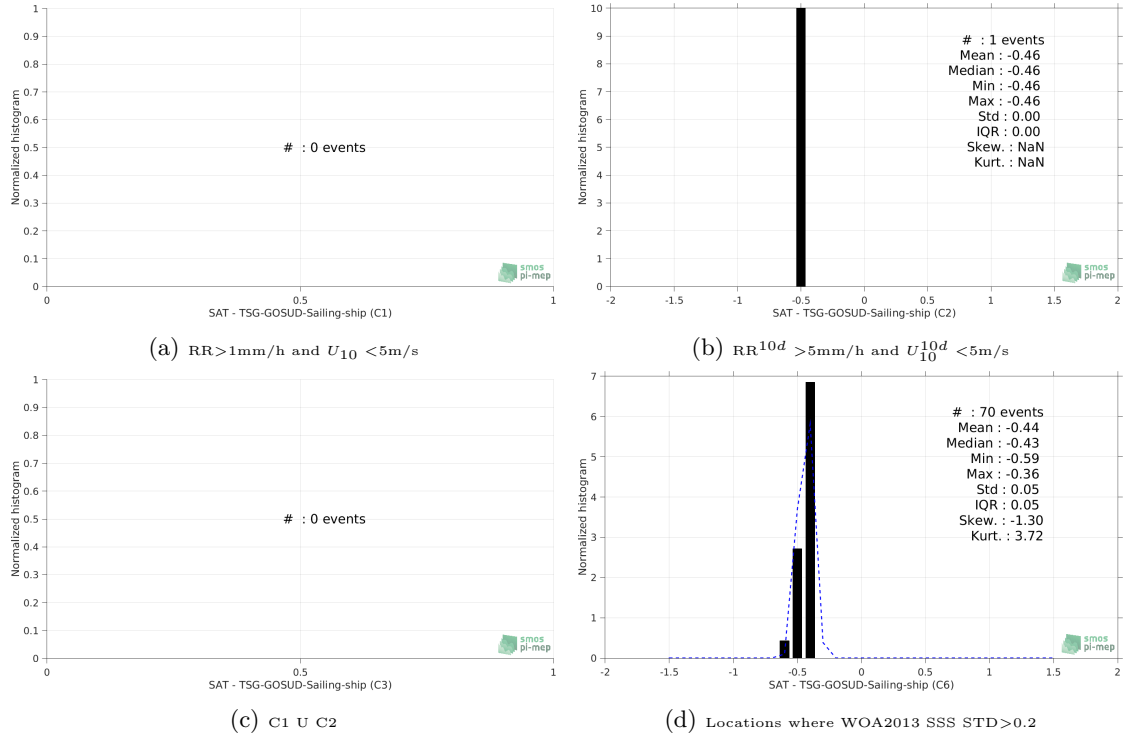
Figure 13: Normalized histogram of \Delta\text{SSS} (SMOS-L4-CATDS-CECOS-IFREMER-V2-WEEKLY-0.5DEG - TSG-GOSUD-Sailing-ship) for 6 different subdatasets corresponding to: RR > 1\text{mm/h} and U_{10} < 5\text{m/s} (a), RR^{10d} > 5\text{mm/h} and U_{10}^{10d} < 5\text{m/s} (b), C1 U C2 (c), Locations where WOA2013 SSS STD > 0.2 (d).
