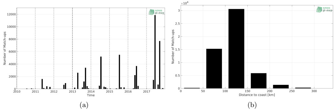
Figure 1: Number of match-ups between TSG (GOSUD-Research-vessel) and SMOS L4 v2 Weekly (CATDS-CECOS-IFREMER) SSS as a function of time (a) and as function of the distance to coast (b) over the Mediterranean Sea Pi-MEP region and for the full satellite product period.
