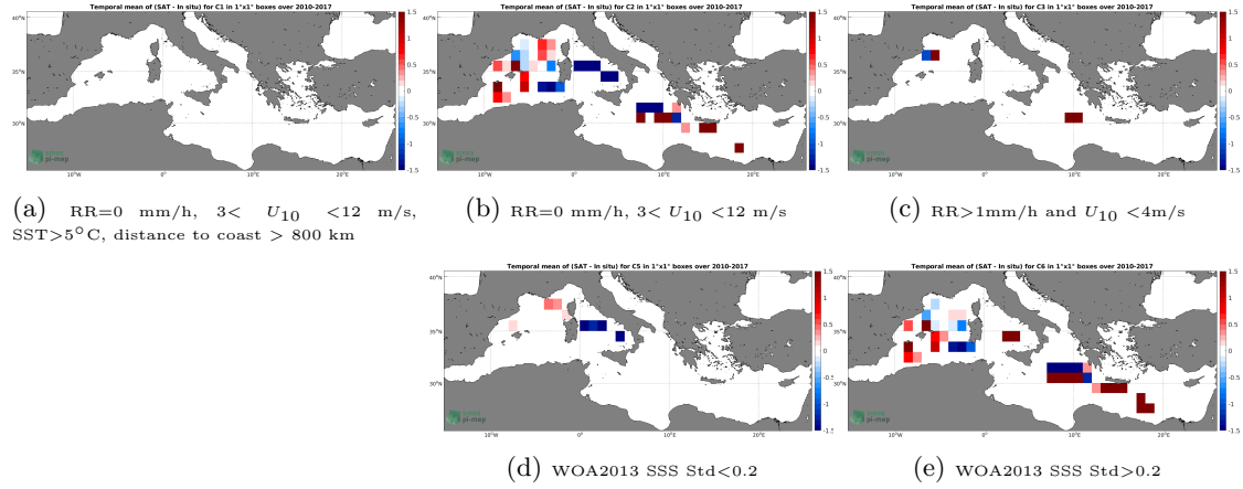
Figure 12: Temporal mean gridded over spatial boxes of size 1^\circ \times 1^\circ of \Delta SSS (SMOS L4 v2 Weekly (CATDS-CECOS-IFREMER) - TSG (GOSUD-Research-vessel)) for 5 different subdatasets corresponding to: RR=0 mm/h, 3 < U_{10} < 12 m/s, SST > 5^\circ\text{C} , distance to coast > 800 km (a), RR=0 mm/h, 3 < U_{10} < 12 m/s (b), RR > 1 mm/h and U_{10} < 4 m/s (c), WOA2013 SSS Std < 0.2 (d), WOA2013 SSS Std > 0.2 (e).
