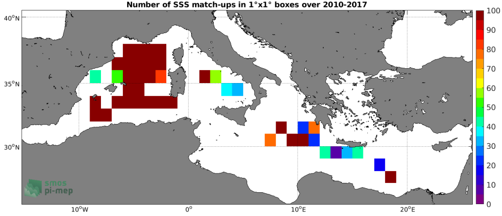
Figure 4: Number of SSS match-ups between TSG (GOSUD-Research-vessel) SSS and the SMOS L4 v2 Weekly (CATDS-CECOS-IFREMER) SSS product for the Mediterranean Sea Pi-MEP region over 1^\circ \times 1^\circ boxes and for the full satellite product period.
