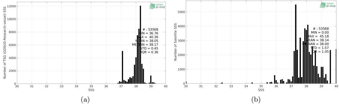
Figure 2: Histograms of SSS from TSG (GOSUD-Research-vessel) (a) and SMOS L4 v2 Weekly (CATDS-CECOS-IFREMER) (b) considering all match-up pairs per bins of 0.1 over the Mediterranean Sea Pi-MEP region and for the full satellite product period.
