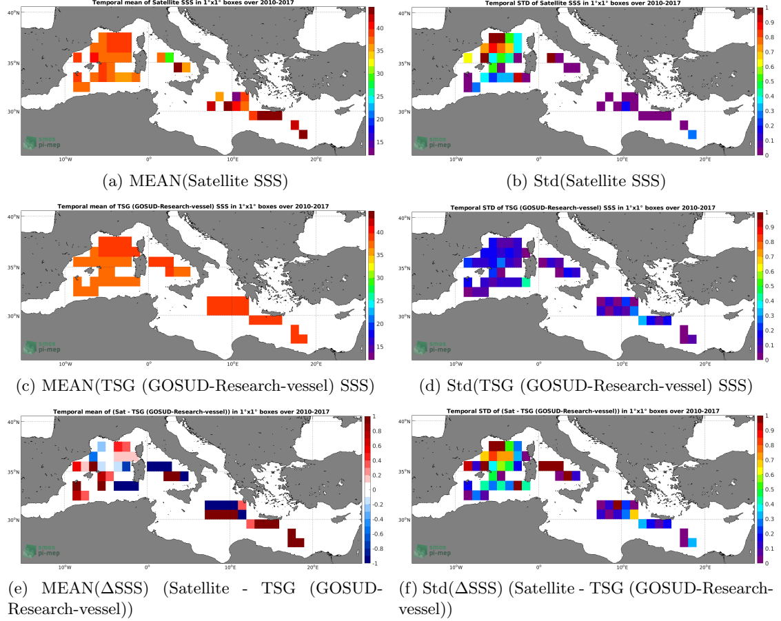
Figure 6: Temporal mean (left) and Std (right) of SSS from SMOS L4 v2 Weekly (CATDS-CECOS-IFREMER) (top), TSG (GOSUD-Research-vessel) (middle), and of \Delta\text{SSS} (Satellite - TSG (GOSUD-Research-vessel)). Only match-up pairs are used to generate these maps.
