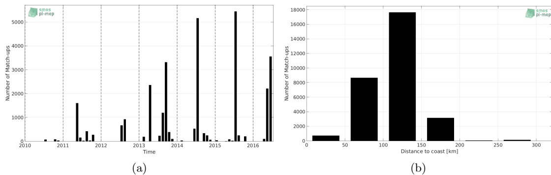
Figure 1: Number of match-ups between TSG-GOSUD-Research-vessel and SMOS-L4-CATDS-CECOS-IFREMER-V2-WEEKLY-0.5DEG SSS as a function of time (a) and as function of the distance to coast (b) over the Mediterranean Sea Pi-MEP region and for the full satellite product period.
