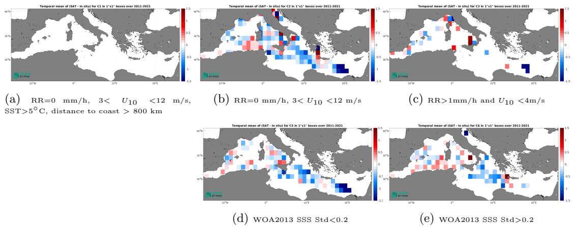
Figure 14: Temporal mean gridded over spatial boxes of size 1^\circ \times 1^\circ of \Delta SSS (SMOS SSS L4 v2 - Daily (BEC) - TSG (LEGOS-DM)) for 5 different subdatasets corresponding to:RR=0 mm/h, 3 < U_{10} < 12 m/s, SST>5°C, distance to coast > 800 km (a), RR=0 mm/h, 3 < U_{10} < 12 m/s (b), RR>1mm/h and U_{10} < 4 m/s (c), WOA2013 SSS Std<0.2 (d), WOA2013 SSS Std>0.2 (e).
