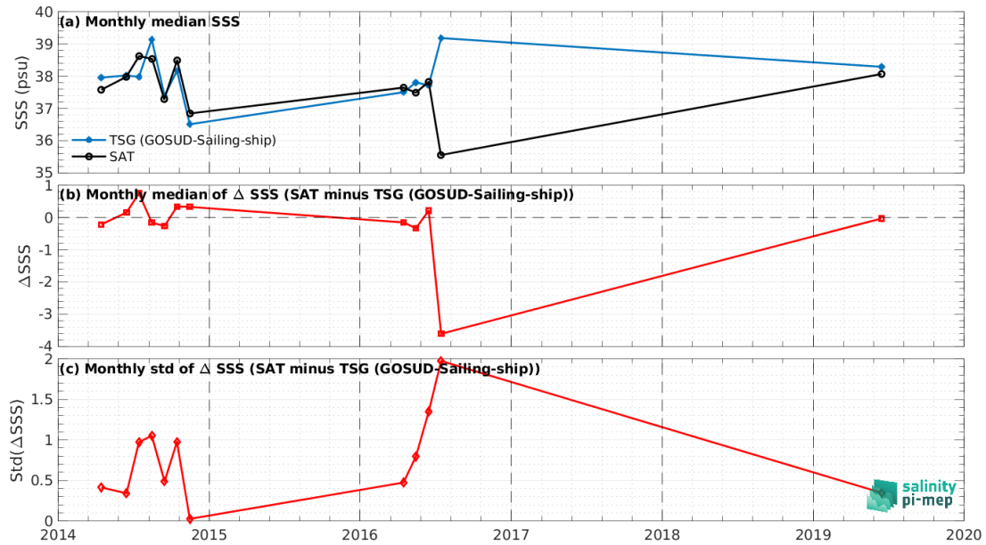
Figure 8: Time series of the monthly median SSS (top), median of \Delta\text{SSS} (Satellite - TSG (GOSUD-Sailing-ship)) and Std of \Delta\text{SSS} (Satellite - TSG (GOSUD-Sailing-ship)) over the Mediterranean Sea Pi-MEP region considering all match-ups collected by the Pi-MEP.
