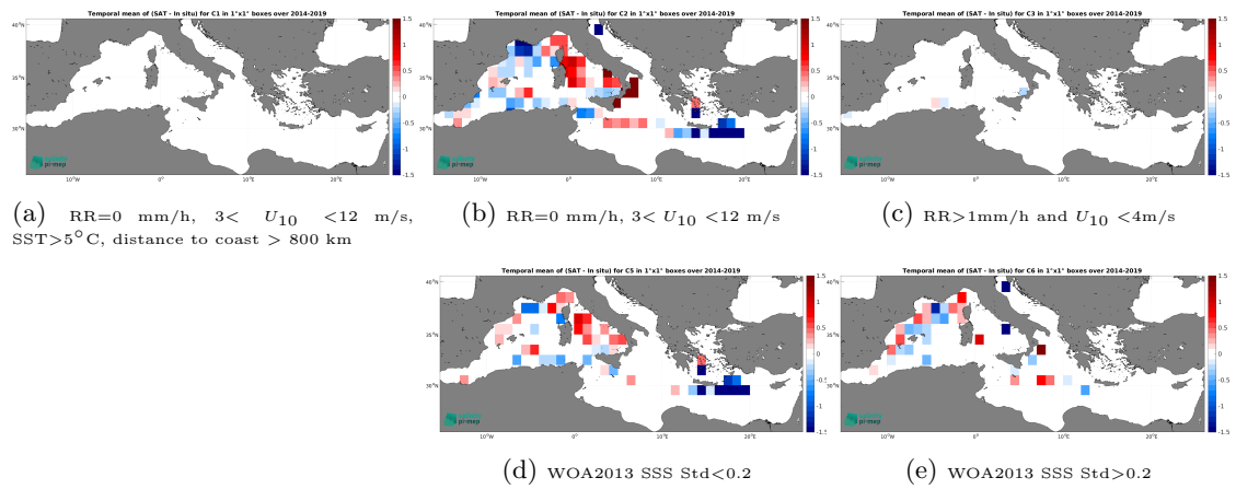
Figure 14: Temporal mean gridded over spatial boxes of size 1^\circ \times 1^\circ of \Delta SSS (SMOS SSS L4 v2 - Daily (BEC) - TSG (GOSUD-Sailing-ship)) for 5 different subdatasets corresponding to:RR=0 mm/h, 3 < U_{10} < 12 m/s, SST>5°C, distance to coast > 800 km (a), RR=0 mm/h, 3 < U_{10} < 12 m/s (b), RR>1mm/h and U_{10} < 4 m/s (c), WOA2013 SSS Std<0.2 (d), WOA2013 SSS Std>0.2 (e).
