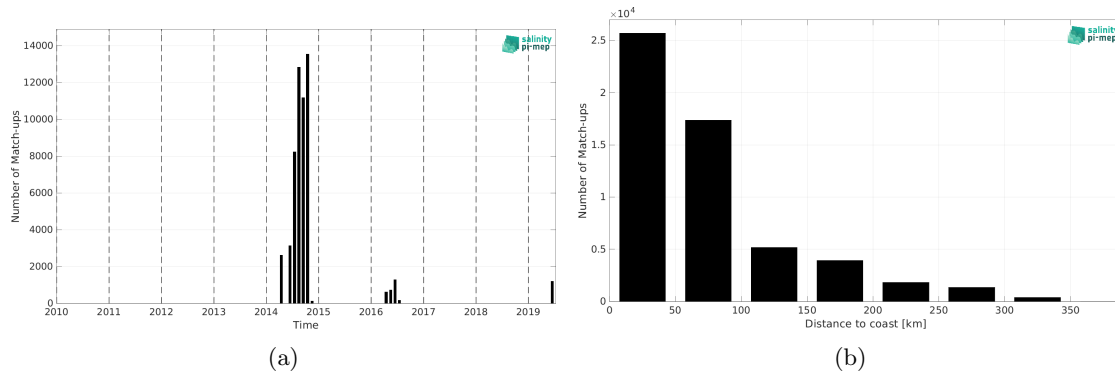
Figure 2: Number of match-ups between TSG (GOSUD-Sailing-ship) and SMOS SSS L4 v2 - Daily (BEC) SSS as a function of time (a) and as function of the distance to coast (b) over the Mediterranean Sea Pi-MEP region and for the full satellite product period.
