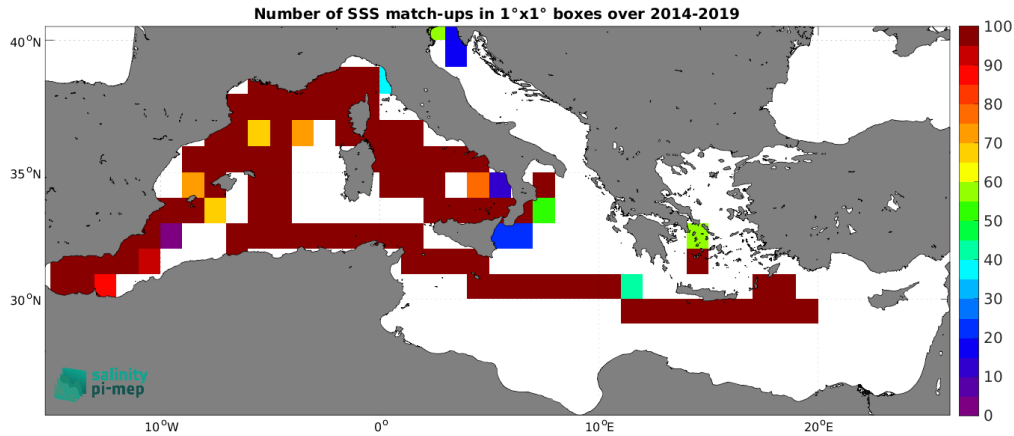
Figure 5: Number of SSS match-ups between TSG (GOSUD-Sailing-ship) SSS and the SMOS SSS L4 v2 - Daily (BEC) SSS product for the Mediterranean Sea Pi-MEP region over 1^\circ \times 1^\circ boxes and for the full satellite product period.
