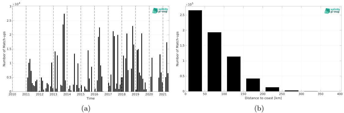
Figure 2: Number of match-ups between TSG (GOSUD-Research-vessel) and SMOS SSS L4 v2 - Daily (BEC) SSS as a function of time (a) and as function of the distance to coast (b) over the Mediterranean Sea Pi-MEP region and for the full satellite product period.
