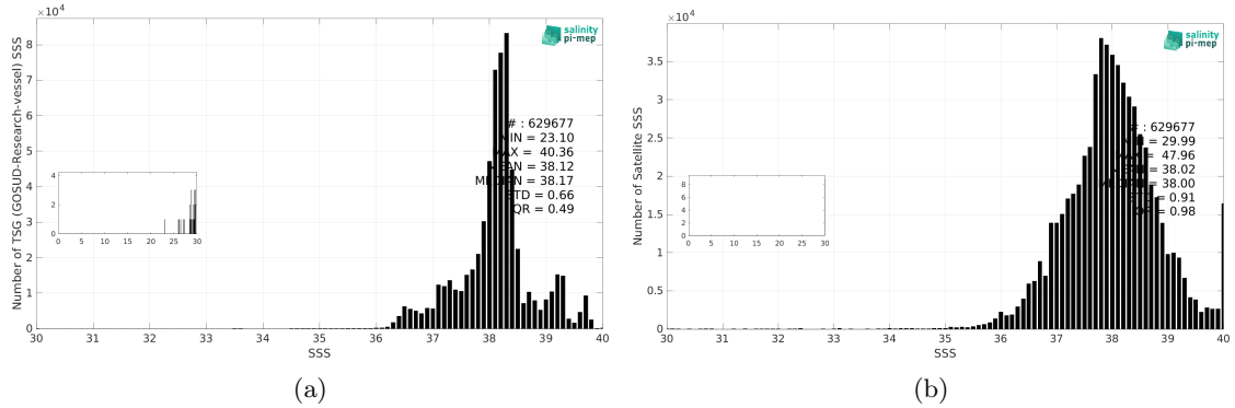
Figure 3: Histograms of SSS from TSG (GOSUD-Research-vessel) (a) and SMOS SSS L4 v2 - Daily (BEC) (b) considering all match-up pairs per bins of 0.1 over the Mediterranean Sea Pi-MEP region and for the full satellite product period.
