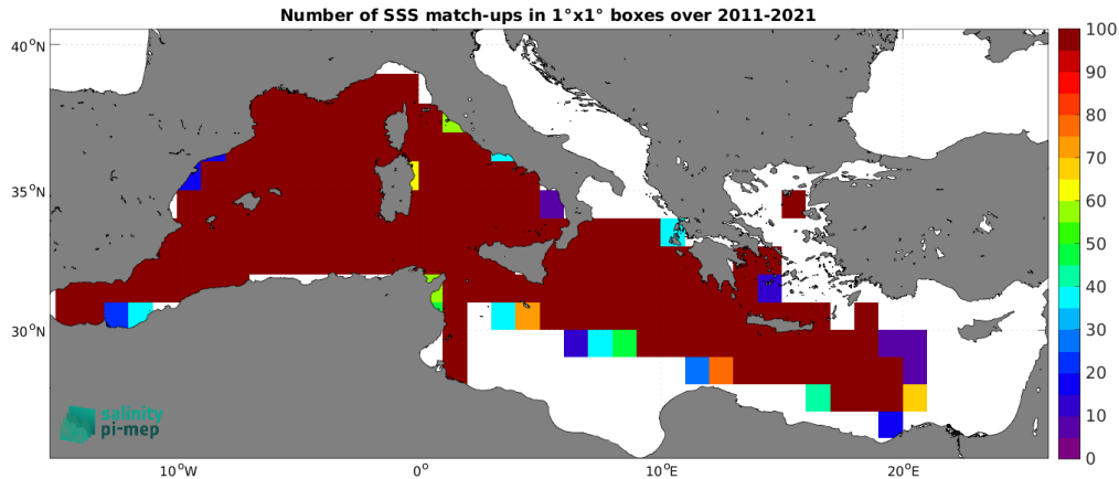
Figure 5: Number of SSS match-ups between TSG (GOSUD-Research-vessel) SSS and the SMOS SSS L4 v2 - Daily (BEC) SSS product for the Mediterranean Sea Pi-MEP region over 1^\circ \times 1^\circ boxes and for the full satellite product period.
