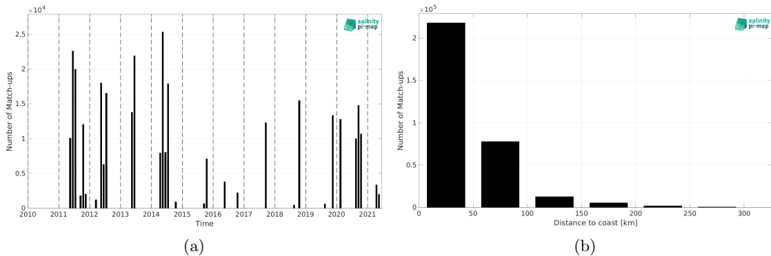
Figure 2: Number of match-ups between TSG (CSIC-UTM) and SMOS SSS L4 v2 - Daily (BEC) SSS as a function of time (a) and as function of the distance to coast (b) over the Mediterranean Sea Pi-MEP region and for the full satellite product period.
