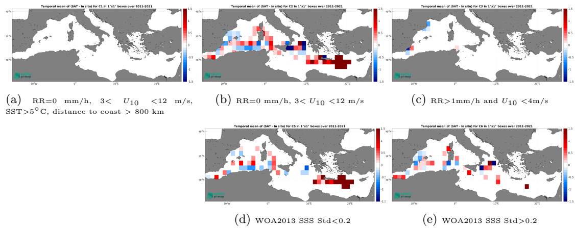
Figure 14: Temporal mean gridded over spatial boxes of size 1^\circ \times 1^\circ of \Delta\text{SSS} (SMOS SSS L4 v2 - Daily (BEC) - TSG (CSIC-UTM)) for 5 different subdatasets corresponding to:RR=0 mm/h, 3 < U_{10} < 12 m/s, SST>5°C, distance to coast > 800 km (a), RR=0 mm/h, 3 < U_{10} < 12 m/s (b), RR>1mm/h and U_{10} < 4 m/s (c), WOA2013 SSS Std<0.2 (d), WOA2013 SSS Std>0.2 (e).
