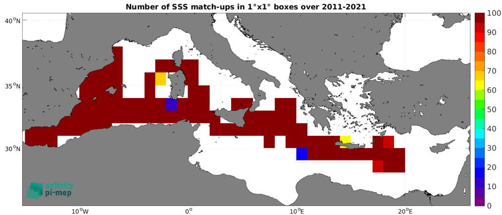
Figure 5: Number of SSS match-ups between TSG (CSIC-UTM) SSS and the SMOS SSS L4 v2 - Daily (BEC) SSS product for the Mediterranean Sea Pi-MEP region over 1^\circ \times 1^\circ boxes and for the full satellite product period.
