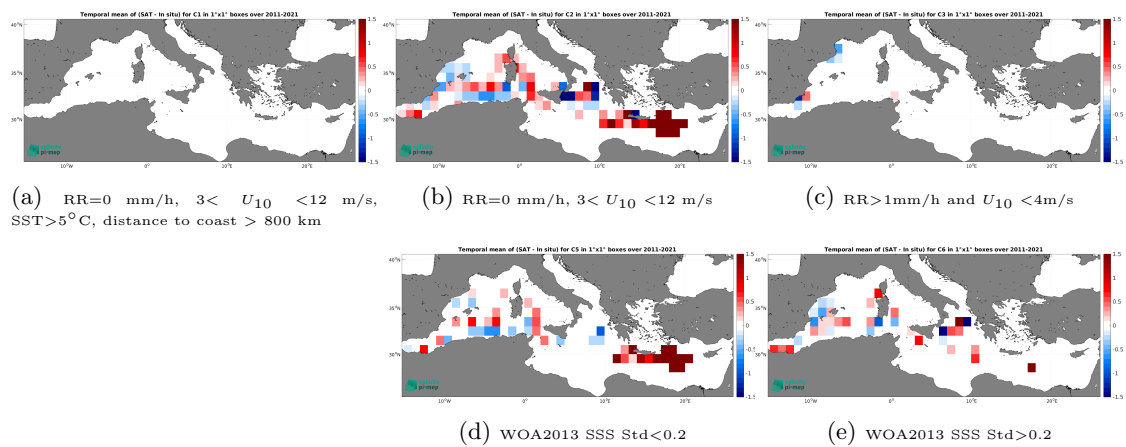
Figure 14: Temporal mean gridded over spatial boxes of size 1^\circ \times 1^\circ of \Delta SSS (SMOS SSS L4 v2 - Daily (BEC) - TSG (CSIC-UTM)) for 5 different subdatasets corresponding to:RR=0 mm/h, 3 < U_{10} < 12 m/s, SST >5^\circ\text{C} , distance to coast > 800 km (a), RR=0 mm/h, 3 < U_{10} < 12 m/s (b), RR >1 mm/h and U_{10} < 4 m/s (c), WOA2013 SSS Std <0.2 (d), WOA2013 SSS Std >0.2 (e).
