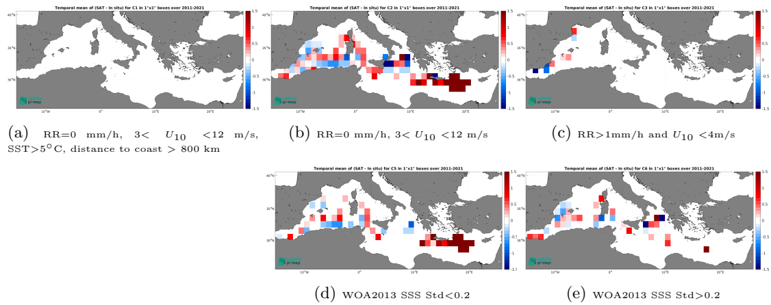
Figure 12: Temporal mean gridded over spatial boxes of size 1^\circ \times 1^\circ of \Delta\text{SSS} (SMOS SSS L4 v2 - Daily (BEC) - TSG (CSIC-UTM)) for 5 different subdatasets corresponding to:RR=0 mm/h, 3 < U_{10} < 12 m/s, SST >5^\circ\text{C} , distance to coast > 800 km (a), RR=0 mm/h, 3 < U_{10} < 12 m/s (b), RR >1 mm/h and U_{10} < 4 m/s (c), WOA2013 SSS Std <0.2 (d), WOA2013 SSS Std >0.2 (e).
