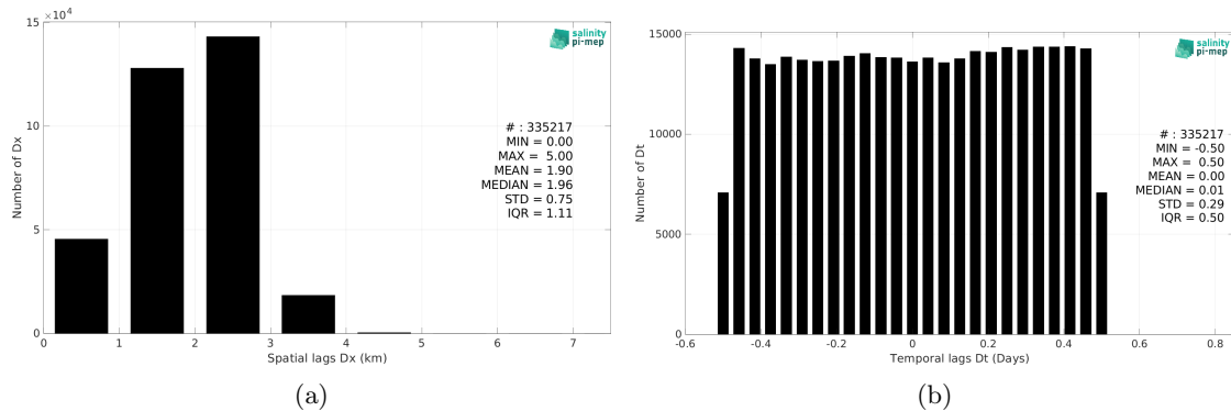
Figure 5: Histograms of the spatial (a) and temporal (b) lags between the location/time of the TSG (CSIC-UTM) measurement and the date of the corresponding SMOS SSS L4 v2 - Daily (BEC) SSS pixel.
