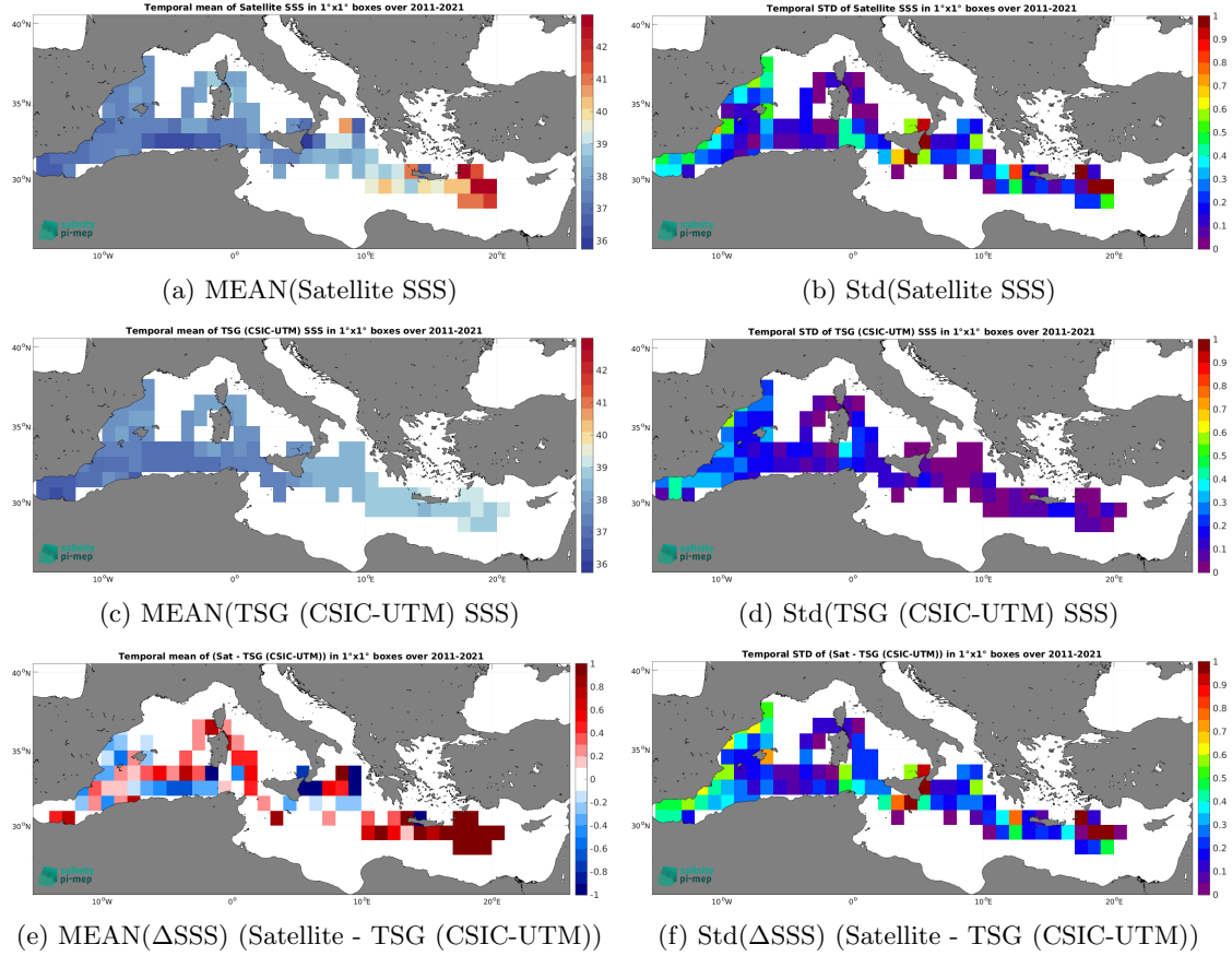
Figure 6: Temporal mean (left) and Std (right) of SSS from SMOS SSS L4 v2 - Daily (BEC) (top), TSG (CSIC-UTM) (middle), and of \Delta\text{SSS} (Satellite - TSG (CSIC-UTM)). Only match-up pairs are used to generate these maps.
