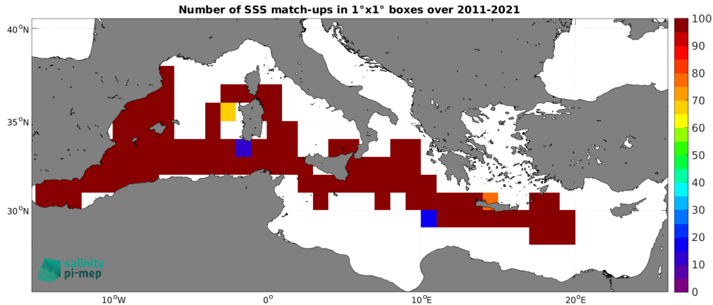
Figure 4: Number of SSS match-ups between TSG (CSIC-UTM) SSS and the SMOS SSS L4 v2 - Daily (BEC) SSS product for the Mediterranean Sea Pi-MEP region over 1^\circ \times 1^\circ boxes and for the full satellite product period.
