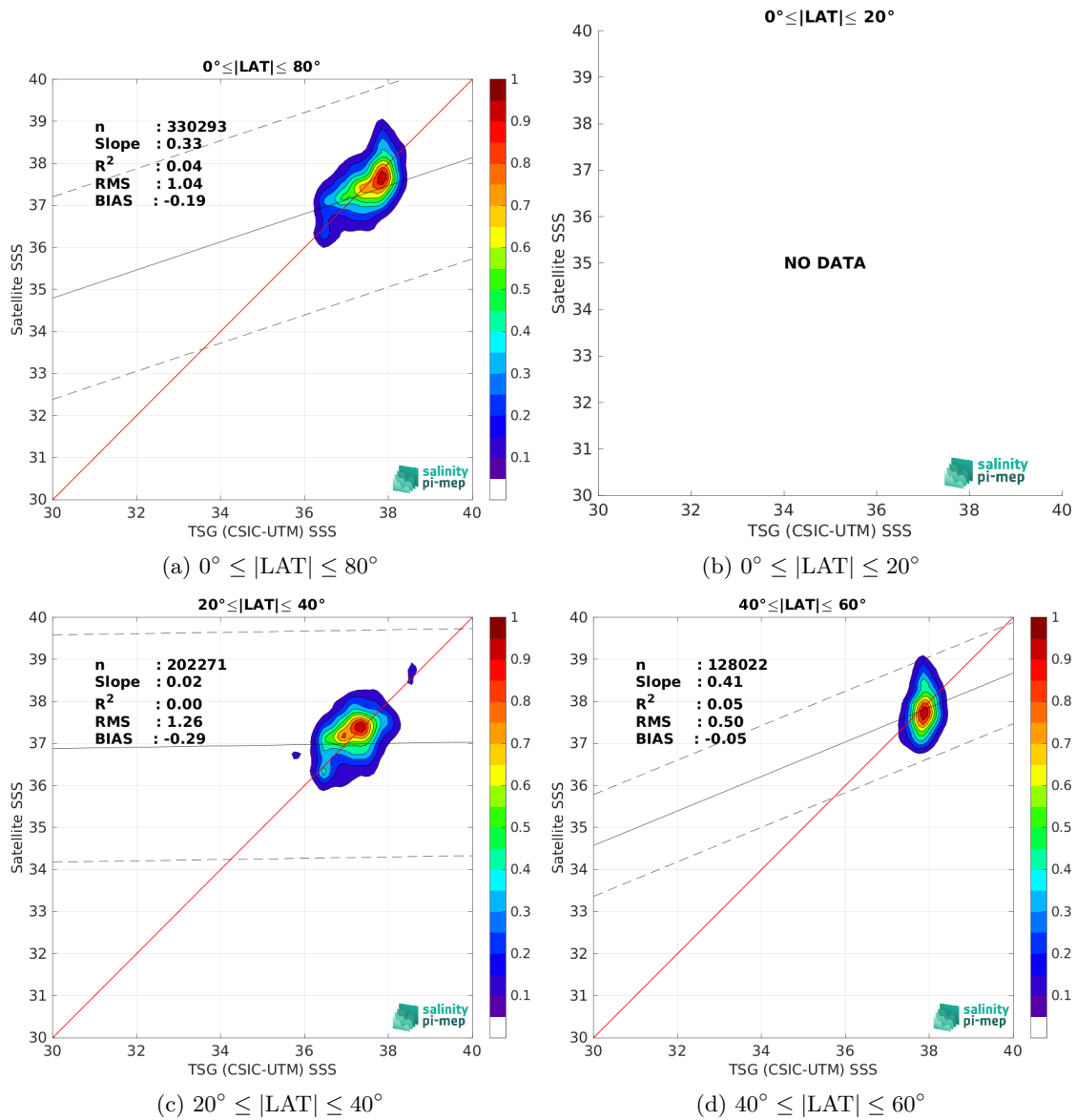
Figure 9: Contour maps of the concentration of SMOS SSS L4 v2 - Daily (BEC) SSS (y-axis) versus TSG (CSIC-UTM) SSS (x-axis) at match-up pairs for different latitude bands. For each plot, the red line shows x=y . The black thin and dashed lines indicate a linear fit through the data cloud and the \pm 95\% confidence levels, respectively. The number match-up pairs n , the slope and R^2 coefficient of the linear fit, the root mean square (RMS) and the mean bias between satellite and in situ data are indicated for each latitude band in each plots.
