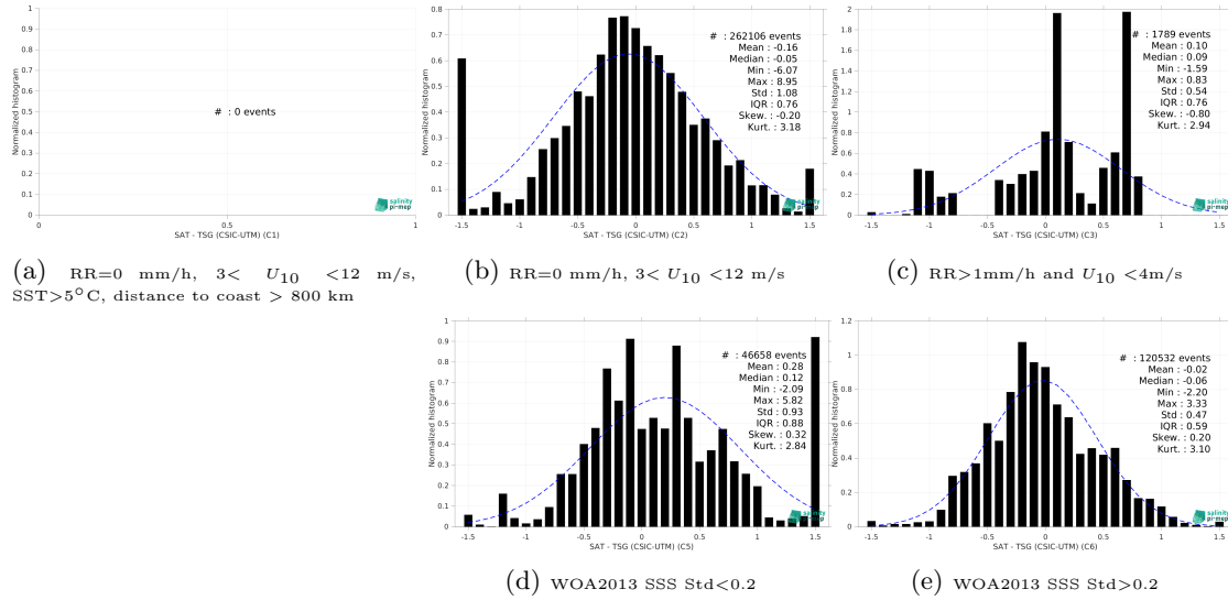
Figure 13: Normalized histogram of \Delta SSS (SMOS SSS L4 v2 - Daily (BEC) - TSG (CSIC-UTM)) for 5 different subdatasets corresponding to: RR=0 mm/h, 3 < U_{10} < 12 m/s, SST > 5°C, distance to coast > 800 km (a), RR=0 mm/h, 3 < U_{10} < 12 m/s (b), RR > 1mm/h and U_{10} < 4 m/s (c), WOA2013 SSS Std < 0.2 (d), WOA2013 SSS Std > 0.2 (e).
