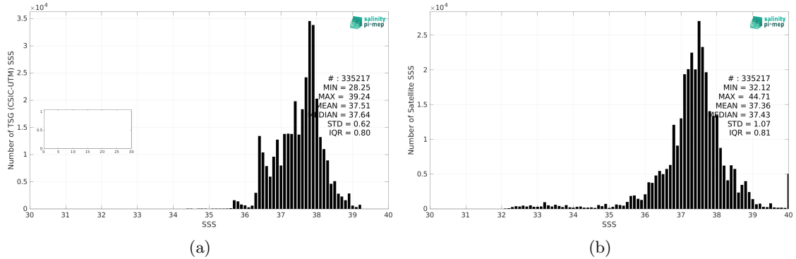
Figure 2: Histograms of SSS from TSG (CSIC-UTM) (a) and SMOS SSS L4 v2 - Daily (BEC) (b) considering all match-up pairs per bins of 0.1 over the Mediterranean Sea Pi-MEP region and for the full satellite product period.
