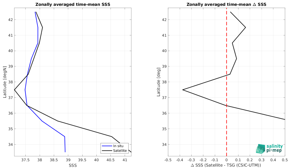
Figure 8: Left panel: Zonal mean SSS from SMOS SSS L4 v2 - Daily (BEC) satellite product (black) and from TSG (CSIC-UTM) (blue). Right panel: Zonal mean of \Delta SSS (Satellite - TSG (CSIC-UTM)) for all the collected Pi-MEP match-up pairs estimated over the full satellite product period.
