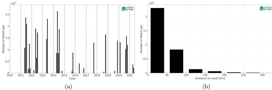
Figure 1: Number of match-ups between TSG (CSIC-UTM) and SMOS SSS L4 v2 - Daily (BEC) SSS as a function of time (a) and as function of the distance to coast (b) over the Mediterranean Sea Pi-MEP region and for the full satellite product period.
