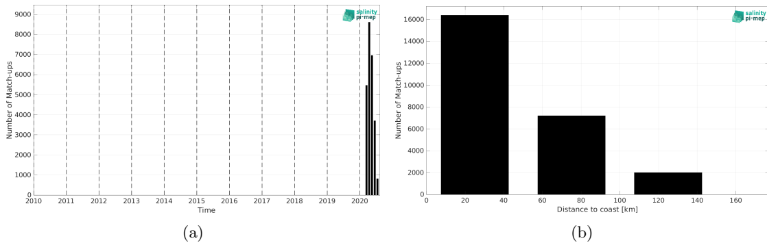
Figure 1: Number of match-ups between Saildrone and SMOS SSS L4 v2 - Daily (BEC) SSS as a function of time (a) and as function of the distance to coast (b) over the Mediterranean Sea Pi-MEP region and for the full satellite product period.
