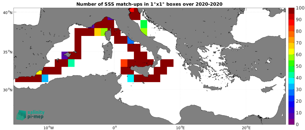
Figure 4: Number of SSS match-ups between Saildrone SSS and the SMOS SSS L4 v2 - Daily (BEC) SSS product for the Mediterranean Sea Pi-MEP region over 1^\circ \times 1^\circ boxes and for the full satellite product period.
