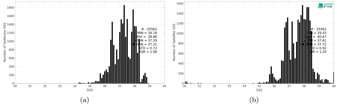
Figure 2: Histograms of SSS from Sairdrone (a) and SMOS SSS L4 v2 - Daily (BEC) (b) considering all match-up pairs per bins of 0.1 over the Mediterranean Sea Pi-MEP region and for the full satellite product period.
