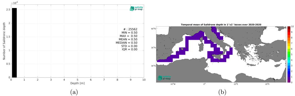
Figure 3: Histograms of the depth of the upper level SSS measurements from Sairdrone in the Match-up DataBase for the Mediterranean Sea Pi-MEP region (a) and temporal mean spatial distribution of pressure of the in situ SSS data over 1^\circ \times 1^\circ boxes and for the full satellite product period (b).
