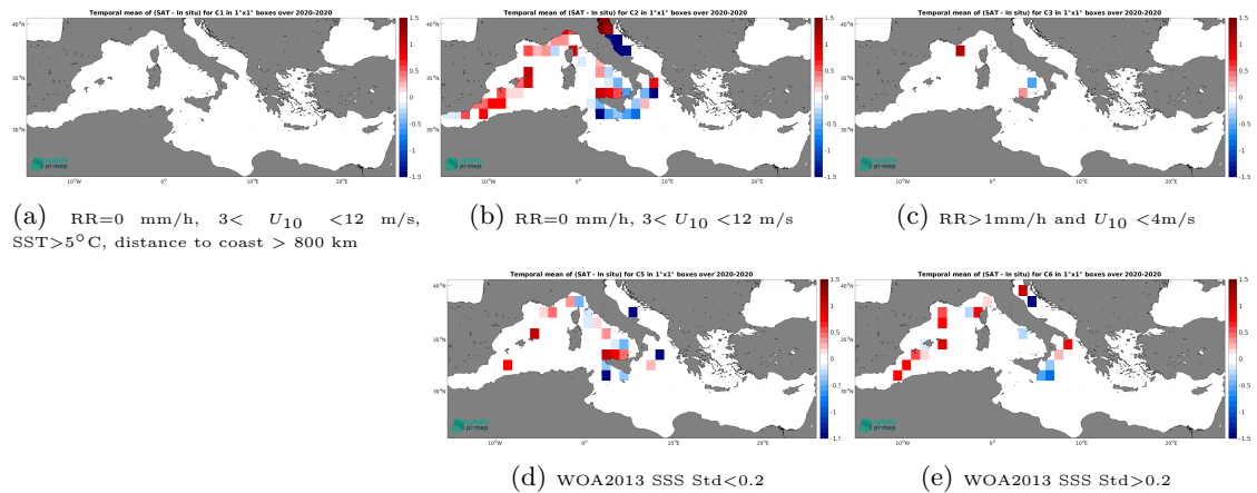
Figure 12: Temporal mean gridded over spatial boxes of size 1^\circ \times 1^\circ of \Delta SSS (SMOS SSS L4 v2 - Daily (BEC) - Saldrone) for 5 different subdatasets corresponding to:RR=0 mm/h, 3 < U_{10} < 12 m/s, SST >5^\circ\text{C} , distance to coast > 800 km (a), RR=0 mm/h, 3 < U_{10} < 12 m/s (b), RR >1 mm/h and U_{10} < 4 m/s (c), WOA2013 SSS Std <0.2 (d), WOA2013 SSS Std >0.2 (e).
