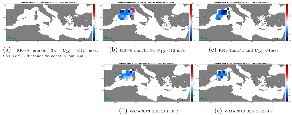
Figure 13: Temporal mean gridded over spatial boxes of size 1^\circ \times 1^\circ of \Delta SSS (SMOS SSS L4 v2 - Daily (BEC) - Surface drifters) for 5 different subdatasets corresponding to:RR=0 mm/h, 3 < U_{10} < 12 m/s, SST >5^\circ\text{C} , distance to coast > 800 km (a), RR=0 mm/h, 3 < U_{10} < 12 m/s (b), RR >1 mm/h and U_{10} < 4 m/s (c), WOA2013 SSS Std <0.2 (d), WOA2013 SSS Std >0.2 (e).
