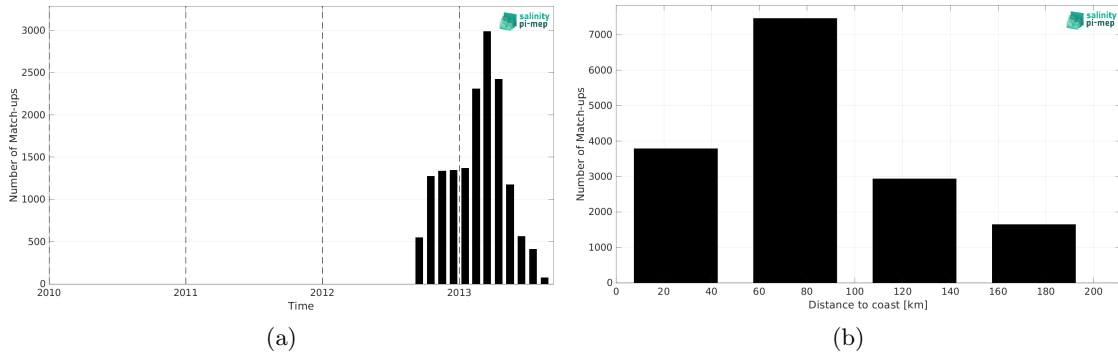
Figure 2: Number of match-ups between Surface drifters and SMOS SSS L4 v2 - Daily (BEC) SSS as a function of time (a) and as function of the distance to coast (b) over the Mediterranean Sea Pi-MEP region and for the full satellite product period.
