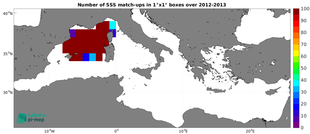
Figure 4: Number of SSS match-ups between Surface drifters SSS and the SMOS SSS L4 v2 - Daily (BEC) SSS product for the Mediterranean Sea Pi-MEP region over 1^\circ \times 1^\circ boxes and for the full satellite product period.
