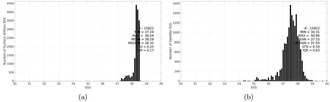
Figure 3: Histograms of SSS from Surface drifters (a) and SMOS SSS L4 v2 - Daily (BEC) (b) considering all match-up pairs per bins of 0.1 over the Mediterranean Sea Pi-MEP region and for the full satellite product period.
