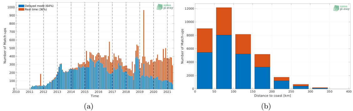
Figure 1: Number of match-ups between Argo and SMOS SSS L4 v2 - Daily (BEC) SSS as a function of time (a) and as function of the distance to coast (b) over the Mediterranean Sea Pi-MEP region and for the full satellite product period.
