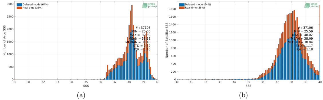
Figure 2: Histograms of SSS from Argo (a) and SMOS SSS L4 v2 - Daily (BEC) (b) considering all match-up pairs per bins of 0.1 over the Mediterranean Sea Pi-MEP region and for the full satellite product period.
