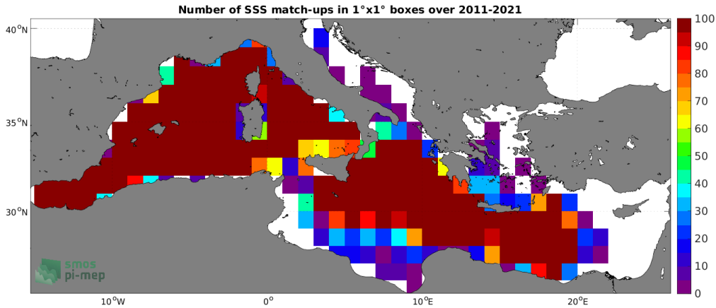
Figure 4: Number of SSS match-ups between Argo SSS and the SMOS SSS L4 v2 - Daily (BEC) SSS product for the Mediterranean Sea Pi-MEP region over 1^\circ \times 1^\circ boxes and for the full satellite product period.
