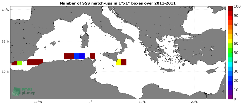
Figure 4: Number of SSS match-ups between TSG (SAMOS) SSS and the SMOS SSS L2Q v331 - With FLAG (CMEMS-CATDS-CPDC) SSS product for the Mediterranean Sea Pi-MEP region over 1^\circ \times 1^\circ boxes and for the full satellite product period.
