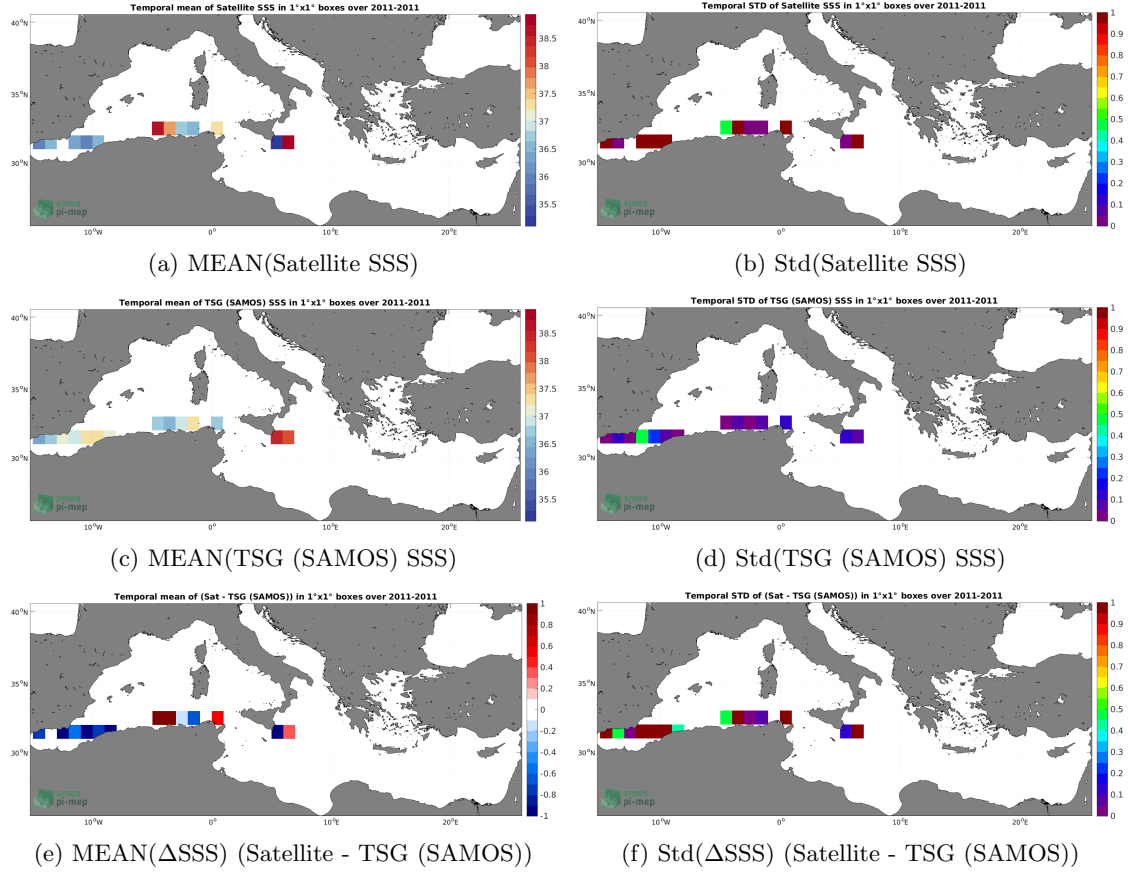
Figure 6: Temporal mean (left) and Std (right) of SSS from SMOS SSS L2Q v331 - With FLAG (CMEMS-CATDS-CPDC) (top), TSG (SAMOS) (middle), and of \Delta SSS (Satellite - TSG (SAMOS)). Only match-up pairs are used to generate these maps.
