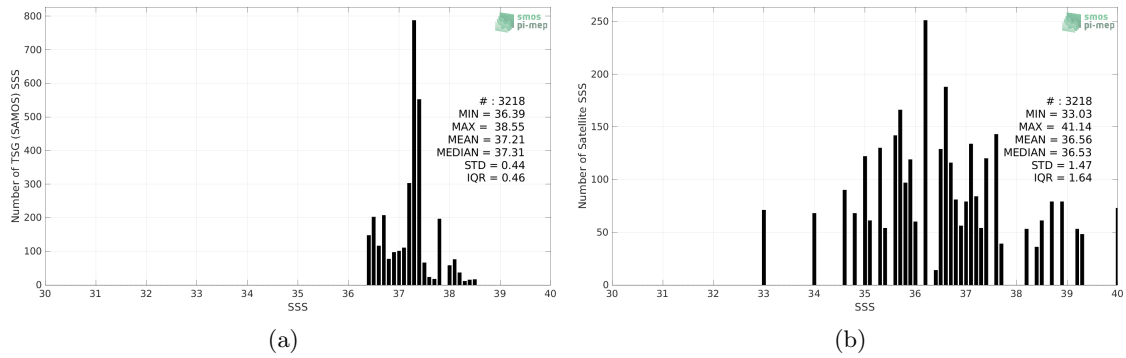
Figure 2: Histograms of SSS from TSG (SAMOS) (a) and SMOS SSS L2Q v331 - With FLAG (CMEMS-CATDS-CPDC) (b) considering all match-up pairs per bins of 0.1 over the Mediterranean Sea Pi-MEP region and for the full satellite product period.
