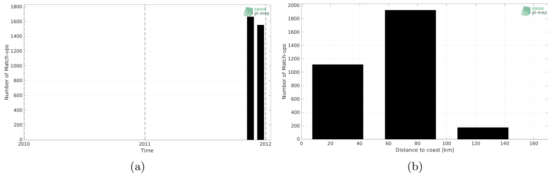
Figure 1: Number of match-ups between TSG (SAMOS) and SMOS SSS L2Q v331 - With FLAG (CMEMS-CATDS-CPDC) SSS as a function of time (a) and as function of the distance to coast (b) over the Mediterranean Sea Pi-MEP region and for the full satellite product period.
