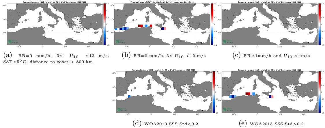
Figure 12: Temporal mean gridded over spatial boxes of size 1^{\circ}\times 1^{\circ} of \Delta\text{SSS} (SMOS SSS L2Q v331 - With FLAG (CMEMS-CATDS-CPDC) - TSG (SAMOS)) for 5 different subdatasets corresponding to:RR=0 mm/h, 3 < U_{10} < 12 m/s, SST >5^{\circ}\text{C} , distance to coast > 800 km (a), RR=0 mm/h, 3 < U_{10} < 12 m/s (b), RR >1 mm/h and U_{10} < 4 m/s (c), WOA2013 SSS Std <0.2 (d), WOA2013 SSS Std >0.2 (e).
