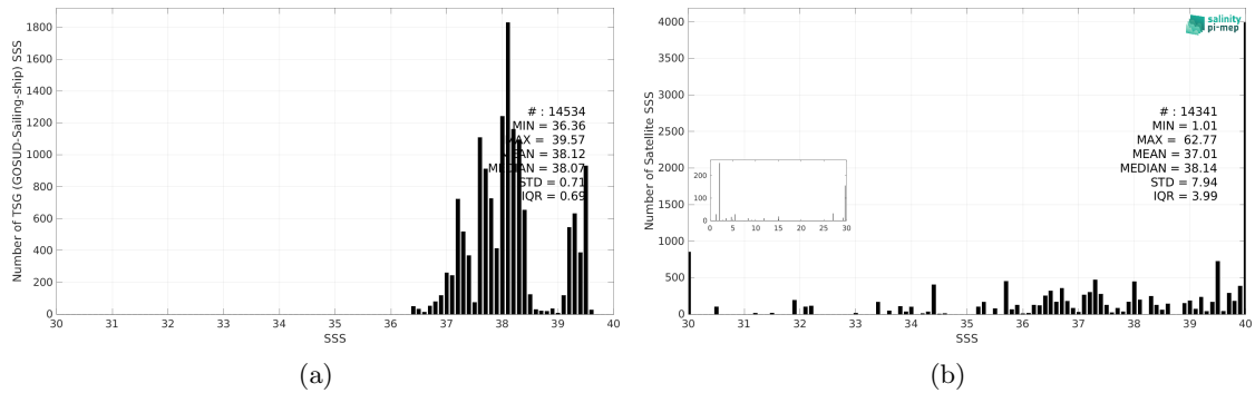
Figure 3: Histograms of SSS from TSG (GOSUD-Sailing-ship) (a) and SMOS SSS L2Q v331 - With FLAG (CMEMS-CATDS-CPDC) (b) considering all match-up pairs per bins of 0.1 over the Mediterranean Sea Pi-MEP region and for the full satellite product period.
