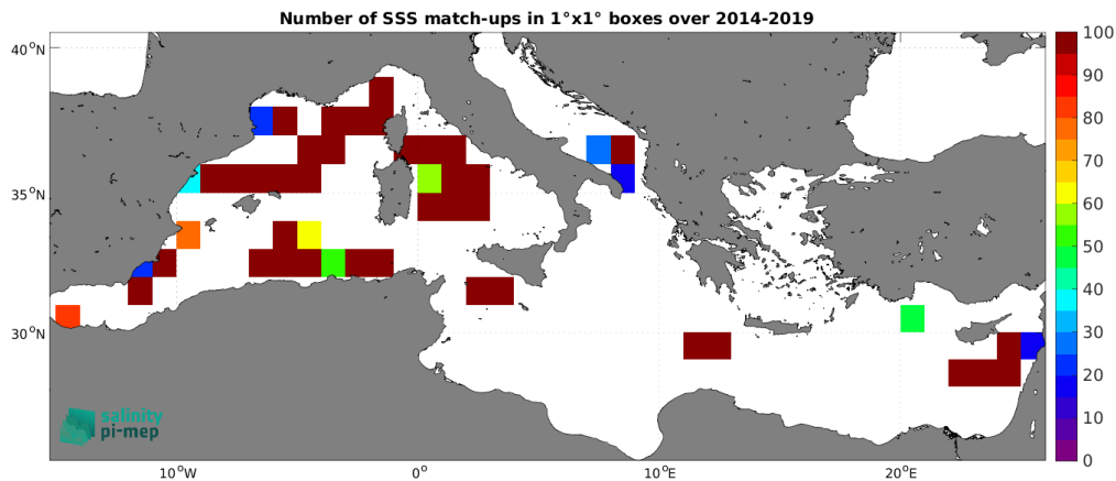
Figure 5: Number of SSS match-ups between TSG (GOSUD-Sailing-ship) SSS and the SMOS SSS L2Q v331 - With FLAG (CMEMS-CATDS-CPDC) SSS product for the Mediterranean Sea Pi-MEP region over 1^\circ \times 1^\circ boxes and for the full satellite product period.
