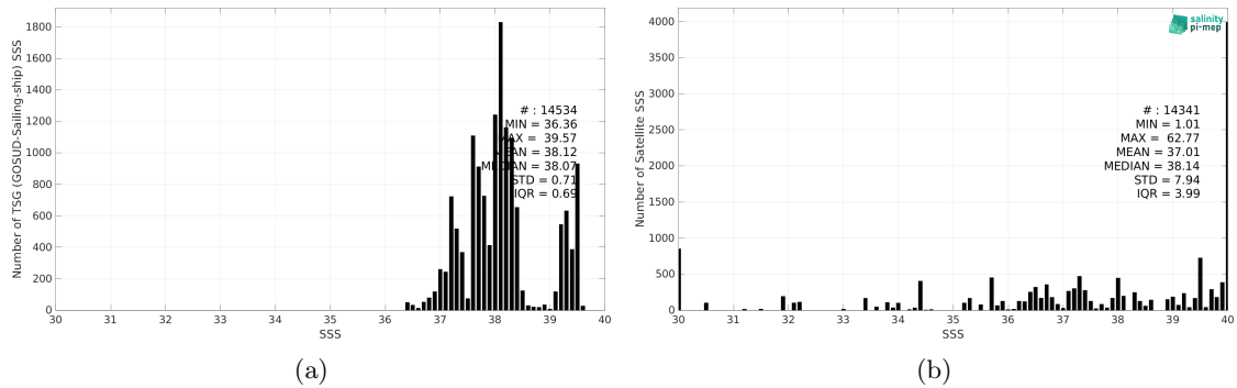
Figure 2: Histograms of SSS from TSG (GOSUD-Sailing-ship) (a) and SMOS SSS L2Q v331 - With FLAG (CMEMS-CATDS-CPDC) (b) considering all match-up pairs per bins of 0.1 over the Mediterranean Sea Pi-MEP region and for the full satellite product period.
