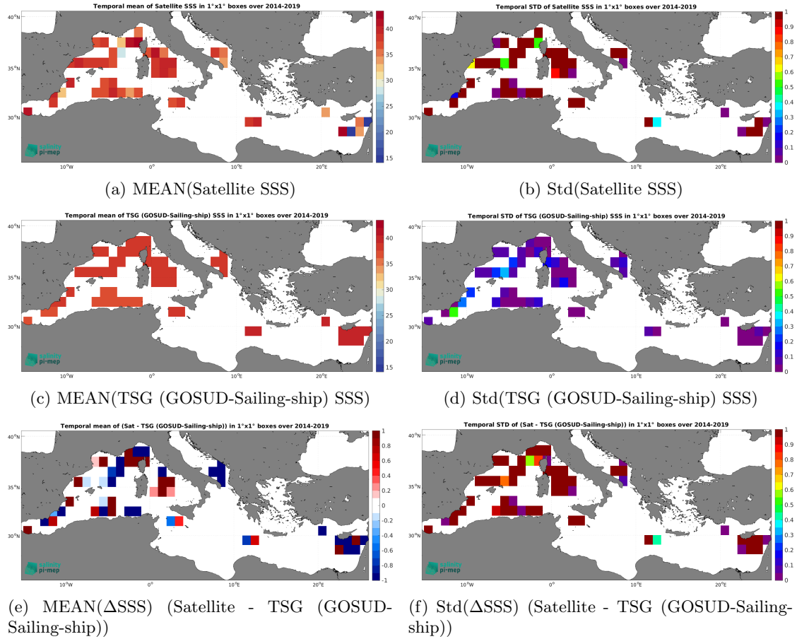
Figure 6: Temporal mean (left) and Std (right) of SSS from SMOS SSS L2Q v331 - With FLAG (CMEMS-CATDS-CPDC) (top), TSG (GOSUD-Sailing-ship) (middle), and of \Delta\text{SSS} (Satellite - TSG (GOSUD-Sailing-ship)). Only match-up pairs are used to generate these maps.
