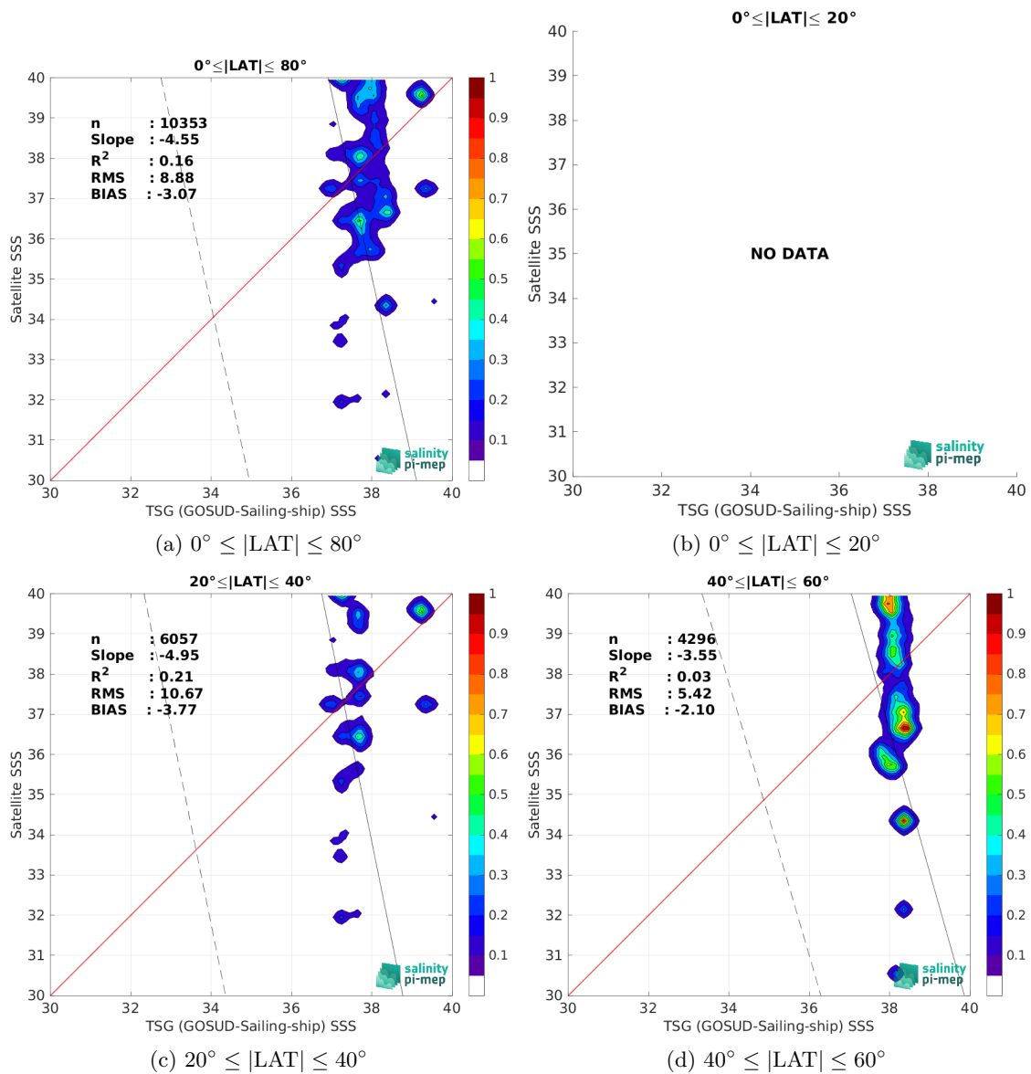
Figure 9: Contour maps of the concentration of SMOS SSS L2Q v331 - With FLAG (CMEMS-CATDS-CPDC) SSS (y-axis) versus TSG (GOSUD-Sailing-ship) SSS (x-axis) at match-up pairs for different latitude bands. For each plot, the red line shows x=y . The black thin and dashed lines indicate a linear fit through the data cloud and the \pm 95\% confidence levels, respectively. The number match-up pairs n , the slope and R^2 coefficient of the linear fit, the root mean square (RMS) and the mean bias between satellite and in situ data are indicated for each latitude band in each plots.
