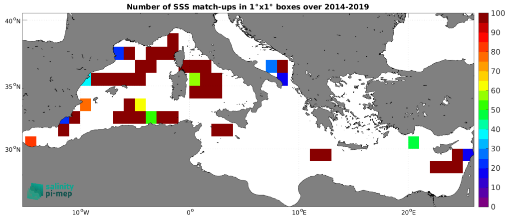
Figure 4: Number of SSS match-ups between TSG (GOSUD-Sailing-ship) SSS and the SMOS SSS L2Q v331 - With FLAG (CMEMS-CATDS-CPDC) SSS product for the Mediterranean Sea Pi-MEP region over 1^\circ \times 1^\circ boxes and for the full satellite product period.
