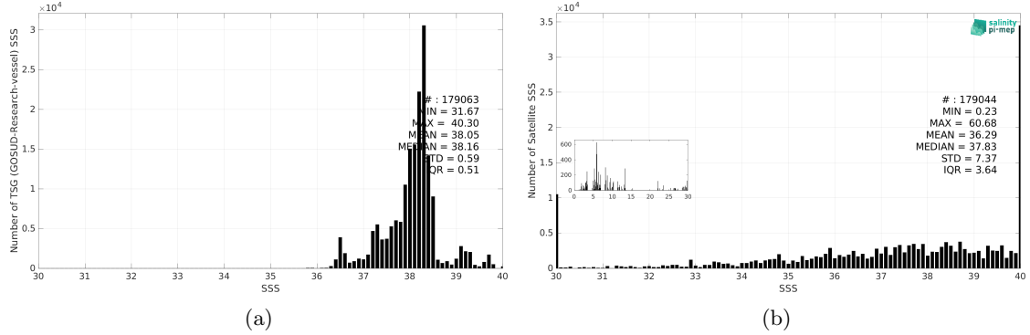
Figure 3: Histograms of SSS from TSG (GOSUD-Research-vessel) (a) and SMOS SSS L2Q v331 - With FLAG (CMEMS-CATDS-CPDC) (b) considering all match-up pairs per bins of 0.1 over the Mediterranean Sea Pi-MEP region and for the full satellite product period.
