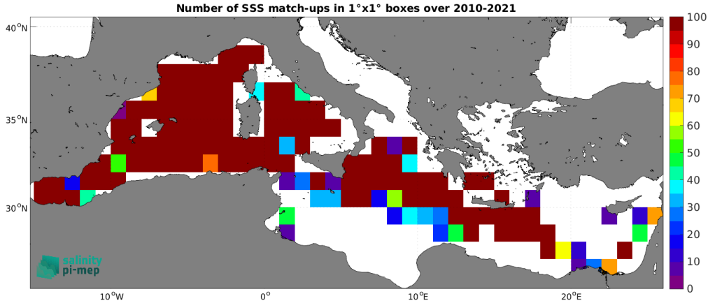
Figure 5: Number of SSS match-ups between TSG (GOSUD-Research-vessel) SSS and the SMOS SSS L2Q v331 - With FLAG (CMEMS-CATDS-CPDC) SSS product for the Mediterranean Sea Pi-MEP region over 1^\circ \times 1^\circ boxes and for the full satellite product period.
