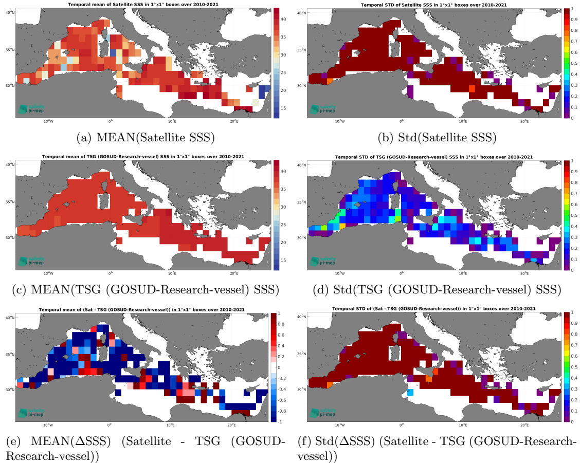
Figure 7: Temporal mean (left) and Std (right) of SSS from SMOS SSS L2Q v331 - With FLAG (CMEMS-CATDS-CPDC) (top), TSG (GOSUD-Research-vessel) (middle), and of \Delta\text{SSS} (Satellite - TSG (GOSUD-Research-vessel)). Only match-up pairs are used to generate these maps.
