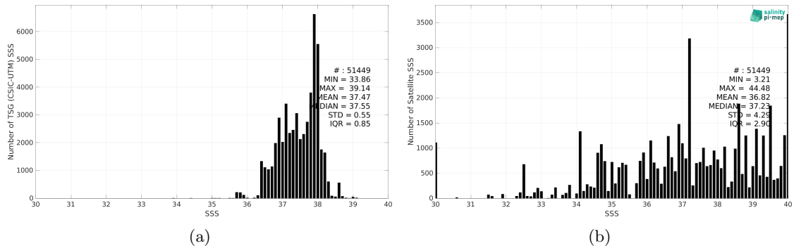
Figure 2: Histograms of SSS from TSG (CSIC-UTM) (a) and SMOS SSS L2Q v331 - With FLAG (CMEMS-CATDS-CPDC) (b) considering all match-up pairs per bins of 0.1 over the Mediterranean Sea Pi-MEP region and for the full satellite product period.
