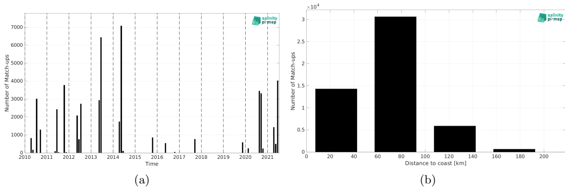
Figure 1: Number of match-ups between TSG (CSIC-UTM) and SMOS SSS L2Q v331 - With FLAG (CMEMS-CATDS-CPDC) SSS as a function of time (a) and as function of the distance to coast (b) over the Mediterranean Sea Pi-MEP region and for the full satellite product period.
