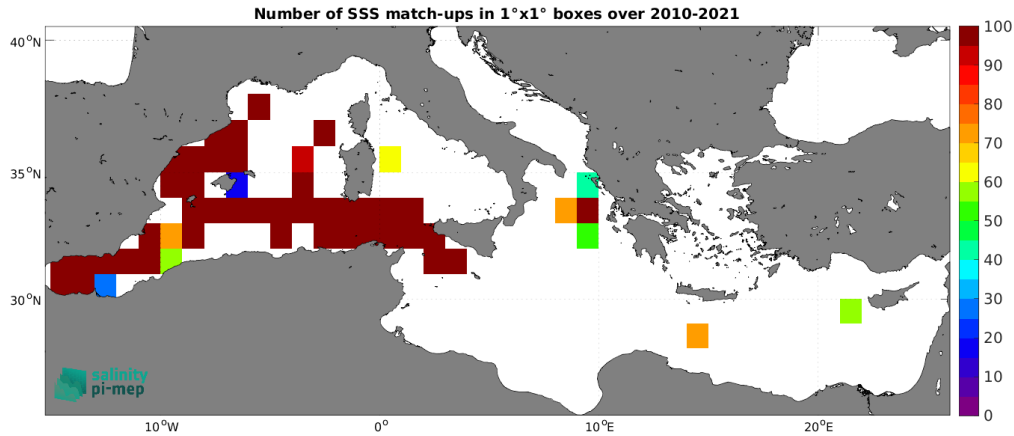
Figure 4: Number of SSS match-ups between TSG (CSIC-UTM) SSS and the SMOS SSS L2Q v331 - With FLAG (CMEMS-CATDS-CPDC) SSS product for the Mediterranean Sea Pi-MEP region over 1^\circ \times 1^\circ boxes and for the full satellite product period.
