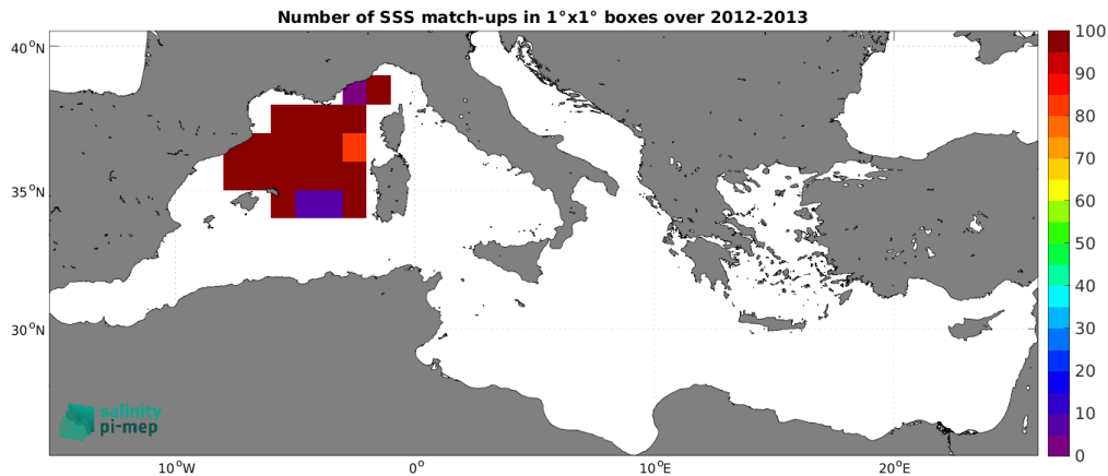
Figure 4: Number of SSS match-ups between Surface drifters SSS and the SMOS SSS L2Q v331 - With FLAG (CMEMS-CATDS-CPDC) SSS product for the Mediterranean Sea Pi-MEP region over 1^\circ \times 1^\circ boxes and for the full satellite product period.
