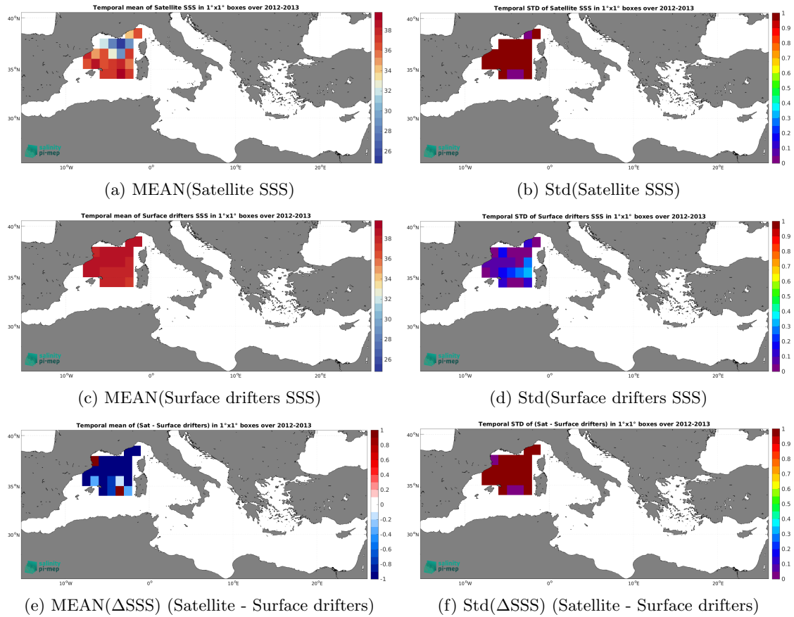
Figure 6: Temporal mean (left) and Std (right) of SSS from SMOS SSS L2Q v331 - With FLAG (CMEMS-CATDS-CPDC) (top), Surface drifters (middle), and of \Delta SSS (Satellite - Surface drifters). Only match-up pairs are used to generate these maps.
