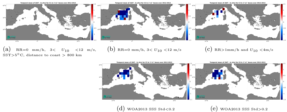
Figure 13: Temporal mean gridded over spatial boxes of size 1^\circ \times 1^\circ of \Delta SSS (SMOS SSS L2Q v331 - With FLAG (CMEMS-CATDS-CPDC) - Surface drifters) for 5 different subdatasets corresponding to:RR=0 mm/h, 3 < U_{10} < 12 m/s, SST >5^\circ\text{C} , distance to coast > 800 km (a), RR=0 mm/h, 3 < U_{10} < 12 m/s (b), RR >1 mm/h and U_{10} < 4 m/s (c), WOA2013 SSS Std <0.2 (d), WOA2013 SSS Std >0.2 (e).
