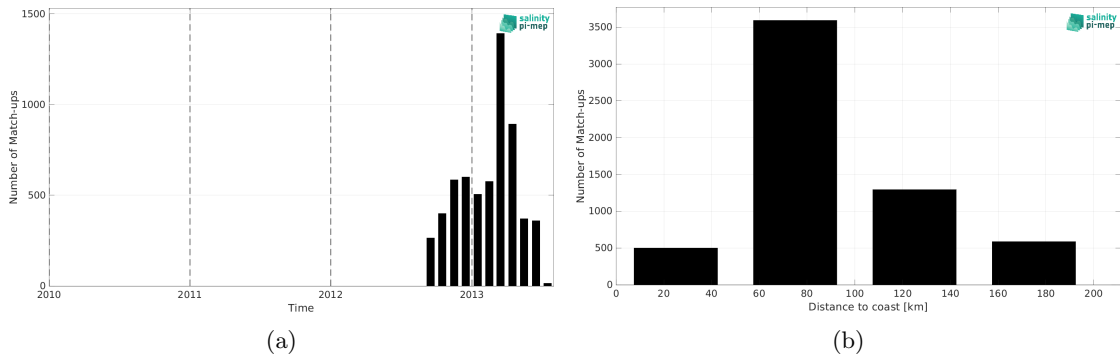
Figure 2: Number of match-ups between Surface drifters and SMOS SSS L2Q v331 - With FLAG (CMEMS-CATDS-CPDC) SSS as a function of time (a) and as function of the distance to coast (b) over the Mediterranean Sea Pi-MEP region and for the full satellite product period.
