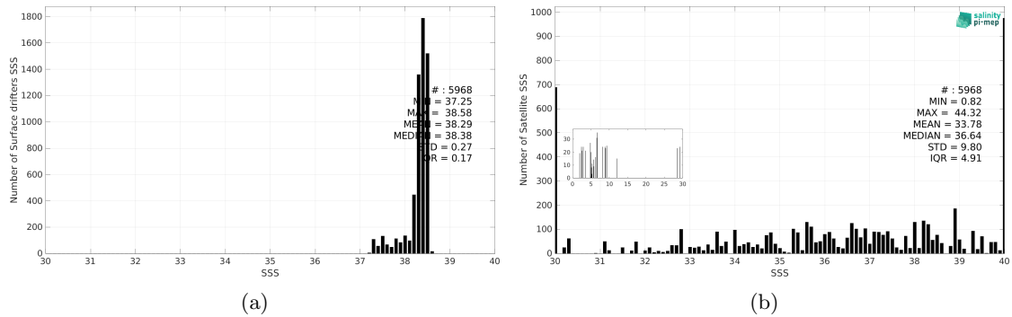
Figure 3: Histograms of SSS from Surface drifters (a) and SMOS SSS L2Q v331 - With FLAG (CMEMS-CATDS-CPDC) (b) considering all match-up pairs per bins of 0.1 over the Mediterranean Sea Pi-MEP region and for the full satellite product period.
