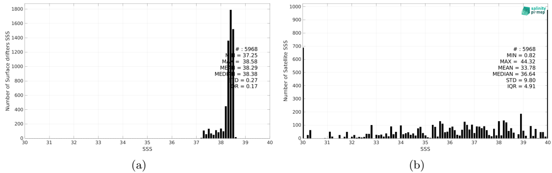
Figure 2: Histograms of SSS from Surface drifters (a) and SMOS SSS L2Q v331 - With FLAG (CMEMS-CATDS-CPDC) (b) considering all match-up pairs per bins of 0.1 over the Mediterranean Sea Pi-MEP region and for the full satellite product period.
