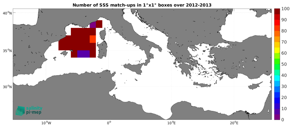
Figure 3: Number of SSS match-ups between Surface drifters SSS and the SMOS SSS L2Q v331 - With FLAG (CMEMS-CATDS-CPDC) SSS product for the Mediterranean Sea Pi-MEP region over 1^\circ \times 1^\circ boxes and for the full satellite product period.
