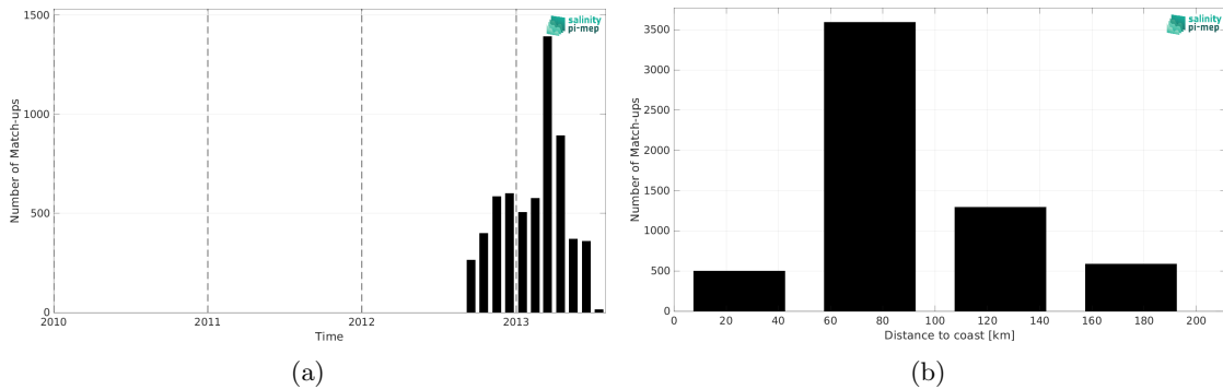
Figure 1: Number of match-ups between Surface drifters and SMOS SSS L2Q v331 - With FLAG (CMEMS-CATDS-CPDC) SSS as a function of time (a) and as function of the distance to coast (b) over the Mediterranean Sea Pi-MEP region and for the full satellite product period.
