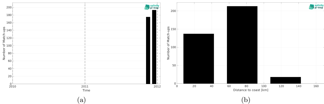
Figure 2: Number of match-ups between TSG (SAMOS) and SMOS SSS L2Q v331 - No FLAG (CMEMS-CATDS-CPDC) SSS as a function of time (a) and as function of the distance to coast (b) over the Mediterranean Sea Pi-MEP region and for the full satellite product period.
