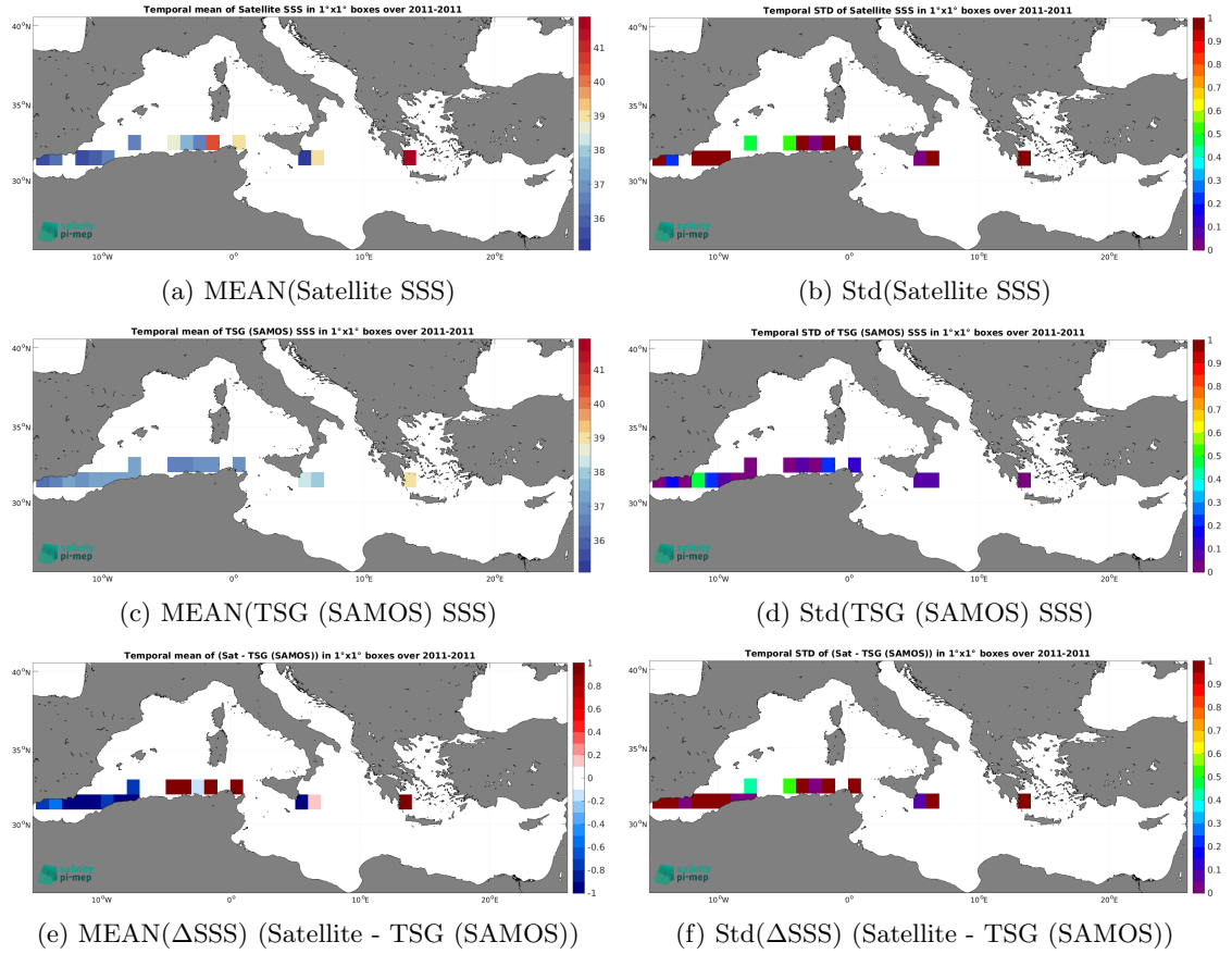
Figure 7: Temporal mean (left) and Std (right) of SSS from SMOS SSS L2Q v331 - No FLAG (CMEMS-CATDS-CPDC) (top), TSG (SAMOS) (middle), and of \Delta\text{SSS} (Satellite - TSG (SAMOS)). Only match-up pairs are used to generate these maps.
