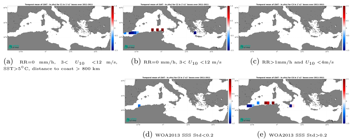
Figure 14: Temporal mean gridded over spatial boxes of size 1^\circ \times 1^\circ of \Delta\text{SSS} (SMOS SSS L2Q v331 - No FLAG (CMEMS-CATDS-CPDC) - TSG (SAMOS)) for 5 different subdatasets corresponding to:RR=0 mm/h, 3 < U_{10} < 12 m/s, SST>5°C, distance to coast > 800 km (a), RR=0 mm/h, 3 < U_{10} < 12 m/s (b), RR>1mm/h and U_{10} < 4 m/s (c), WOA2013 SSS Std<0.2 (d), WOA2013 SSS Std>0.2 (e).
