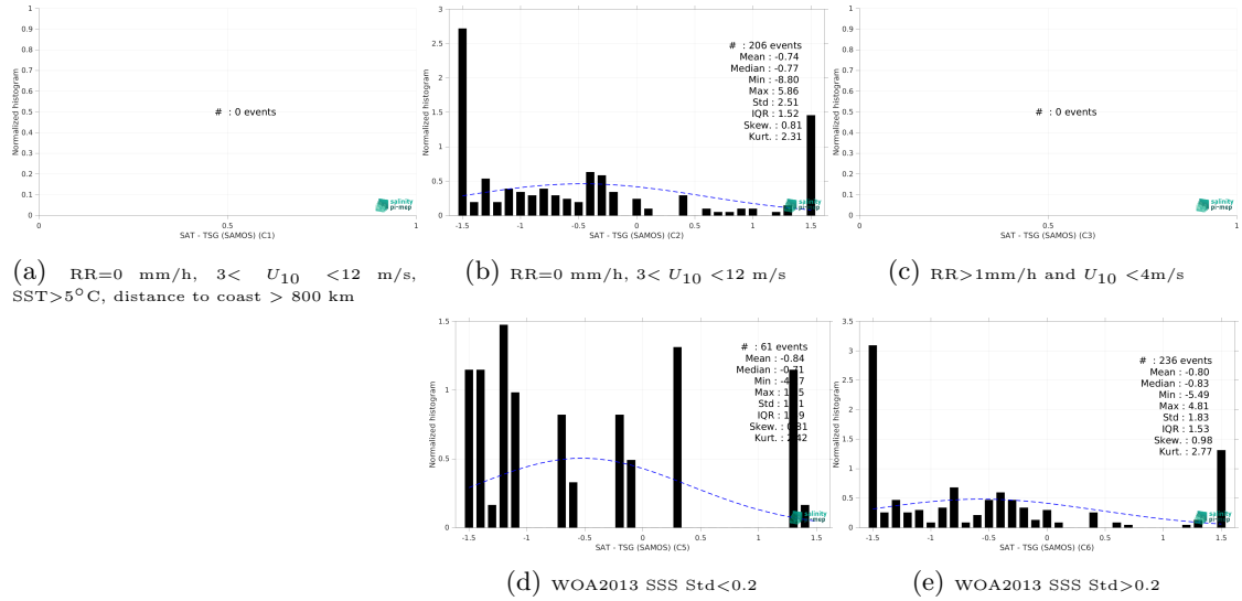
Figure 15: Normalized histogram of \Delta SSS (SMOS SSS L2Q v331 - No FLAG (CMEMS-CATDS-CPDC) - TSG (SAMOS)) for 5 different subdatasets corresponding to: RR=0 mm/h, 3 < U_{10} < 12 m/s, SST > 5°C, distance to coast > 800 km (a), RR=0 mm/h, 3 < U_{10} < 12 m/s (b), RR > 1mm/h and U_{10} < 4 m/s (c), WOA2013 SSS Std < 0.2 (d), WOA2013 SSS Std > 0.2 (e).
