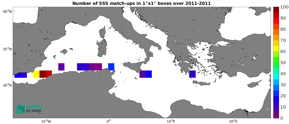
Figure 5: Number of SSS match-ups between TSG (SAMOS) SSS and the SMOS SSS L2Q v331 - No FLAG (CMEMS-CATDS-CPDC) SSS product for the Mediterranean Sea Pi-MEP region over 1^\circ \times 1^\circ boxes and for the full satellite product period.
