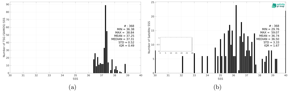
Figure 3: Histograms of SSS from TSG (SAMOS) (a) and SMOS SSS L2Q v331 - No FLAG (CMEMS-CATDS-CPDC) (b) considering all match-up pairs per bins of 0.1 over the Mediterranean Sea Pi-MEP region and for the full satellite product period.
