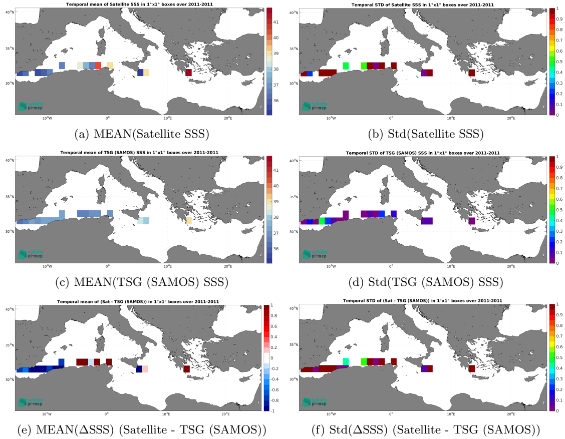
Figure 6: Temporal mean (left) and Std (right) of SSS from SMOS SSS L2Q v331 - No FLAG (CMEMS-CATDS-CPDC) (top), TSG (SAMOS) (middle), and of \Delta\text{SSS} (Satellite - TSG (SAMOS)). Only match-up pairs are used to generate these maps.
