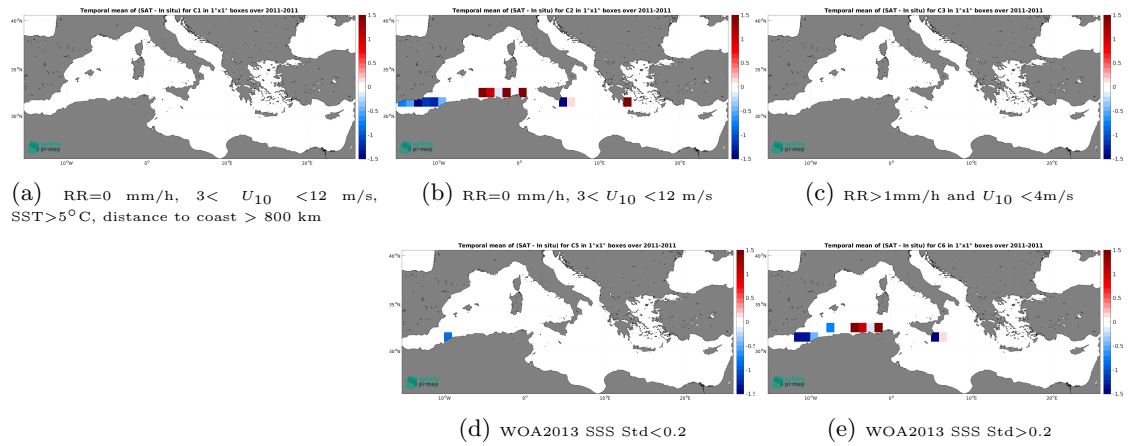
Figure 12: Temporal mean gridded over spatial boxes of size 1^{\circ}\times 1^{\circ} of \Delta\text{SSS} (SMOS SSS L2Q v331 - No FLAG (CMEMS-CATDS-CPDC) - TSG (SAMOS)) for 5 different subdatasets corresponding to:RR=0 mm/h, 3 < U_{10} < 12 m/s, SST > 5^{\circ}\text{C} , distance to coast > 800 km (a), RR=0 mm/h, 3 < U_{10} < 12 m/s (b), RR > 1 mm/h and U_{10} < 4 m/s (c), WOA2013 SSS Std < 0.2 (d), WOA2013 SSS Std > 0.2 (e).
