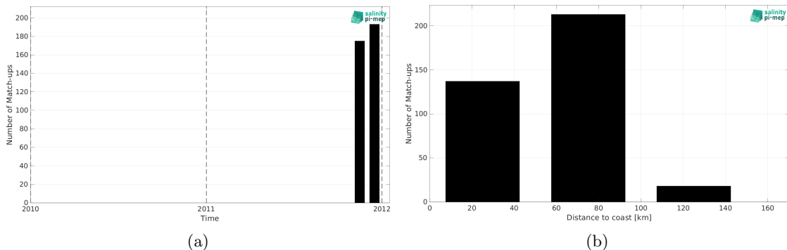
Figure 1: Number of match-ups between TSG (SAMOS) and SMOS SSS L2Q v331 - No FLAG (CMEMS-CATDS-CPDC) SSS as a function of time (a) and as function of the distance to coast (b) over the Mediterranean Sea Pi-MEP region and for the full satellite product period.
