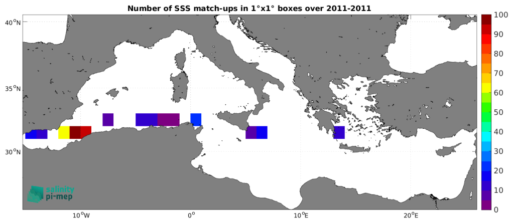
Figure 4: Number of SSS match-ups between TSG (SAMOS) SSS and the SMOS SSS L2Q v331 - No FLAG (CMEMS-CATDS-CPDC) SSS product for the Mediterranean Sea Pi-MEP region over 1^\circ \times 1^\circ boxes and for the full satellite product period.
