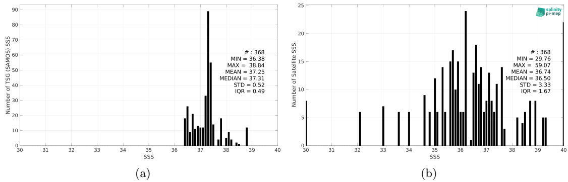
Figure 2: Histograms of SSS from TSG (SAMOS) (a) and SMOS SSS L2Q v331 - No FLAG (CMEMS-CATDS-CPDC) (b) considering all match-up pairs per bins of 0.1 over the Mediterranean Sea Pi-MEP region and for the full satellite product period.
