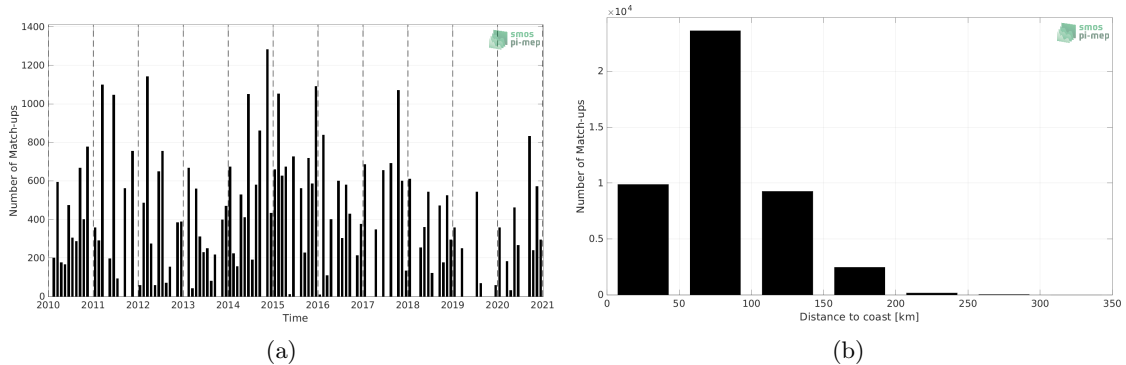
Figure 1: Number of match-ups between TSG (LEGOS-DM) and SMOS SSS L2Q v331 - No FLAG (CMEMS-CATDS-CPDC) SSS as a function of time (a) and as function of the distance to coast (b) over the Mediterranean Sea Pi-MEP region and for the full satellite product period.
