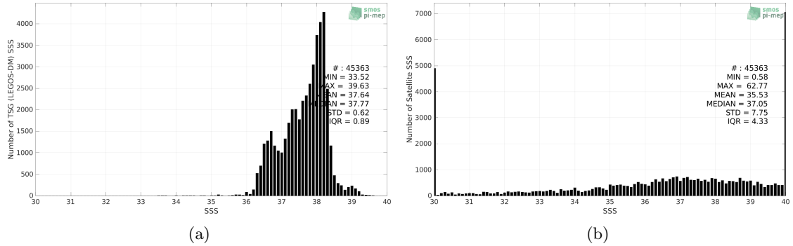
Figure 2: Histograms of SSS from TSG (LEGOS-DM) (a) and SMOS SSS L2Q v331 - No FLAG (CMEMS-CATDS-CPDC) (b) considering all match-up pairs per bins of 0.1 over the Mediterranean Sea Pi-MEP region and for the full satellite product period.
