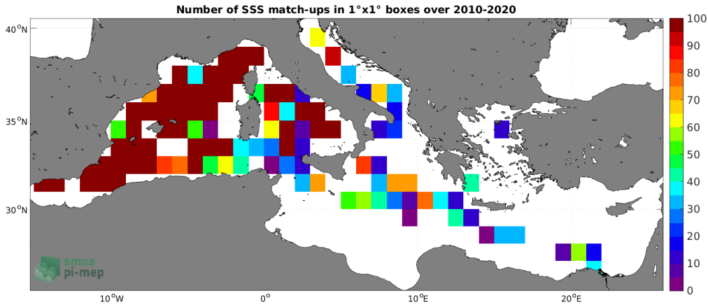
Figure 4: Number of SSS match-ups between TSG (LEGOS-DM) SSS and the SMOS SSS L2Q v331 - No FLAG (CMEMS-CATDS-CPDC) SSS product for the Mediterranean Sea Pi-MEP region over 1^\circ \times 1^\circ boxes and for the full satellite product period.
