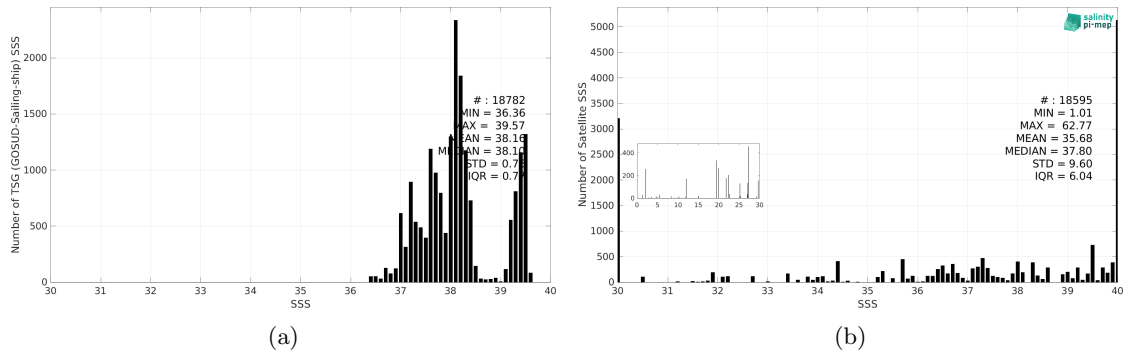
Figure 3: Histograms of SSS from TSG (GOSUD-Sailing-ship) (a) and SMOS SSS L2Q v331 - No FLAG (CMEMS-CATDS-CPDC) (b) considering all match-up pairs per bins of 0.1 over the Mediterranean Sea Pi-MEP region and for the full satellite product period.
