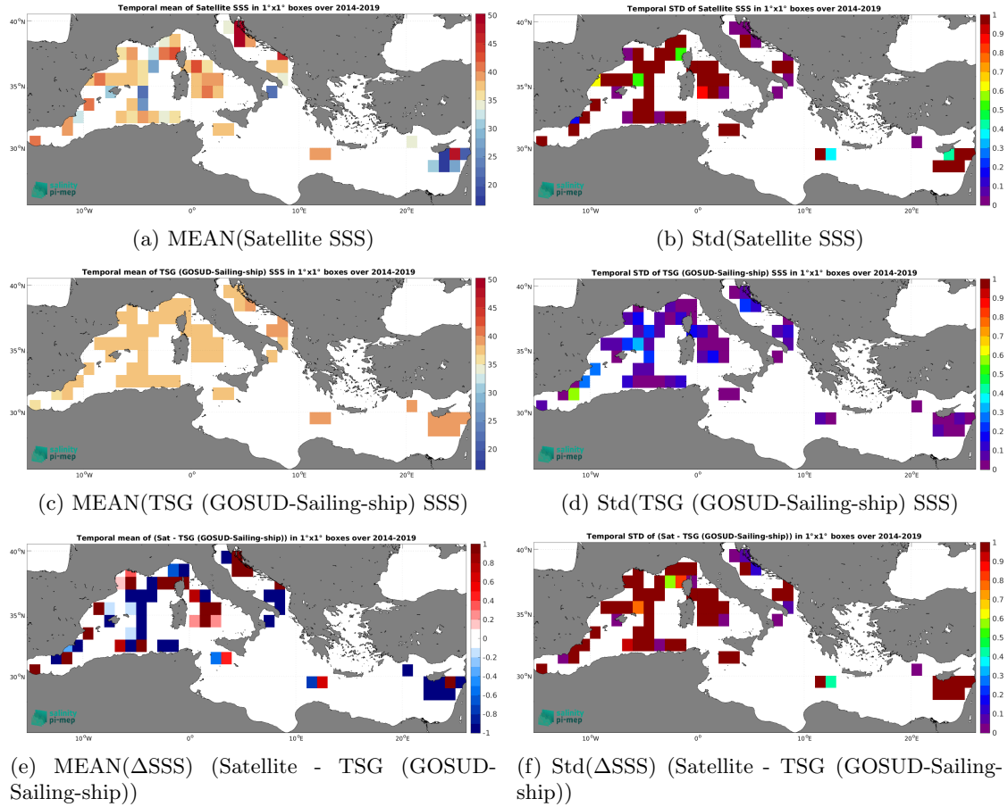
Figure 7: Temporal mean (left) and Std (right) of SSS from SMOS SSS L2Q v331 - No FLAG (CMEMS-CATDS-CPDC) (top), TSG (GOSUD-Sailing-ship) (middle), and of \Delta\text{SSS} (Satellite - TSG (GOSUD-Sailing-ship)). Only match-up pairs are used to generate these maps.
