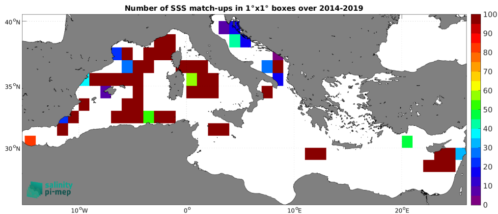
Figure 5: Number of SSS match-ups between TSG (GOSUD-Sailing-ship) SSS and the SMOS SSS L2Q v331 - No FLAG (CMEMS-CATDS-CPDC) SSS product for the Mediterranean Sea Pi-MEP region over 1^\circ \times 1^\circ boxes and for the full satellite product period.
