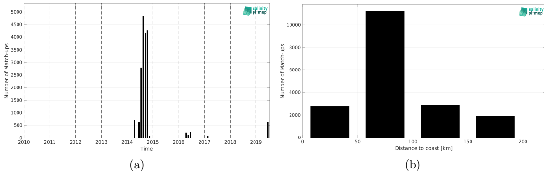
Figure 2: Number of match-ups between TSG (GOSUD-Sailing-ship) and SMOS SSS L2Q v331 - No FLAG (CMEMS-CATDS-CPDC) SSS as a function of time (a) and as function of the distance to coast (b) over the Mediterranean Sea Pi-MEP region and for the full satellite product period.
