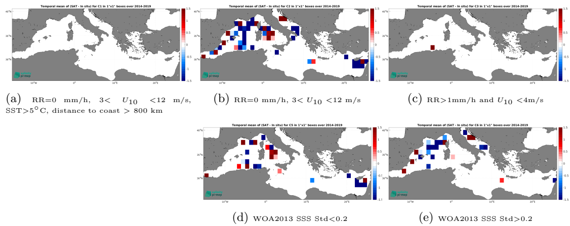
Figure 14: Temporal mean gridded over spatial boxes of size 1^\circ \times 1^\circ of \Delta\text{SSS} (SMOS SSS L2Q v331 - No FLAG (CMEMS-CATDS-CPDC) - TSG (GOSUD-Sailing-ship)) for 5 different sub-datasets corresponding to:RR=0 mm/h, 3 < U_{10} < 12 m/s, SST>5°C, distance to coast > 800 km (a), RR=0 mm/h, 3 < U_{10} < 12 m/s (b), RR>1mm/h and U_{10} < 4 m/s (c), WOA2013 SSS Std<0.2 (d), WOA2013 SSS Std>0.2 (e).
