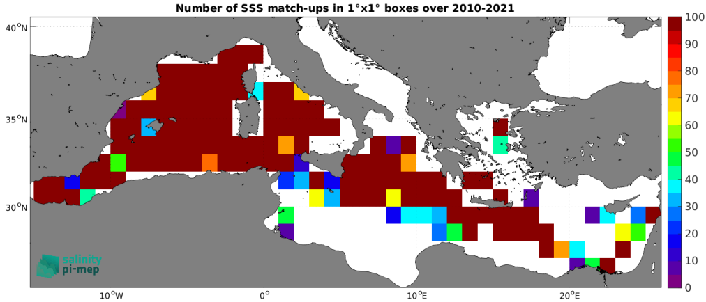
Figure 5: Number of SSS match-ups between TSG (GOSUD-Research-vessel) SSS and the SMOS SSS L2Q v331 - No FLAG (CMEMS-CATDS-CPDC) SSS product for the Mediterranean Sea Pi-MEP region over 1^\circ \times 1^\circ boxes and for the full satellite product period.
