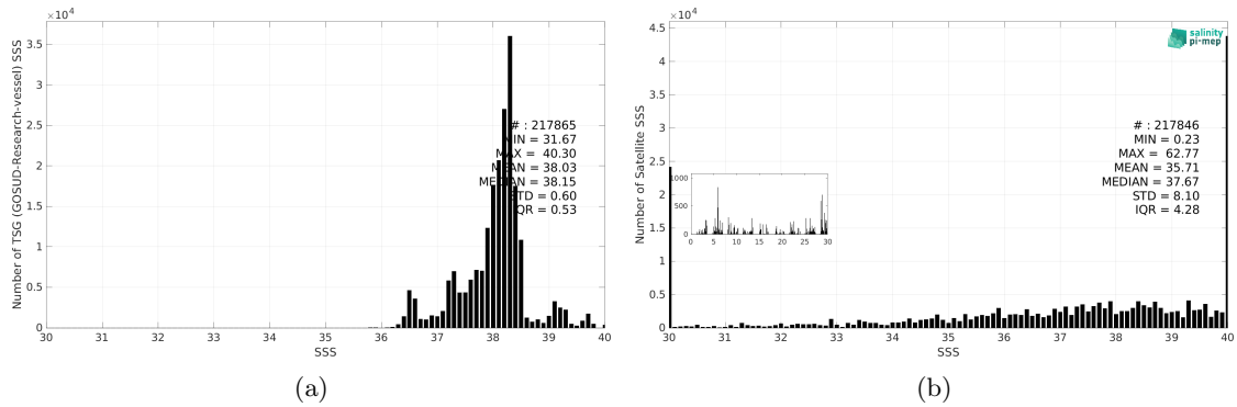
Figure 3: Histograms of SSS from TSG (GOSUD-Research-vessel) (a) and SMOS SSS L2Q v331 - No FLAG (CMEMS-CATDS-CPDC) (b) considering all match-up pairs per bins of 0.1 over the Mediterranean Sea Pi-MEP region and for the full satellite product period.
