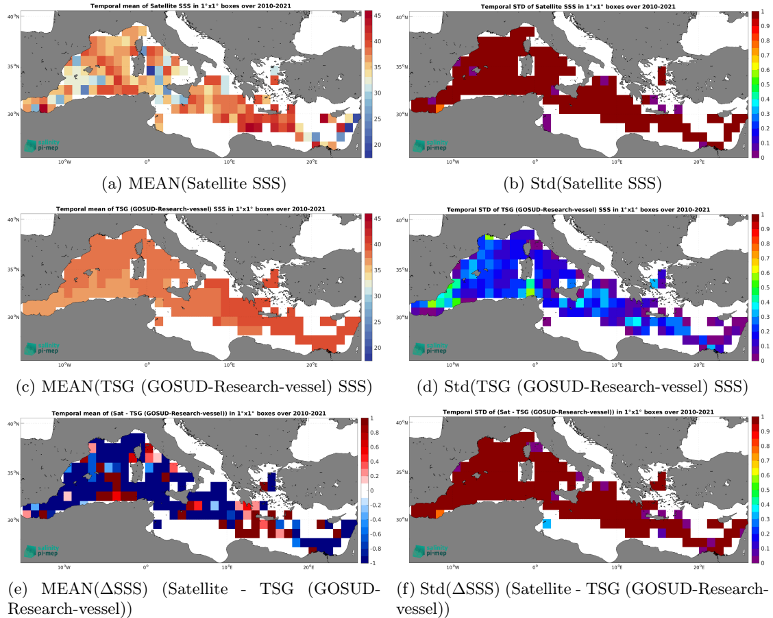
Figure 7: Temporal mean (left) and Std (right) of SSS from SMOS SSS L2Q v331 - No FLAG (CMEMS-CATDS-CPDC) (top), TSG (GOSUD-Research-vessel) (middle), and of \Delta\text{SSS} (Satellite - TSG (GOSUD-Research-vessel)). Only match-up pairs are used to generate these maps.
