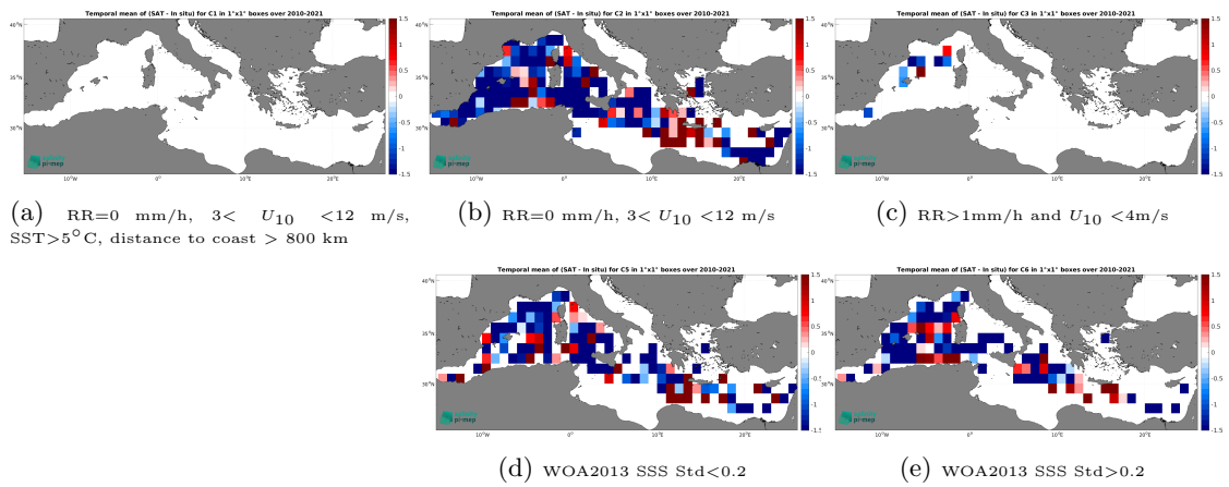
Figure 14: Temporal mean gridded over spatial boxes of size 1^\circ \times 1^\circ of \Delta SSS (SMOS SSS L2Q v331 - No FLAG (CMEMS-CATDS-CPDC) - TSG (GOSUD-Research-vessel)) for 5 different subdatasets corresponding to:RR=0 mm/h, 3 < U_{10} < 12 m/s, SST>5°C, distance to coast > 800 km (a), RR=0 mm/h, 3 < U_{10} < 12 m/s (b), RR>1mm/h and U_{10} < 4 m/s (c), WOA2013 SSS Std<0.2 (d), WOA2013 SSS Std>0.2 (e).
