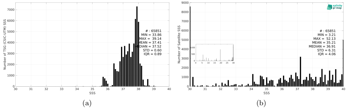
Figure 3: Histograms of SSS from TSG (CSIC-UTM) (a) and SMOS SSS L2Q v331 - No FLAG (CMEMS-CATDS-CPDC) (b) considering all match-up pairs per bins of 0.1 over the Mediterranean Sea Pi-MEP region and for the full satellite product period.
