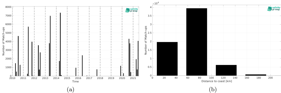
Figure 2: Number of match-ups between TSG (CSIC-UTM) and SMOS SSS L2Q v331 - No FLAG (CMEMS-CATDS-CPDC) SSS as a function of time (a) and as function of the distance to coast (b) over the Mediterranean Sea Pi-MEP region and for the full satellite product period.
