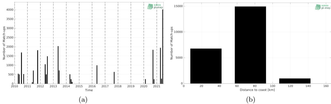
Figure 1: Number of match-ups between TSG (CSIC-UTM) and SMOS SSS L2Q v331 - No FLAG (CMEMS-CATDS-CPDC) SSS as a function of time (a) and as function of the distance to coast (b) over the Mediterranean Sea Pi-MEP region and for the full satellite product period.
