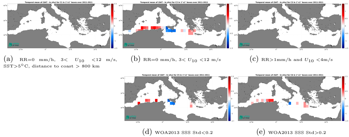
Figure 12: Temporal mean gridded over spatial boxes of size 1^{\circ}\times 1^{\circ} of \Delta\text{SSS} (SMOS SSS L3 v9 - 9 Days (CATDS-CEC-LOCEAN) - TSG (SAMOS)) for 5 different subdatasets corresponding to: RR=0 mm/h, 3 < U_{10} < 12 m/s, SST > 5^{\circ}\text{C} , distance to coast > 800 km (a), RR=0 mm/h, 3 < U_{10} < 12 m/s (b), RR > 1 mm/h and U_{10} < 4 m/s (c), WOA2013 SSS Std < 0.2 (d), WOA2013 SSS Std > 0.2 (e).
