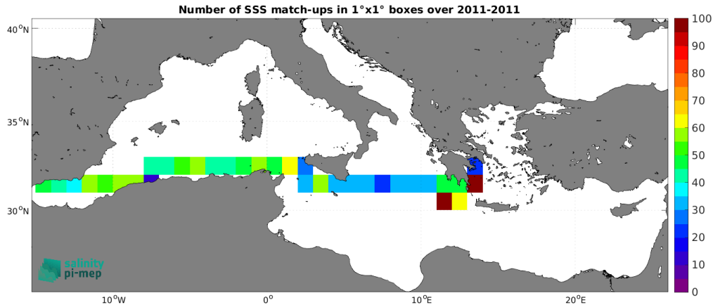
Figure 4: Number of SSS match-ups between TSG (SAMOS) SSS and the SMOS SSS L3 v9 - 9 Days (CATDS-CEC-LOCEAN) SSS product for the Mediterranean Sea Pi-MEP region over 1^\circ \times 1^\circ boxes and for the full satellite product period.
