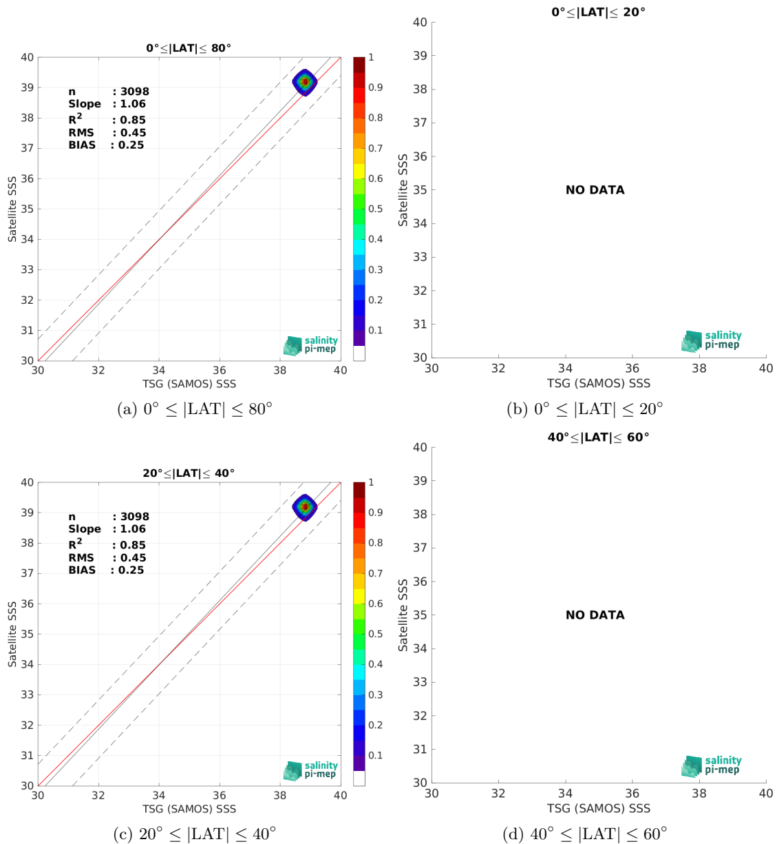
Figure 9: Contour maps of the concentration of SMOS SSS L3 v9 - 9 Days (CATDS-CEC-LOCEAN) SSS (y-axis) versus TSG (SAMOS) SSS (x-axis) at match-up pairs for different latitude bands. For each plot, the red line shows x=y . The black thin and dashed lines indicate a linear fit through the data cloud and the \pm 95\% confidence levels, respectively. The number match-up pairs n , the slope and R^2 coefficient of the linear fit, the root mean square (RMS) and the mean bias between satellite and in situ data are indicated for each latitude band in each plots.
