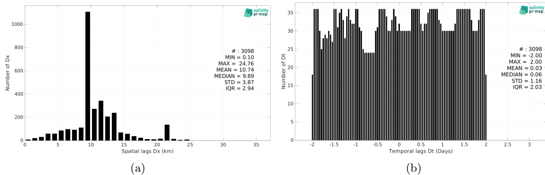
Figure 5: Histograms of the spatial (a) and temporal (b) lags between the location/time of the TSG (SAMOS) measurement and the date of the corresponding SMOS SSS L3 v9 - 9 Days (CATDS-CEC-LOCEAN) SSS pixel.
