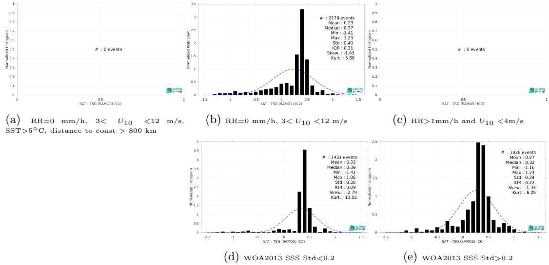
Figure 13: Normalized histogram of \Delta SSS (SMOS SSS L3 v9 - 9 Days (CATDS-CEC-LOCEAN) - TSG (SAMOS)) for 5 different subdatasets corresponding to: RR=0 mm/h, 3 < U_{10} < 12 m/s, SST>5°C, distance to coast > 800 km (a), RR=0 mm/h, 3 < U_{10} < 12 m/s (b), RR>1mm/h and U_{10} < 4 m/s (c), WOA2013 SSS Std<0.2 (d), WOA2013 SSS Std>0.2 (e).
