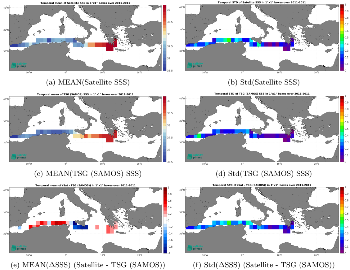
Figure 6: Temporal mean (left) and Std (right) of SSS from SMOS SSS L3 v9 - 9 Days (CATDS-CEC-LOCEAN) (top), TSG (SAMOS) (middle), and of \Delta\text{SSS} (Satellite - TSG (SAMOS)). Only match-up pairs are used to generate these maps.
