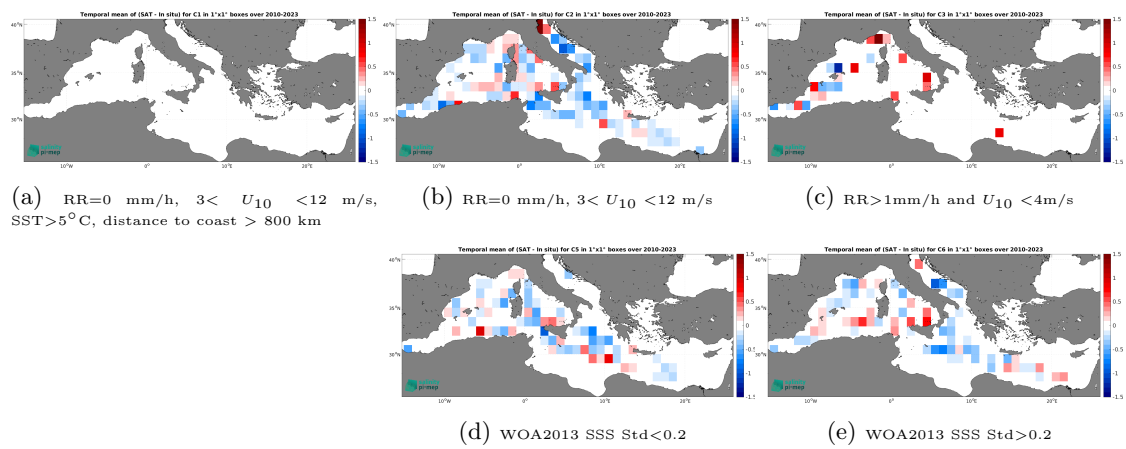
Figure 14: Temporal mean gridded over spatial boxes of size 1^\circ \times 1^\circ of \Delta\text{SSS} (SMOS SSS L3 v9 - 9 Days (CATDS-CEC-LOCEAN) - TSG (LEGOS-DM)) for 5 different subdatasets corresponding to:RR=0 mm/h, 3 < U_{10} < 12 m/s, SST>5°C, distance to coast > 800 km (a), RR=0 mm/h, 3 < U_{10} < 12 m/s (b), RR>1mm/h and U_{10} < 4 m/s (c), WOA2013 SSS Std<0.2 (d), WOA2013 SSS Std>0.2 (e).
