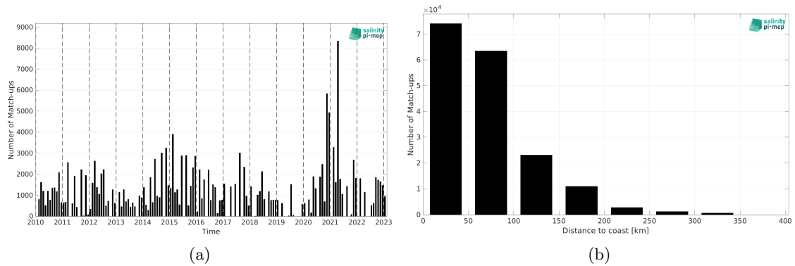
Figure 2: Number of match-ups between TSG (LEGOS-DM) and SMOS SSS L3 v9 - 9 Days (CATDS-CEC-LOCEAN) SSS as a function of time (a) and as function of the distance to coast (b) over the Mediterranean Sea Pi-MEP region and for the full satellite product period.
