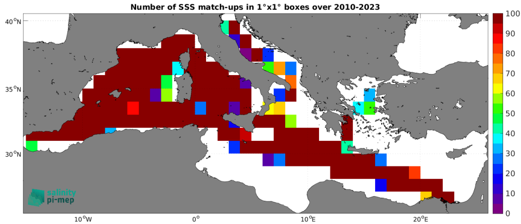
Figure 5: Number of SSS match-ups between TSG (LEGOS-DM) SSS and the SMOS SSS L3 v9 - 9 Days (CATDS-CEC-LOCEAN) SSS product for the Mediterranean Sea Pi-MEP region over 1^\circ \times 1^\circ boxes and for the full satellite product period.
