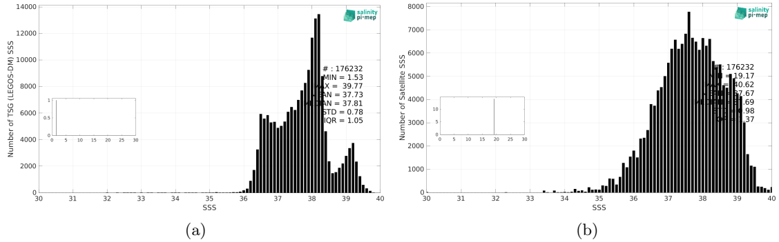
Figure 3: Histograms of SSS from TSG (LEGOS-DM) (a) and SMOS SSS L3 v9 - 9 Days (CATDS-CEC-LOCEAN) (b) considering all match-up pairs per bins of 0.1 over the Mediterranean Sea Pi-MEP region and for the full satellite product period.
