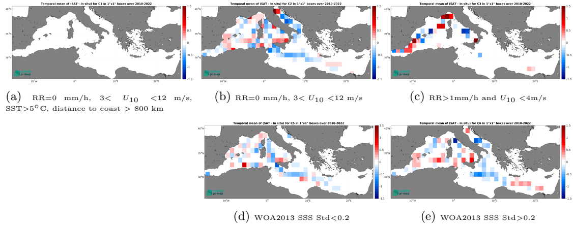
Figure 12: Temporal mean gridded over spatial boxes of size 1^{\circ}\times 1^{\circ} of \Delta\text{SSS} (SMOS SSS L3 v9 - 9 Days (CATDS-CEC-LOCEAN) - TSG (LEGOS-DM)) for 5 different subdatasets corresponding to: RR=0 mm/h, 3 < U_{10} < 12 m/s, SST > 5^{\circ}\text{C} , distance to coast > 800 km (a), RR=0 mm/h, 3 < U_{10} < 12 m/s (b), RR > 1 mm/h and U_{10} < 4 m/s (c), WOA2013 SSS Std < 0.2 (d), WOA2013 SSS Std > 0.2 (e).
