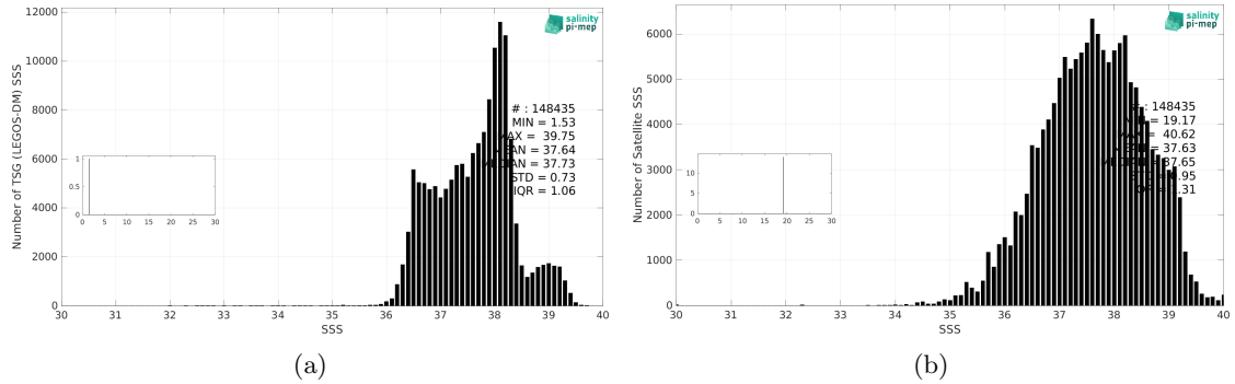
Figure 2: Histograms of SSS from TSG (LEGOS-DM) (a) and SMOS SSS L3 v9 - 9 Days (CATDS-CEC-LOCEAN) (b) considering all match-up pairs per bins of 0.1 over the Mediterranean Sea Pi-MEP region and for the full satellite product period.
