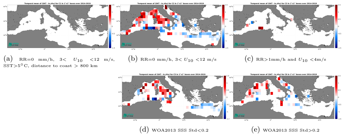
Figure 12: Temporal mean gridded over spatial boxes of size 1^{\circ}\times 1^{\circ} of \Delta SSS (SMOS SSS L3 v9 - 9 Days (CATDS-CEC-LOCEAN) - TSG (GOSUD-Sailing-ship)) for 5 different subdatasets corresponding to: RR=0 mm/h, 3 < U_{10} < 12 m/s, SST > 5^{\circ}\text{C} , distance to coast > 800 km (a), RR=0 mm/h, 3 < U_{10} < 12 m/s (b), RR > 1 mm/h and U_{10} < 4 m/s (c), WOA2013 SSS Std < 0.2 (d), WOA2013 SSS Std > 0.2 (e).
