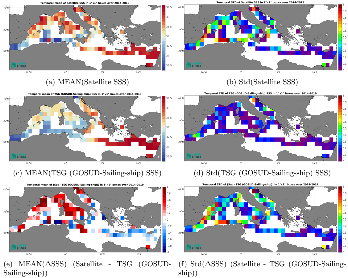
Figure 6: Temporal mean (left) and Std (right) of SSS from SMOS SSS L3 v9 - 9 Days (CATDS-CEC-LOCEAN) (top), TSG (GOSUD-Sailing-ship) (middle), and of \Delta\text{SSS} (Satellite - TSG (GOSUD-Sailing-ship)). Only match-up pairs are used to generate these maps.
