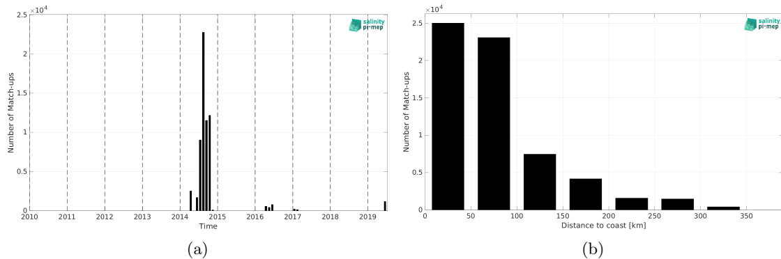
Figure 1: Number of match-ups between TSG (GOSUD-Sailing-ship) and SMOS SSS L3 v9 - 9 Days (CATDS-CEC-LOCEAN) SSS as a function of time (a) and as function of the distance to coast (b) over the Mediterranean Sea Pi-MEP region and for the full satellite product period.
