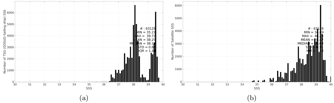
Figure 2: Histograms of SSS from TSG (GOSUD-Sailing-ship) (a) and SMOS SSS L3 v9 - 9 Days (CATDS-CEC-LOCEAN) (b) considering all match-up pairs per bins of 0.1 over the Mediterranean Sea Pi-MEP region and for the full satellite product period.
