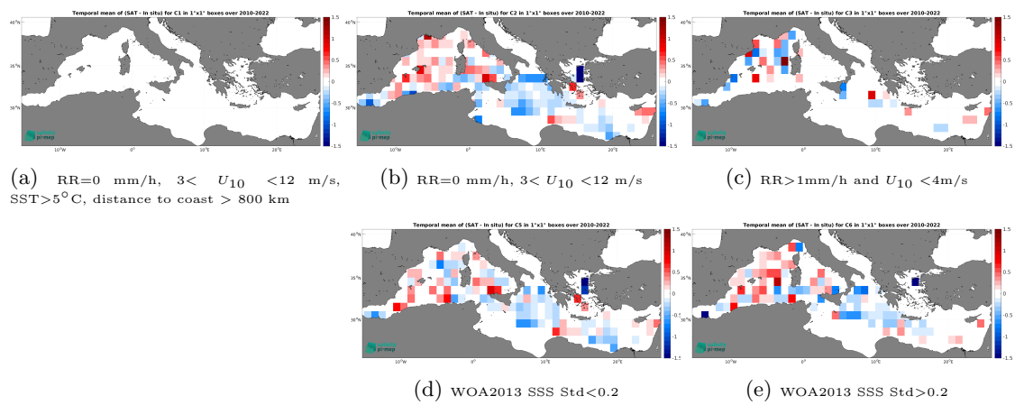
Figure 14: Temporal mean gridded over spatial boxes of size 1^\circ \times 1^\circ of \Delta\text{SSS} (SMOS SSS L3 v9 - 9 Days (CATDS-CEC-LOCEAN) - TSG (GOSUD-Research-vessel)) for 5 different subdatasets corresponding to:RR=0 mm/h, 3 < U_{10} < 12 m/s, SST>5°C, distance to coast > 800 km (a), RR=0 mm/h, 3 < U_{10} < 12 m/s (b), RR>1mm/h and U_{10} < 4 m/s (c), WOA2013 SSS Std<0.2 (d), WOA2013 SSS Std>0.2 (e).
