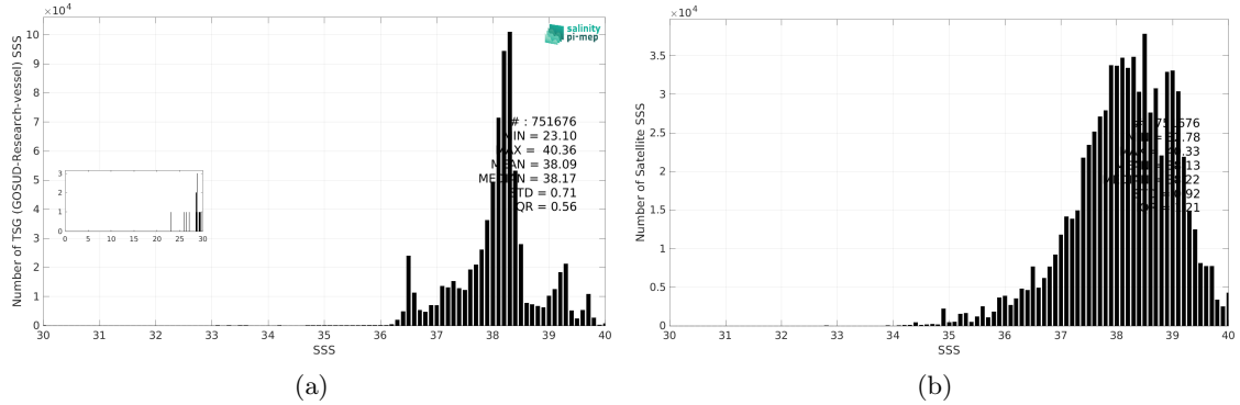
Figure 3: Histograms of SSS from TSG (GOSUD-Research-vessel) (a) and SMOS SSS L3 v9 - 9 Days (CATDS-CEC-LOCEAN) (b) considering all match-up pairs per bins of 0.1 over the Mediterranean Sea Pi-MEP region and for the full satellite product period.
