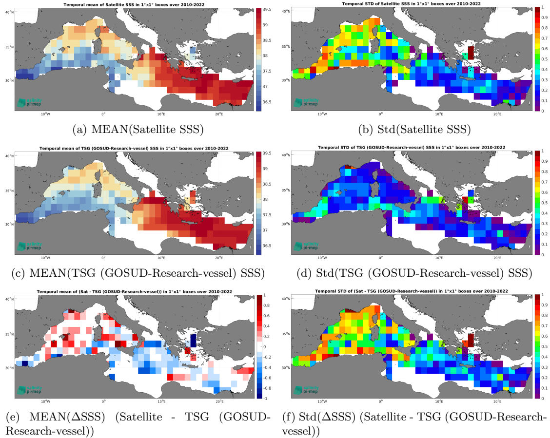
Figure 7: Temporal mean (left) and Std (right) of SSS from SMOS SSS L3 v9 - 9 Days (CATDS-CEC-LOCEAN) (top), TSG (GOSUD-Research-vessel) (middle), and of \Delta\text{SSS} (Satellite - TSG (GOSUD-Research-vessel)). Only match-up pairs are used to generate these maps.
