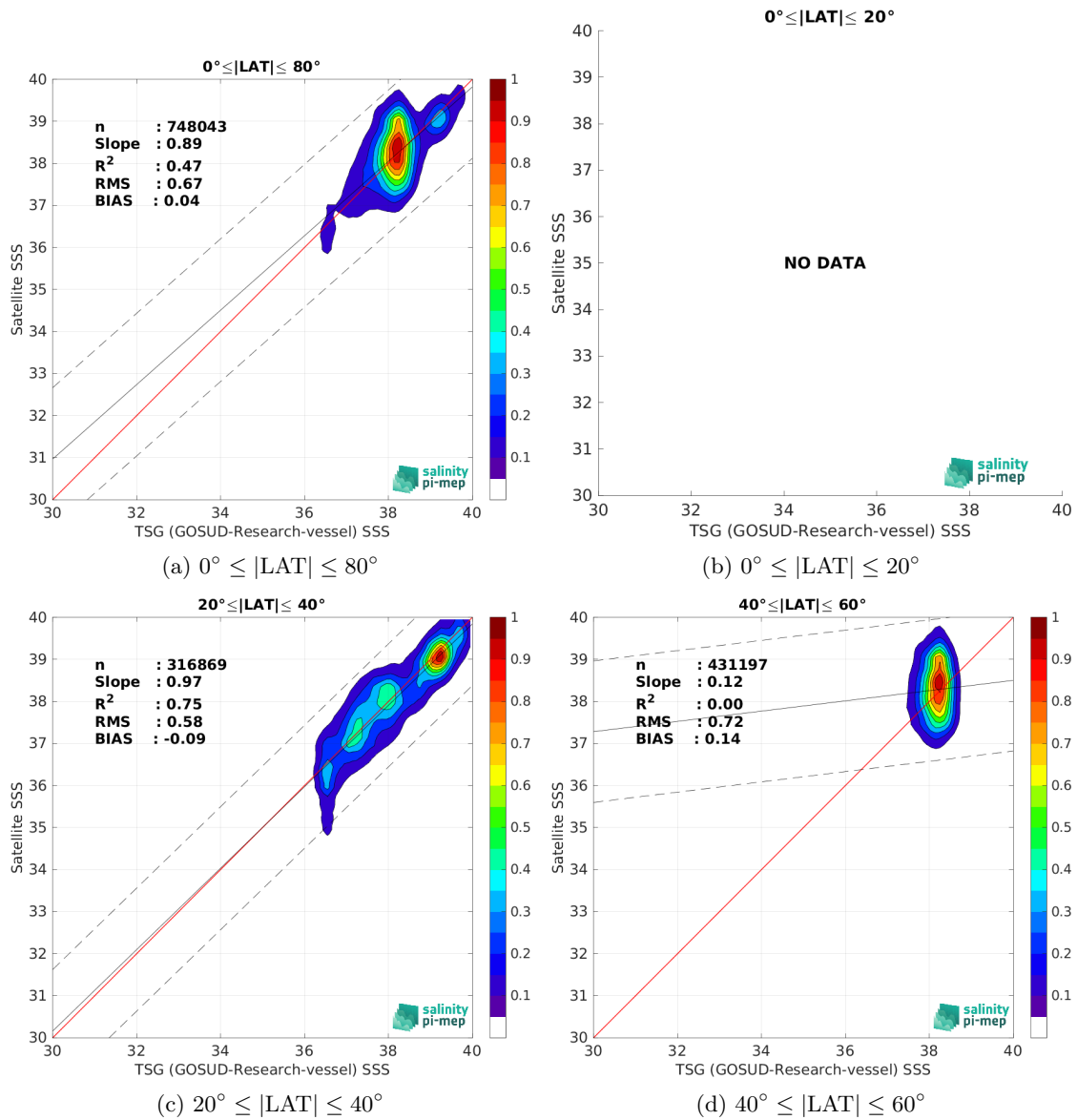
Figure 10: Contour maps of the concentration of SMOS SSS L3 v9 - 9 Days (CATDS-CEC-LOCEAN) SSS (y-axis) versus TSG (GOSUD-Research-vessel) SSS (x-axis) at match-up pairs for different latitude bands. For each plot, the red line shows x=y . The black thin and dashed lines indicate a linear fit through the data cloud and the \pm 95\% confidence levels, respectively. The number match-up pairs n , the slope and R^2 coefficient of the linear fit, the root mean square (RMS) and the mean bias between satellite and in situ data are indicated for each latitude band in each plots.
