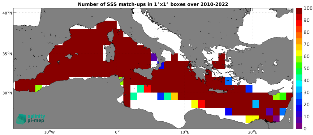
Figure 5: Number of SSS match-ups between TSG (GOSUD-Research-vessel) SSS and the SMOS SSS L3 v9 - 9 Days (CATDS-CEC-LOCEAN) SSS product for the Mediterranean Sea Pi-MEP region over 1^\circ \times 1^\circ boxes and for the full satellite product period.
