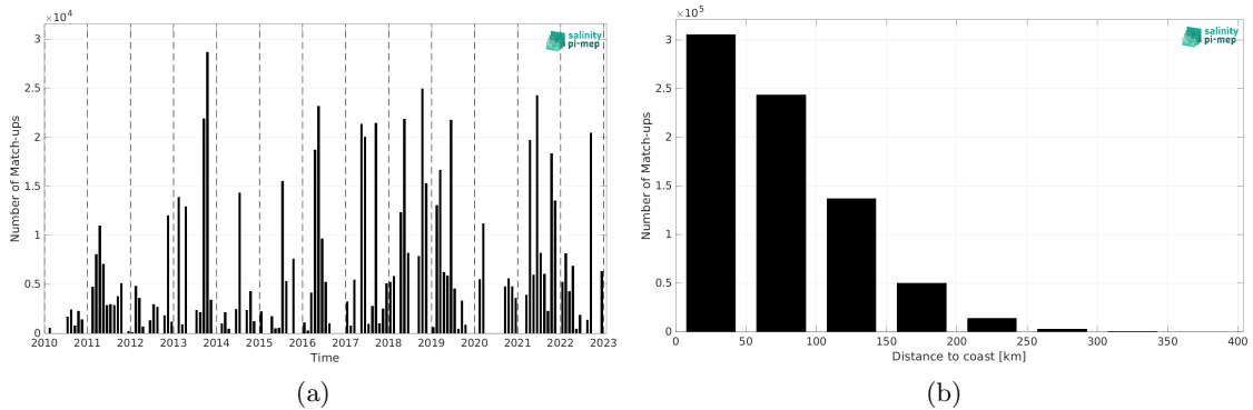
Figure 2: Number of match-ups between TSG (GOSUD-Research-vessel) and SMOS SSS L3 v9 - 9 Days (CATDS-CEC-LOCEAN) SSS as a function of time (a) and as function of the distance to coast (b) over the Mediterranean Sea Pi-MEP region and for the full satellite product period.
