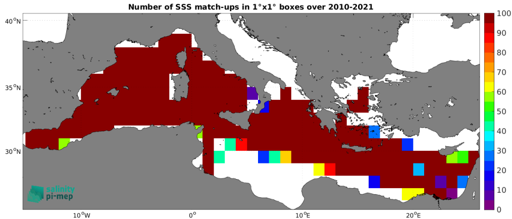
Figure 4: Number of SSS match-ups between TSG (GOSUD-Research-vessel) SSS and the SMOS SSS L3 v9 - 9 Days (CATDS-CEC-LOCEAN) SSS product for the Mediterranean Sea Pi-MEP region over 1^\circ \times 1^\circ boxes and for the full satellite product period.
