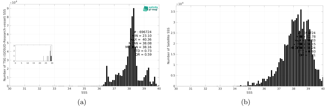
Figure 2: Histograms of SSS from TSG (GOSUD-Research-vessel) (a) and SMOS SSS L3 v9 - 9 Days (CATDS-CEC-LOCEAN) (b) considering all match-up pairs per bins of 0.1 over the Mediterranean Sea Pi-MEP region and for the full satellite product period.
