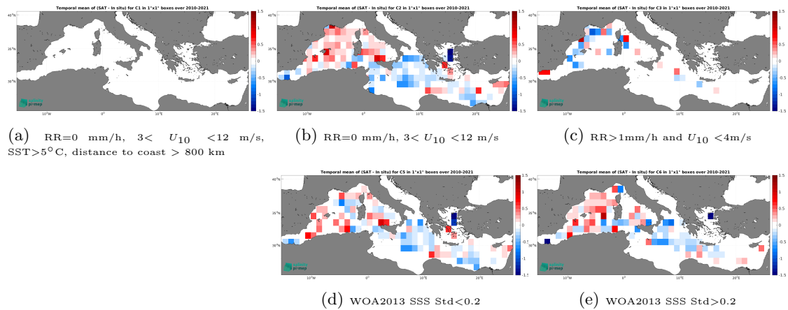
Figure 12: Temporal mean gridded over spatial boxes of size 1^{\circ}\times 1^{\circ} of \Delta SSS (SMOS SSS L3 v9 - 9 Days (CATDS-CEC-LOCEAN) - TSG (GOSUD-Research-vessel)) for 5 different subdatasets corresponding to:RR=0 mm/h, 3 < U_{10} < 12 m/s, SST >5^{\circ}\text{C} , distance to coast > 800 km (a), RR=0 mm/h, 3 < U_{10} < 12 m/s (b), RR >1 mm/h and U_{10} < 4 m/s (c), WOA2013 SSS Std <0.2 (d), WOA2013 SSS Std >0.2 (e).
