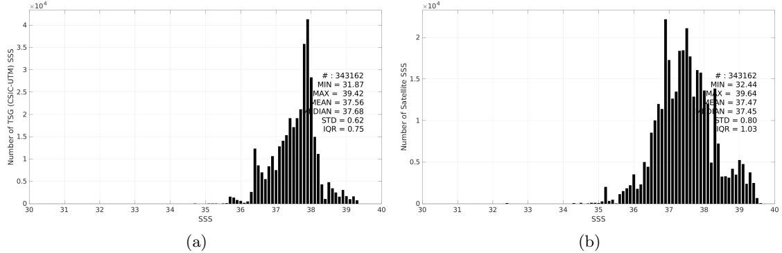
Figure 3: Histograms of SSS from TSG (CSIC-UTM) (a) and SMOS SSS L3 v9 - 9 Days (CATDS-CEC-LOCEAN) (b) considering all match-up pairs per bins of 0.1 over the Mediterranean Sea Pi-MEP region and for the full satellite product period.
