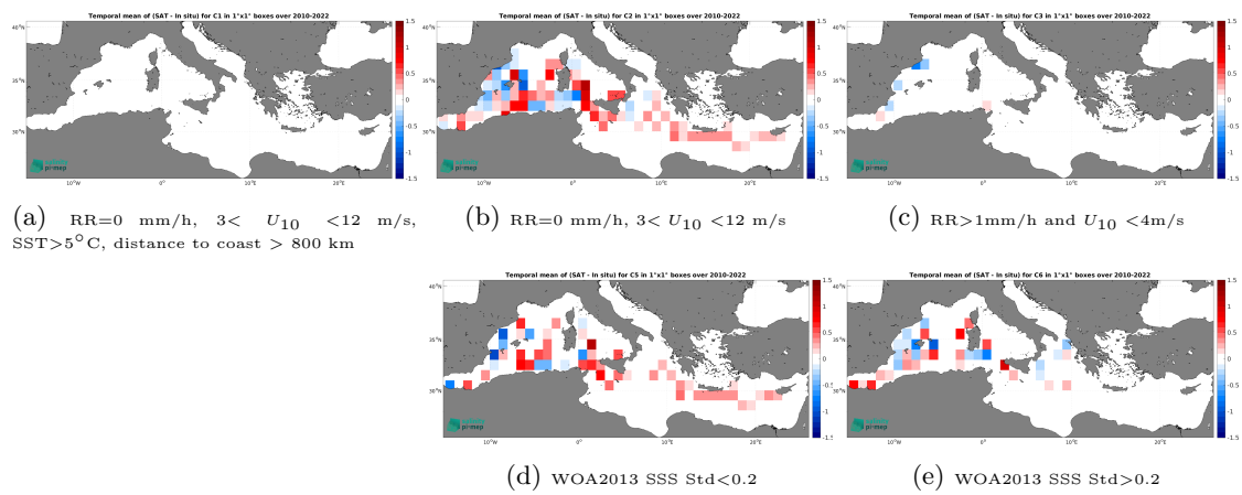
Figure 14: Temporal mean gridded over spatial boxes of size 1^\circ \times 1^\circ of \Delta\text{SSS} (SMOS SSS L3 v9 - 9 Days (CATDS-CEC-LOCEAN) - TSG (CSIC-UTM)) for 5 different subdatasets corresponding to:RR=0 mm/h, 3 < U_{10} < 12 m/s, SST >5^\circ\text{C} , distance to coast > 800 km (a), RR=0 mm/h, 3 < U_{10} < 12 m/s (b), RR >1 mm/h and U_{10} < 4 m/s (c), WOA2013 SSS Std <0.2 (d), WOA2013 SSS Std >0.2 (e).
