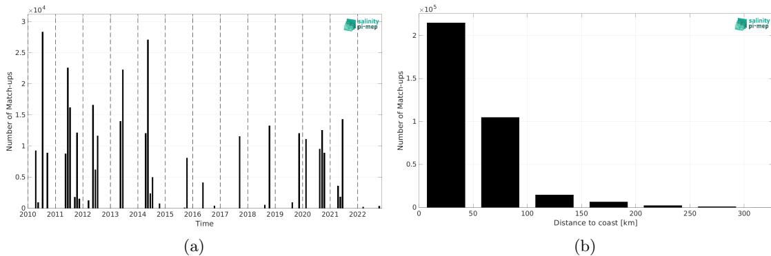
Figure 2: Number of match-ups between TSG (CSIC-UTM) and SMOS SSS L3 v9 - 9 Days (CATDS-CEC-LOCEAN) SSS as a function of time (a) and as function of the distance to coast (b) over the Mediterranean Sea Pi-MEP region and for the full satellite product period.
