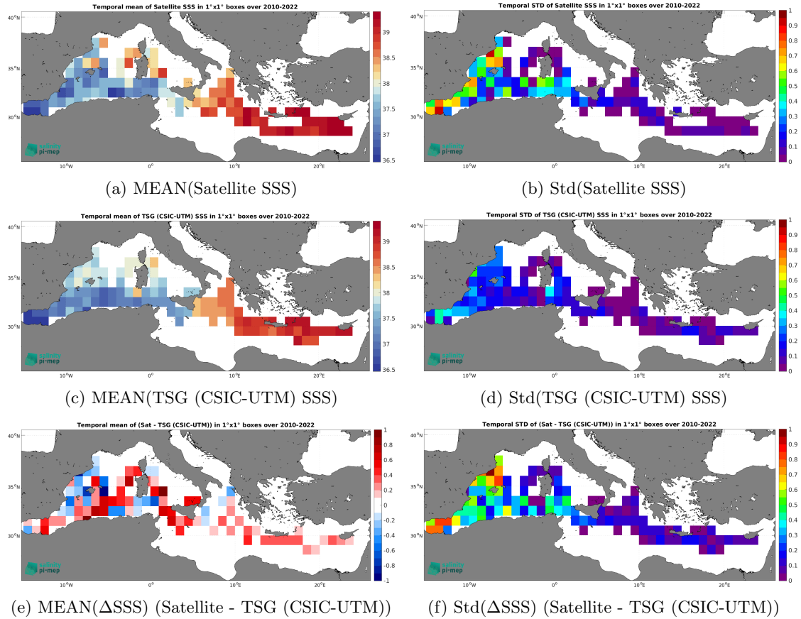
Figure 7: Temporal mean (left) and Std (right) of SSS from SMOS SSS L3 v9 - 9 Days (CATDS-CEC-LOCEAN) (top), TSG (CSIC-UTM) (middle), and of \Delta\text{SSS} (Satellite - TSG (CSIC-UTM)). Only match-up pairs are used to generate these maps.
