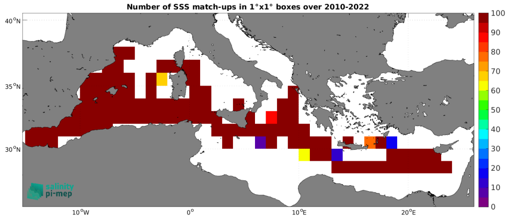
Figure 4: Number of SSS match-ups between TSG (CSIC-UTM) SSS and the SMOS SSS L3 v9 - 9 Days (CATDS-CEC-LOCEAN) SSS product for the Mediterranean Sea Pi-MEP region over 1^\circ \times 1^\circ boxes and for the full satellite product period.
