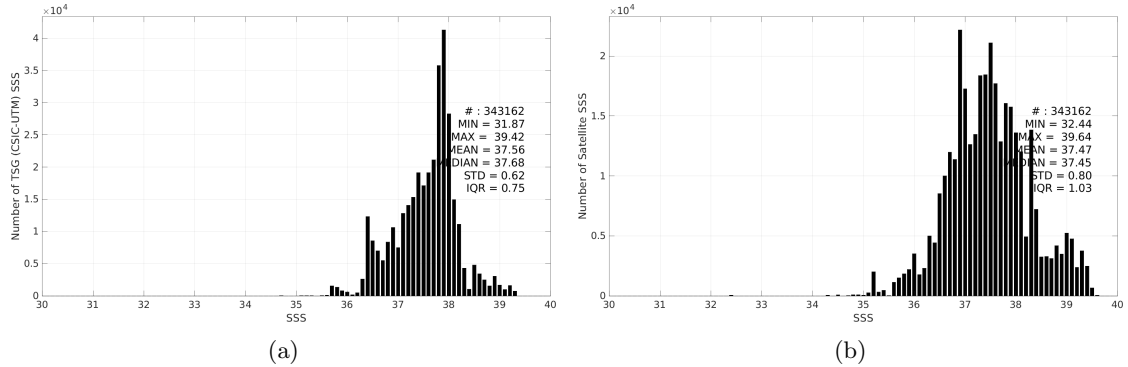
Figure 2: Histograms of SSS from TSG (CSIC-UTM) (a) and SMOS SSS L3 v9 - 9 Days (CATDS-CEC-LOCEAN) (b) considering all match-up pairs per bins of 0.1 over the Mediterranean Sea Pi-MEP region and for the full satellite product period.
