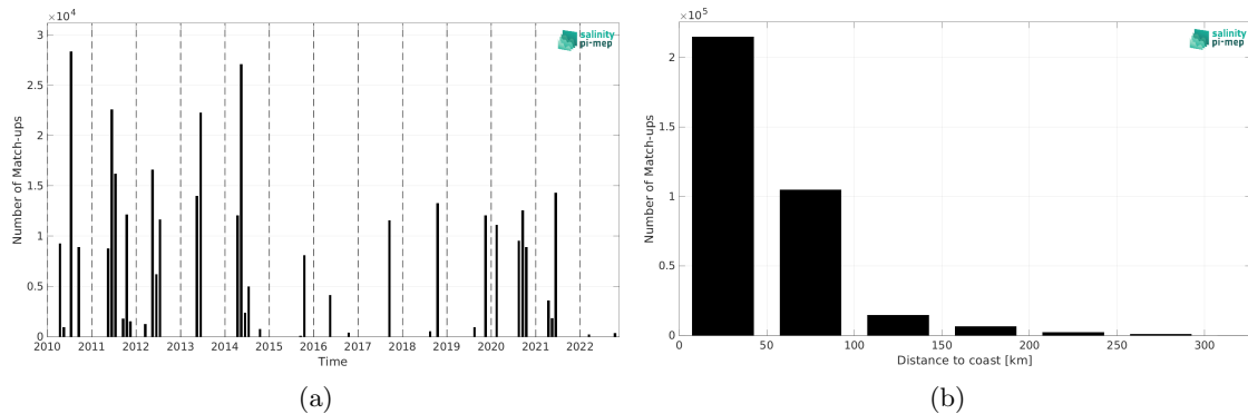
Figure 1: Number of match-ups between TSG (CSIC-UTM) and SMOS SSS L3 v9 - 9 Days (CATDS-CEC-LOCEAN) SSS as a function of time (a) and as function of the distance to coast (b) over the Mediterranean Sea Pi-MEP region and for the full satellite product period.
