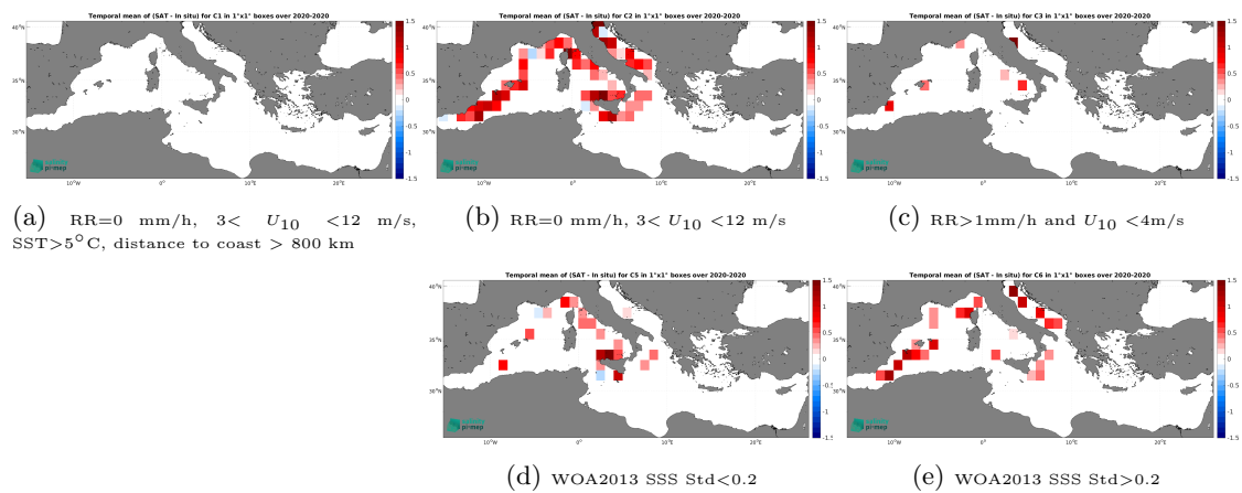
Figure 14: Temporal mean gridded over spatial boxes of size 1^\circ \times 1^\circ of \Delta SSS (SMOS SSS L3 v9 - 9 Days (CATDS-CEC-LOCEAN) - Saildrone) for 5 different subdatasets corresponding to:RR=0 mm/h, 3 < U_{10} < 12 m/s, SST >5^\circ\text{C} , distance to coast > 800 km (a), RR=0 mm/h, 3 < U_{10} < 12 m/s (b), RR >1 mm/h and U_{10} < 4 m/s (c), WOA2013 SSS Std <0.2 (d), WOA2013 SSS Std >0.2 (e).
