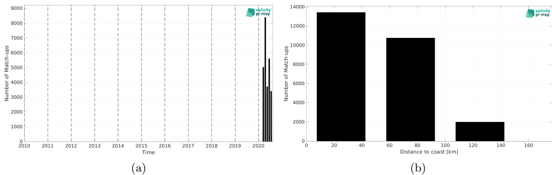
Figure 2: Number of match-ups between Saildrone and SMOS SSS L3 v9 - 9 Days (CATDS-CEC-LOCEAN) SSS as a function of time (a) and as function of the distance to coast (b) over the Mediterranean Sea Pi-MEP region and for the full satellite product period.
