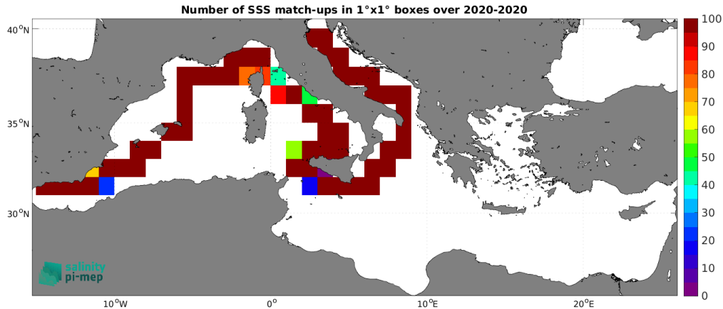
Figure 5: Number of SSS match-ups between Saildrone SSS and the SMOS SSS L3 v9 - 9 Days (CATDS-CEC-LOCEAN) SSS product for the Mediterranean Sea Pi-MEP region over 1^\circ \times 1^\circ boxes and for the full satellite product period.
