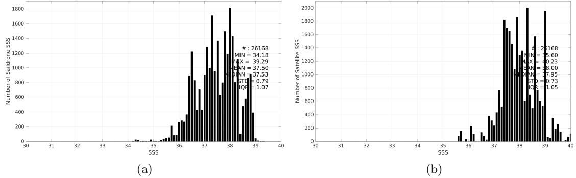
Figure 3: Histograms of SSS from Saildrone (a) and SMOS SSS L3 v9 - 9 Days (CATDS-CEC-LOCEAN) (b) considering all match-up pairs per bins of 0.1 over the Mediterranean Sea Pi-MEP region and for the full satellite product period.
