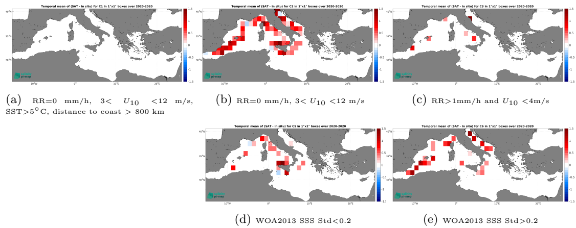
Figure 14: Temporal mean gridded over spatial boxes of size 1^\circ \times 1^\circ of \Delta\text{SSS} (SMOS SSS L3 v9 - 9 Days (CATDS-CEC-LOCEAN) - Saildrone) for 5 different subdatasets corresponding to:RR=0 mm/h, 3 < U_{10} < 12 m/s, SST>5°C, distance to coast > 800 km (a), RR=0 mm/h, 3 < U_{10} < 12 m/s (b), RR>1mm/h and U_{10} < 4 m/s (c), WOA2013 SSS Std<0.2 (d), WOA2013 SSS Std>0.2 (e).
