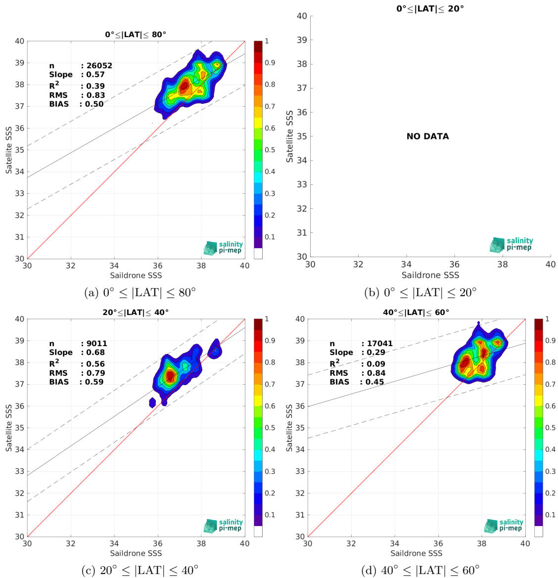
Figure 9: Contour maps of the concentration of SMOS SSS L3 v9 - 9 Days (CATDS-CEC-LOCEAN) SSS (y-axis) versus Sailldrone SSS (x-axis) at match-up pairs for different latitude bands. For each plot, the red line shows x=y . The black thin and dashed lines indicate a linear fit through the data cloud and the \pm 95\% confidence levels, respectively. The number match-up pairs n , the slope and R^2 coefficient of the linear fit, the root mean square (RMS) and the mean bias between satellite and in situ data are indicated for each latitude band in each plots.
