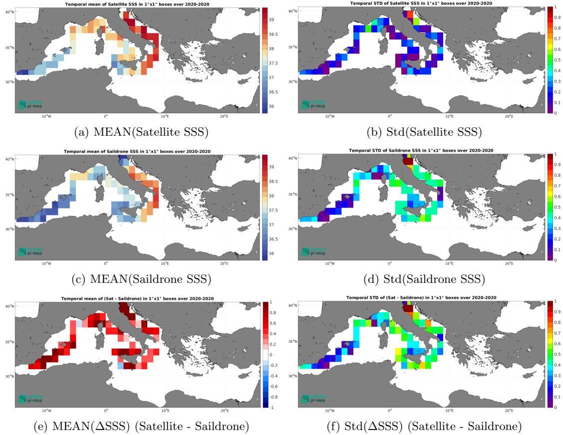
Figure 6: Temporal mean (left) and Std (right) of SSS from SMOS SSS L3 v9 - 9 Days (CATDS-CEC-LOCEAN) (top), Sairdrone (middle), and of \Delta SSS (Satellite - Sairdrone). Only match-up pairs are used to generate these maps.
