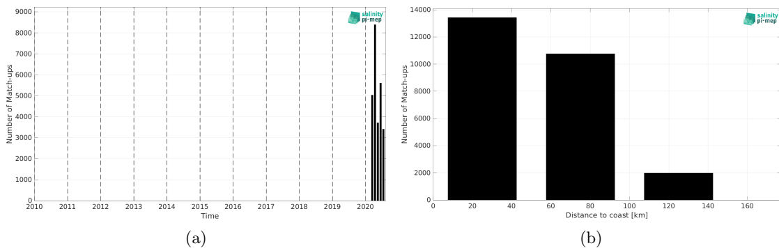
Figure 1: Number of match-ups between Saildrone and SMOS SSS L3 v9 - 9 Days (CATDS-CEC-LOCEAN) SSS as a function of time (a) and as function of the distance to coast (b) over the Mediterranean Sea Pi-MEP region and for the full satellite product period.
