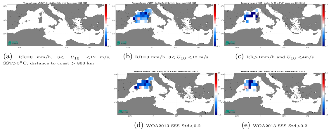
Figure 11: Temporal mean gridded over spatial boxes of size 1^{\circ}\times 1^{\circ} of \Delta\text{SSS} (SMOS SSS L3 v9 - 9 Days (CATDS-CEC-LOCEAN) - Surface drifters) for 5 different subdatasets corresponding to:RR=0 mm/h, 3 < U_{10} < 12 m/s, SST >5^{\circ}\text{C} , distance to coast > 800 km (a), RR=0 mm/h, 3 < U_{10} < 12 m/s (b), RR >1 mm/h and U_{10} < 4 m/s (c), WOA2013 SSS Std <0.2 (d), WOA2013 SSS Std >0.2 (e).
