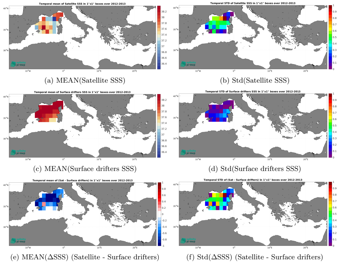
Figure 5: Temporal mean (left) and Std (right) of SSS from SMOS SSS L3 v9 - 9 Days (CATDS-CEC-LOCEAN) (top), Surface drifters (middle), and of \Delta SSS (Satellite - Surface drifters). Only match-up pairs are used to generate these maps.
