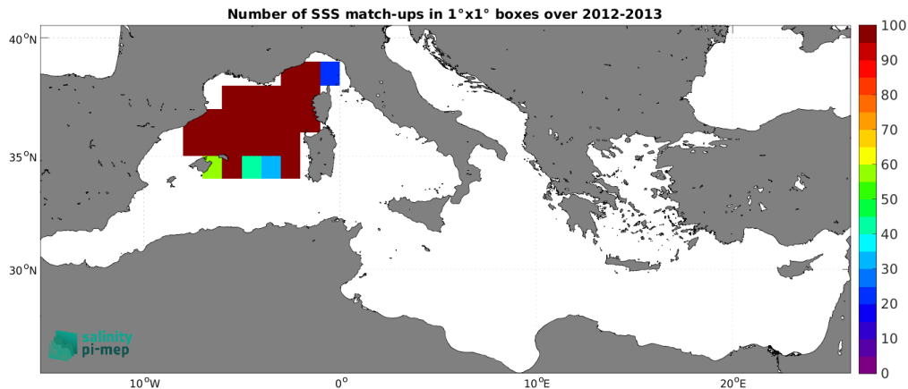
Figure 3: Number of SSS match-ups between Surface drifters SSS and the SMOS SSS L3 v9 - 9 Days (CATDS-CEC-LOCEAN) SSS product for the Mediterranean Sea Pi-MEP region over 1^\circ \times 1^\circ boxes and for the full satellite product period.
