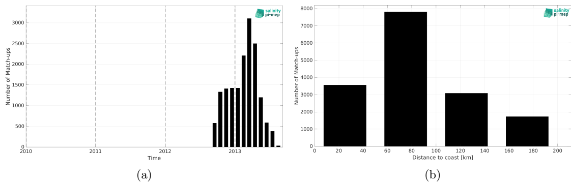
Figure 1: Number of match-ups between Surface drifters and SMOS SSS L3 v9 - 9 Days (CATDS-CEC-LOCEAN) SSS as a function of time (a) and as function of the distance to coast (b) over the Mediterranean Sea Pi-MEP region and for the full satellite product period.
