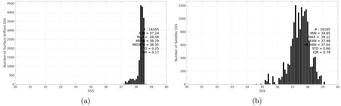
Figure 2: Histograms of SSS from Surface drifters (a) and SMOS SSS L3 v9 - 9 Days (CATDS-CEC-LOCEAN) (b) considering all match-up pairs per bins of 0.1 over the Mediterranean Sea Pi-MEP region and for the full satellite product period.
