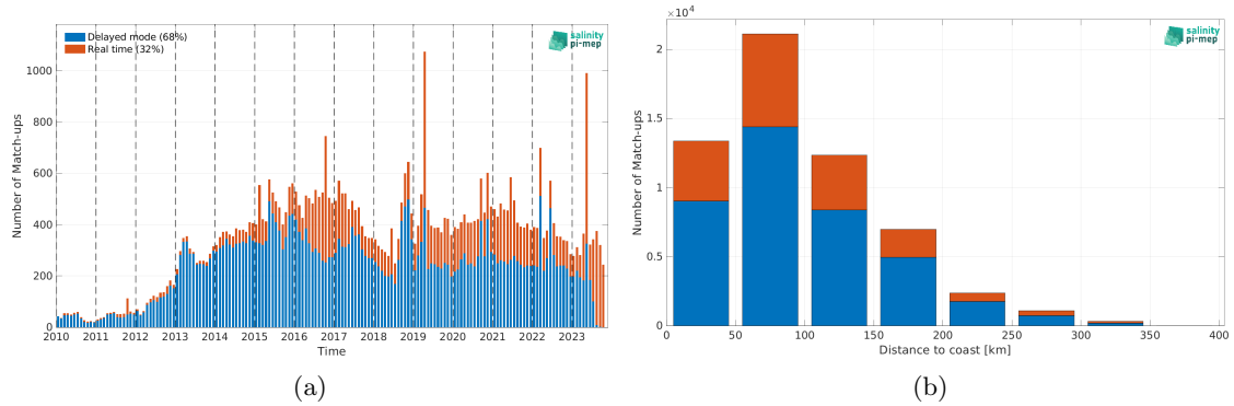
Figure 1: Number of match-ups between Argo and SMOS SSS L3 v9 - 9 Days (CATDS-CEC-LOCEAN) SSS as a function of time (a) and as function of the distance to coast (b) over the Mediterranean Sea Pi-MEP region and for the full satellite product period.
