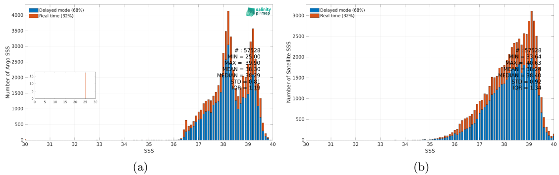
Figure 2: Histograms of SSS from Argo (a) and SMOS SSS L3 v9 - 9 Days (CATDS-CEC-LOCEAN) (b) considering all match-up pairs per bins of 0.1 over the Mediterranean Sea Pi-MEP region and for the full satellite product period.
