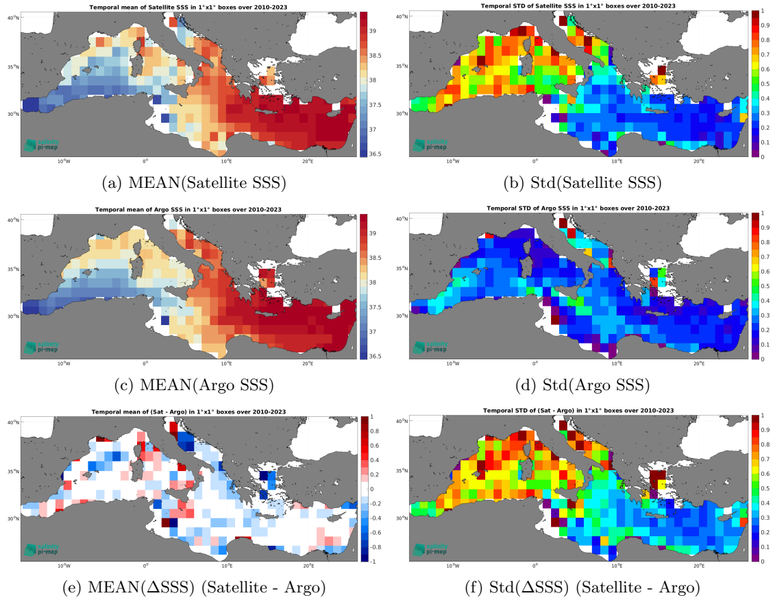
Figure 6: Temporal mean (left) and Std (right) of SSS from SMOS SSS L3 v9 - 9 Days (CATDS-CEC-LOCEAN) (top), Argo (middle), and of \Delta SSS (Satellite - Argo). Only match-up pairs are used to generate these maps.
