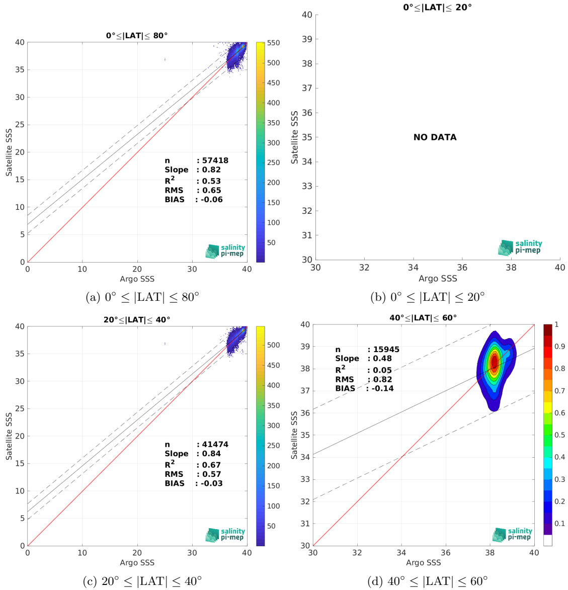
Figure 9: Contour maps of the concentration of SMOS SSS L3 v9 - 9 Days (CATDS-CEC-LOCEAN) SSS (y-axis) versus Argo SSS (x-axis) at match-up pairs for different latitude bands. For each plot, the red line shows x=y . The black thin and dashed lines indicate a linear fit through the data cloud and the \pm 95\% confidence levels, respectively. The number match-up pairs n , the slope and R^2 coefficient of the linear fit, the root mean square (RMS) and the mean bias between satellite and in situ data are indicated for each latitude band in each plots.
