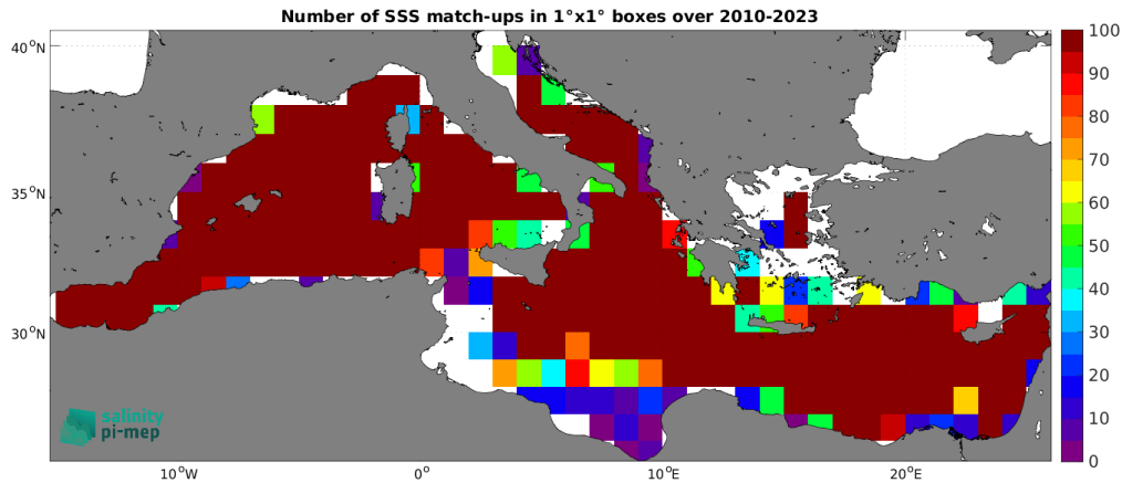
Figure 4: Number of SSS match-ups between Argo SSS and the SMOS SSS L3 v9 - 9 Days (CATDS-CEC-LOCEAN) SSS product for the Mediterranean Sea Pi-MEP region over 1^\circ \times 1^\circ boxes and for the full satellite product period.
