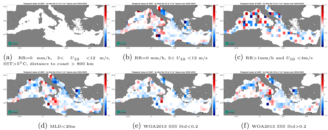
Figure 12: Temporal mean gridded over spatial boxes of size 1^\circ \times 1^\circ of \Delta SSS (SMOS SSS L3 v9 - 9 Days (CATDS-CEC-LOCEAN) - Argo) for 6 different subdatasets corresponding to:RR=0 mm/h, 3 < U_{10} < 12 m/s, SST >5^\circ C, distance to coast > 800 km (a), RR=0 mm/h, 3 < U_{10} < 12 m/s (b), RR >1 mm/h and U_{10} < 4 m/s (c),MLD <20 m (d),WOA2013 SSS Std <0.2 (e),WOA2013 SSS Std >0.2 (f).
