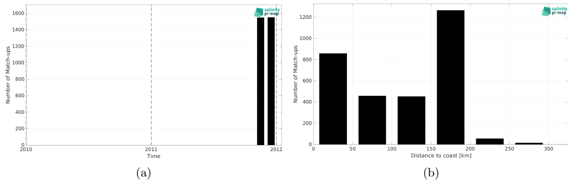
Figure 2: Number of match-ups between TSG (SAMOS) and SMOS SSS L3 v9 - 18 Days (CATDS-CEC-LOCEAN) SSS as a function of time (a) and as function of the distance to coast (b) over the Mediterranean Sea Pi-MEP region and for the full satellite product period.
