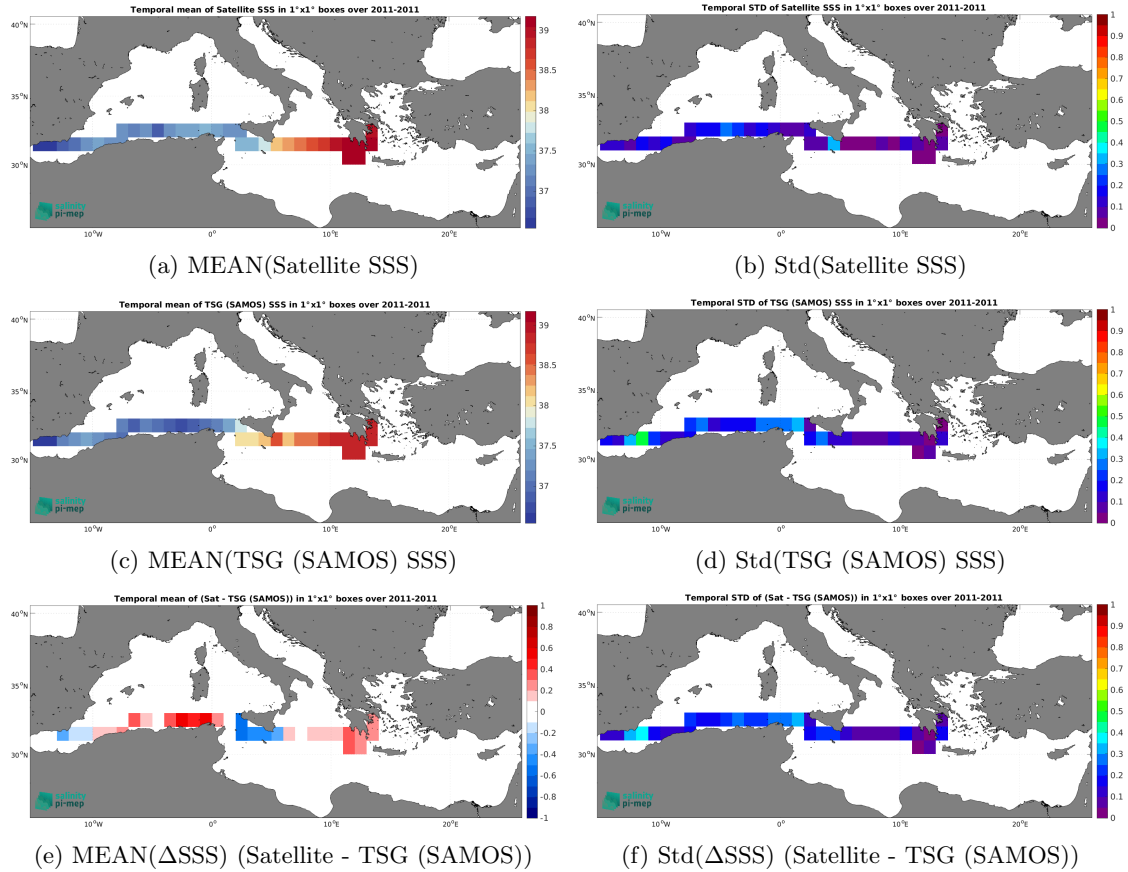
Figure 7: Temporal mean (left) and Std (right) of SSS from SMOS SSS L3 v9 - 18 Days (CATDS-CEC-LOCEAN) (top), TSG (SAMOS) (middle), and of \Delta\text{SSS} (Satellite - TSG (SAMOS)). Only match-up pairs are used to generate these maps.
