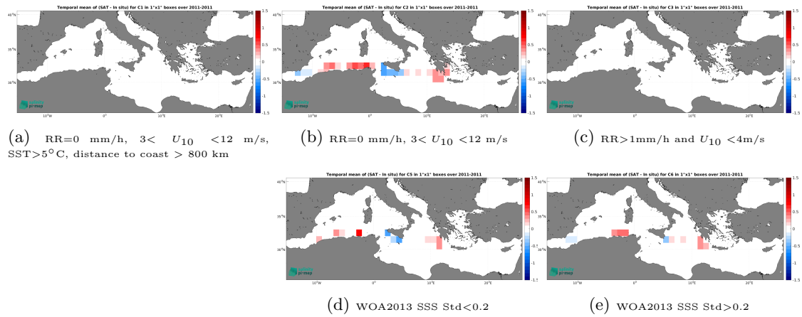
Figure 12: Temporal mean gridded over spatial boxes of size 1^{\circ}\times 1^{\circ} of \Delta\text{SSS} (SMOS SSS L3 v9 - 18 Days (CATDS-CEC-LOCEAN) - TSG (SAMOS)) for 5 different subdatasets corresponding to:RR=0 mm/h, 3 < U_{10} < 12 m/s, SST > 5^{\circ}\text{C} , distance to coast > 800 km (a), RR=0 mm/h, 3 < U_{10} < 12 m/s (b), RR > 1 mm/h and U_{10} < 4 m/s (c), WOA2013 SSS Std < 0.2 (d), WOA2013 SSS Std > 0.2 (e).
