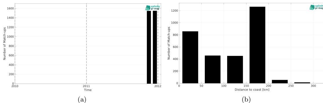
Figure 1: Number of match-ups between TSG (SAMOS) and SMOS SSS L3 v9 - 18 Days (CATDS-CEC-LOCEAN) SSS as a function of time (a) and as function of the distance to coast (b) over the Mediterranean Sea Pi-MEP region and for the full satellite product period.
