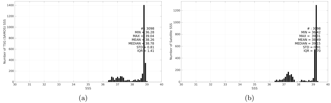
Figure 2: Histograms of SSS from TSG (SAMOS) (a) and SMOS SSS L3 v9 - 18 Days (CATDS-CEC-LOCEAN) (b) considering all match-up pairs per bins of 0.1 over the Mediterranean Sea Pi-MEP region and for the full satellite product period.
