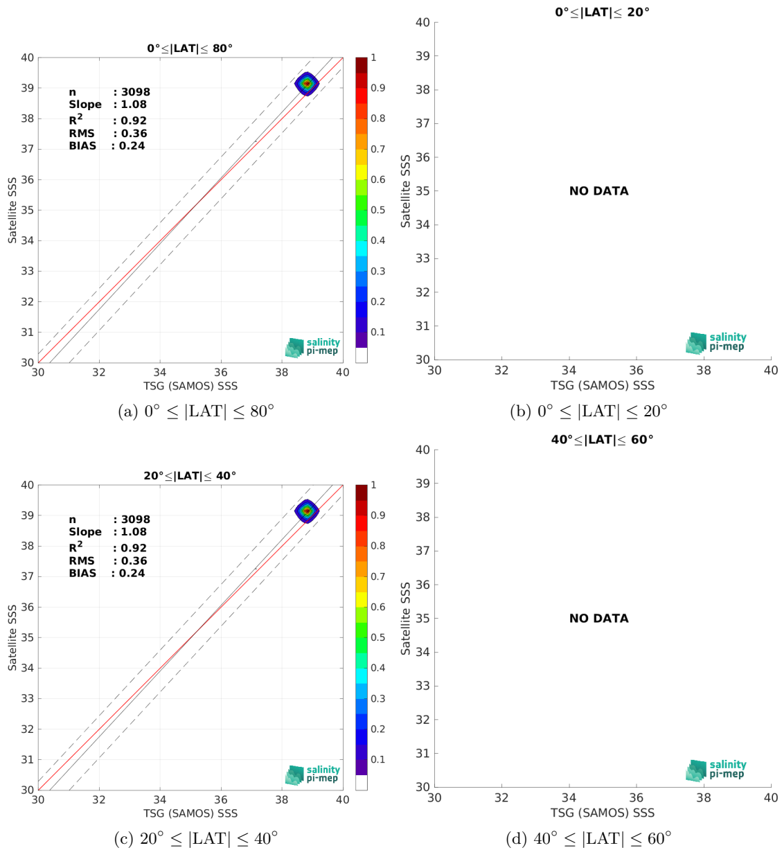
Figure 9: Contour maps of the concentration of SMOS SSS L3 v9 - 18 Days (CATDS-CEC-LOCEAN) SSS (y-axis) versus TSG (SAMOS) SSS (x-axis) at match-up pairs for different latitude bands. For each plot, the red line shows x=y . The black thin and dashed lines indicate a linear fit through the data cloud and the \pm 95\% confidence levels, respectively. The number match-up pairs n , the slope and R^2 coefficient of the linear fit, the root mean square (RMS) and the mean bias between satellite and in situ data are indicated for each latitude band in each plots.
