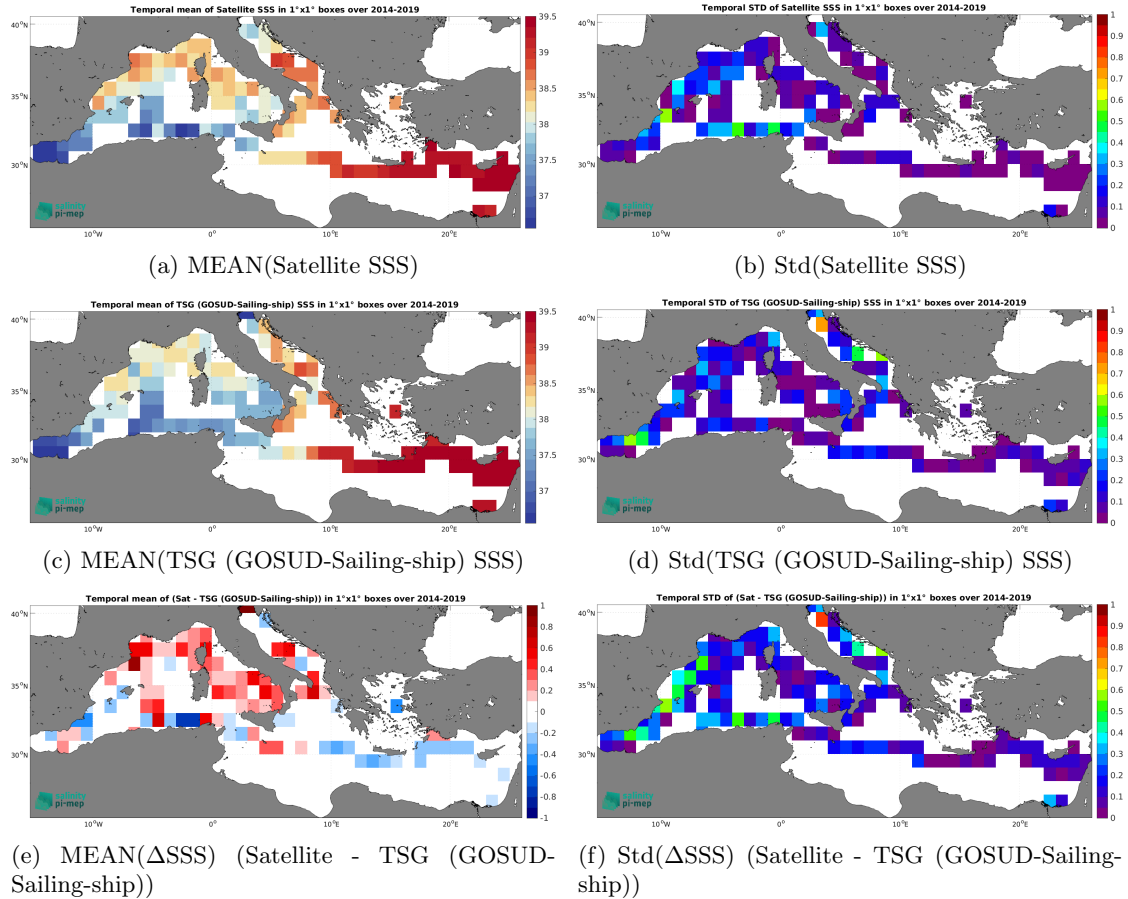
Figure 7: Temporal mean (left) and Std (right) of SSS from SMOS SSS L3 v9 - 18 Days (CATDS-CEC-LOCEAN) (top), TSG (GOSUD-Sailing-ship) (middle), and of \Delta\text{SSS} (Satellite - TSG (GOSUD-Sailing-ship)). Only match-up pairs are used to generate these maps.
