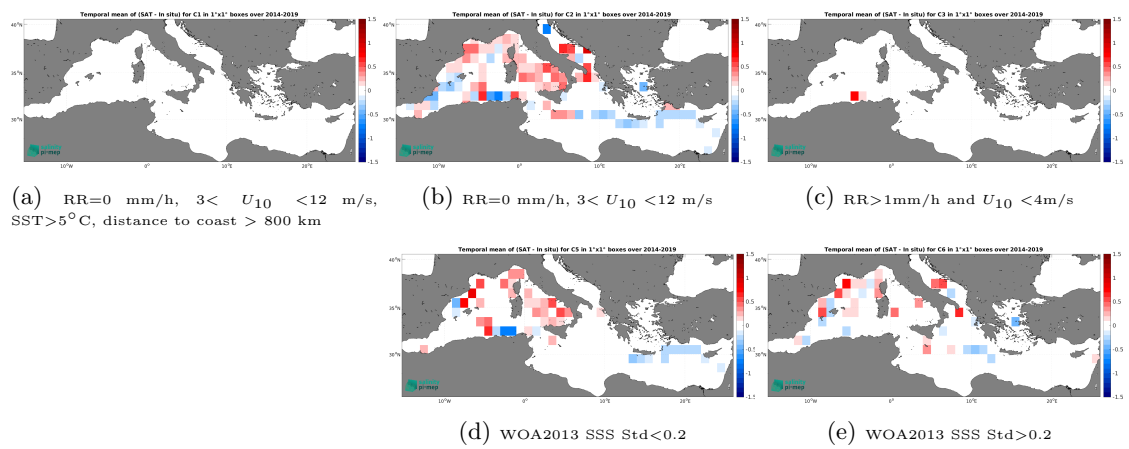
Figure 14: Temporal mean gridded over spatial boxes of size 1^\circ \times 1^\circ of \Delta SSS (SMOS SSS L3 v9 - 18 Days (CATDS-CEC-LOCEAN) - TSG (GOSUD-Sailing-ship)) for 5 different subdatasets corresponding to:RR=0 mm/h, 3 < U_{10} < 12 m/s, SST>5°C, distance to coast > 800 km (a), RR=0 mm/h, 3 < U_{10} < 12 m/s (b), RR>1mm/h and U_{10} < 4 m/s (c), WOA2013 SSS Std<0.2 (d), WOA2013 SSS Std>0.2 (e).
