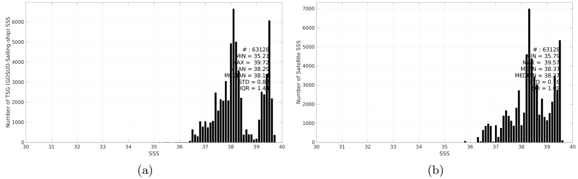
Figure 3: Histograms of SSS from TSG (GOSUD-Sailing-ship) (a) and SMOS SSS L3 v9 - 18 Days (CATDS-CEC-LOCEAN) (b) considering all match-up pairs per bins of 0.1 over the Mediterranean Sea Pi-MEP region and for the full satellite product period.
