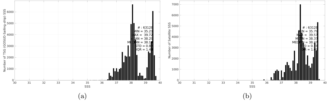
Figure 2: Histograms of SSS from TSG (GOSUD-Sailing-ship) (a) and SMOS SSS L3 v9 - 18 Days (CATDS-CEC-LOCEAN) (b) considering all match-up pairs per bins of 0.1 over the Mediterranean Sea Pi-MEP region and for the full satellite product period.
