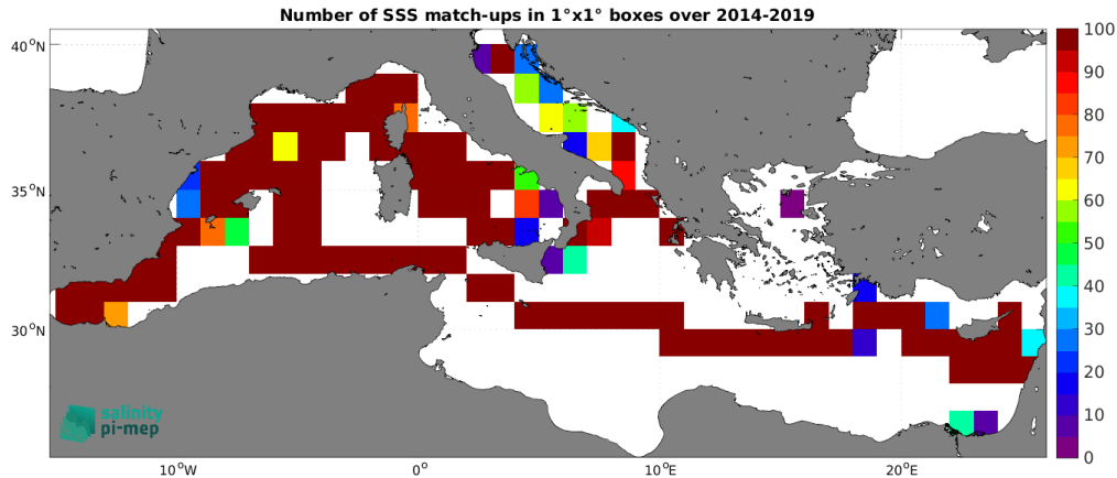
Figure 4: Number of SSS match-ups between TSG (GOSUD-Sailing-ship) SSS and the SMOS SSS L3 v9 - 18 Days (CATDS-CEC-LOCEAN) SSS product for the Mediterranean Sea Pi-MEP region over 1^\circ \times 1^\circ boxes and for the full satellite product period.
