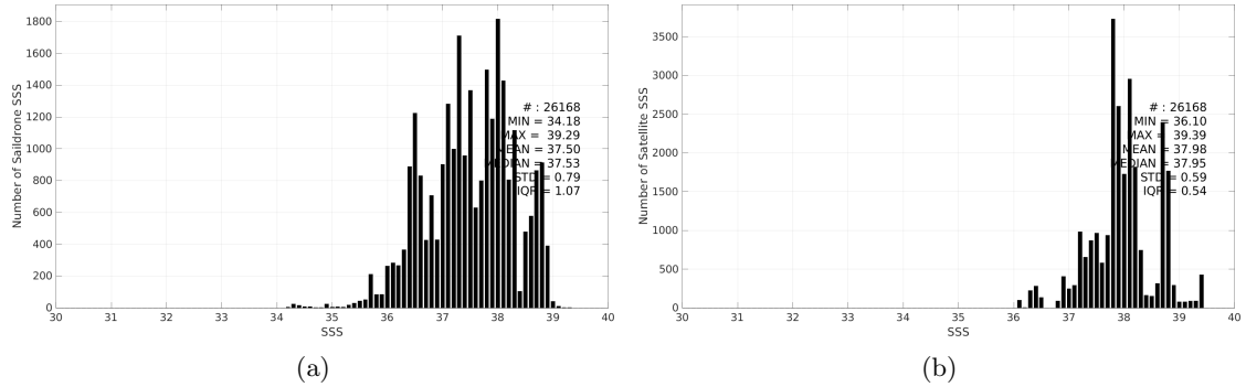
Figure 3: Histograms of SSS from Saildrone (a) and SMOS SSS L3 v9 - 18 Days (CATDS-CEC-LOCEAN) (b) considering all match-up pairs per bins of 0.1 over the Mediterranean Sea Pi-MEP region and for the full satellite product period.
