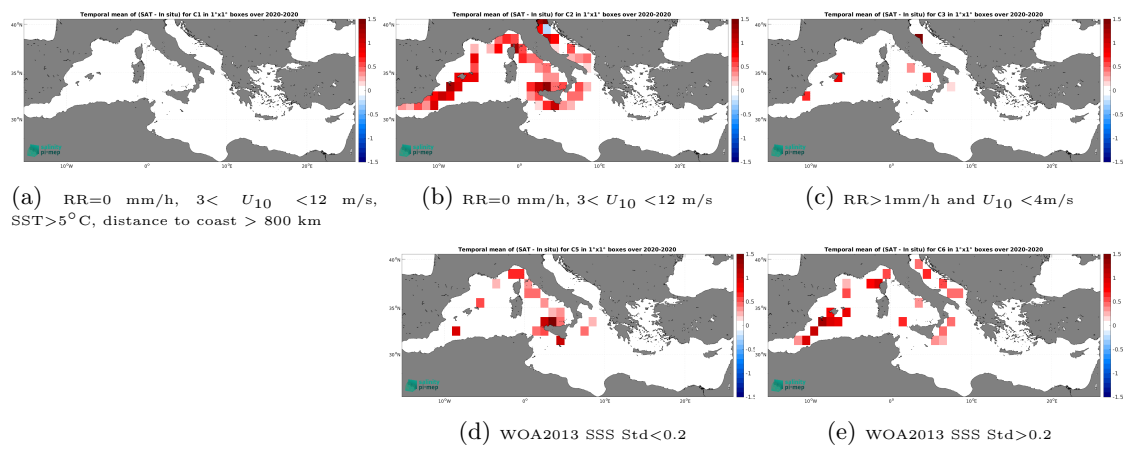
Figure 14: Temporal mean gridded over spatial boxes of size 1^\circ \times 1^\circ of \Delta SSS (SMOS SSS L3 v9 - 18 Days (CATDS-CEC-LOCEAN) - Saildrone) for 5 different subdatasets corresponding to:RR=0 mm/h, 3 < U_{10} < 12 m/s, SST>5°C, distance to coast > 800 km (a), RR=0 mm/h, 3 < U_{10} < 12 m/s (b), RR>1mm/h and U_{10} < 4 m/s (c), WOA2013 SSS Std<0.2 (d), WOA2013 SSS Std>0.2 (e).
