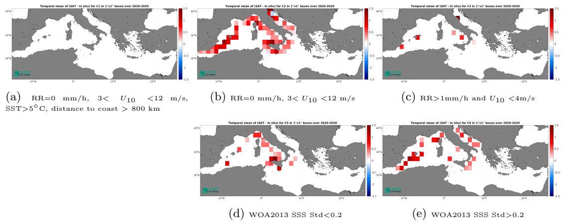
Figure 14: Temporal mean gridded over spatial boxes of size 1^\circ \times 1^\circ of \Delta SSS (SMOS SSS L3 v9 - 18 Days (CATDS-CEC-LOCEAN) - Saildrone) for 5 different subdatasets corresponding to:RR=0 mm/h, 3 < U_{10} < 12 m/s, SST>5°C, distance to coast > 800 km (a), RR=0 mm/h, 3 < U_{10} < 12 m/s (b), RR>1mm/h and U_{10} < 4 m/s (c), WOA2013 SSS Std<0.2 (d), WOA2013 SSS Std>0.2 (e).
