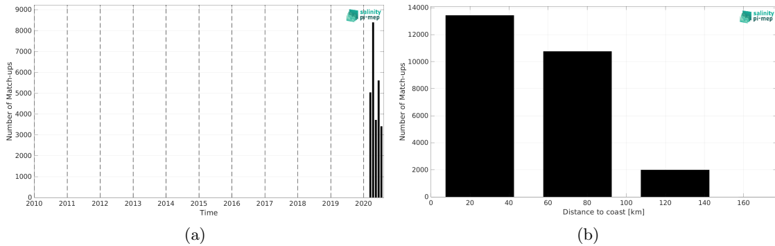
Figure 1: Number of match-ups between Saildrone and SMOS SSS L3 v9 - 18 Days (CATDS-CEC-LOCEAN) SSS as a function of time (a) and as function of the distance to coast (b) over the Mediterranean Sea Pi-MEP region and for the full satellite product period.
