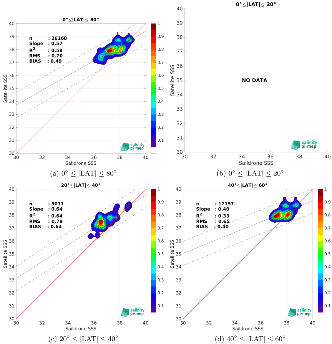
Figure 9: Contour maps of the concentration of SMOS SSS L3 v9 - 18 Days (CATDS-CEC-LOCEAN) SSS (y-axis) versus Sailldrone SSS (x-axis) at match-up pairs for different latitude bands. For each plot, the red line shows x=y . The black thin and dashed lines indicate a linear fit through the data cloud and the \pm 95\% confidence levels, respectively. The number match-up pairs n , the slope and R^2 coefficient of the linear fit, the root mean square (RMS) and the mean bias between satellite and in situ data are indicated for each latitude band in each plots.
