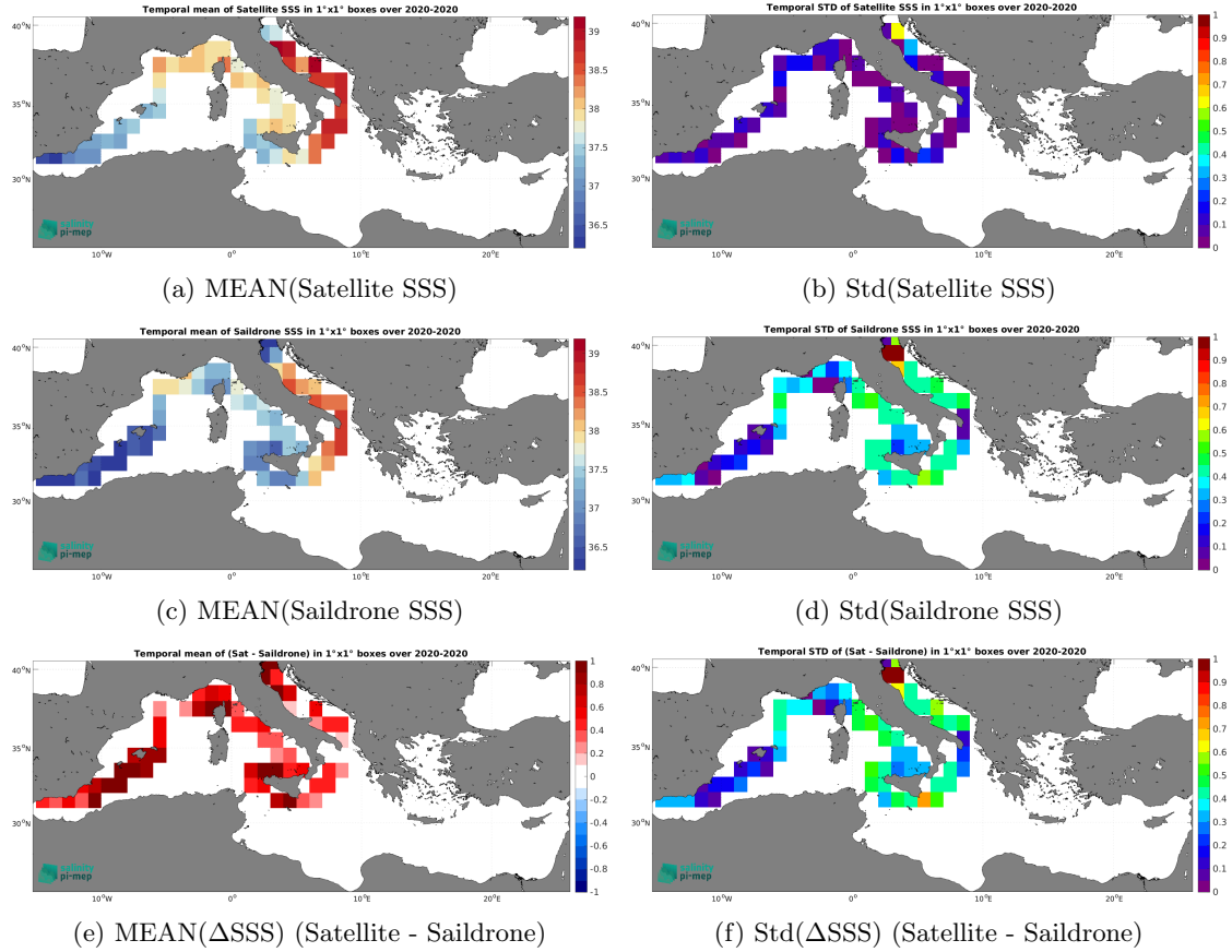
Figure 6: Temporal mean (left) and Std (right) of SSS from SMOS SSS L3 v9 - 18 Days (CATDS-CEC-LOCEAN) (top), Sairdrone (middle), and of \Delta SSS (Satellite - Sairdrone). Only match-up pairs are used to generate these maps.
