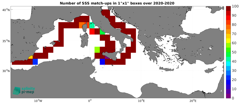
Figure 4: Number of SSS match-ups between Saildrone SSS and the SMOS SSS L3 v9 - 18 Days (CATDS-CEC-LOCEAN) SSS product for the Mediterranean Sea Pi-MEP region over 1^\circ \times 1^\circ boxes and for the full satellite product period.
