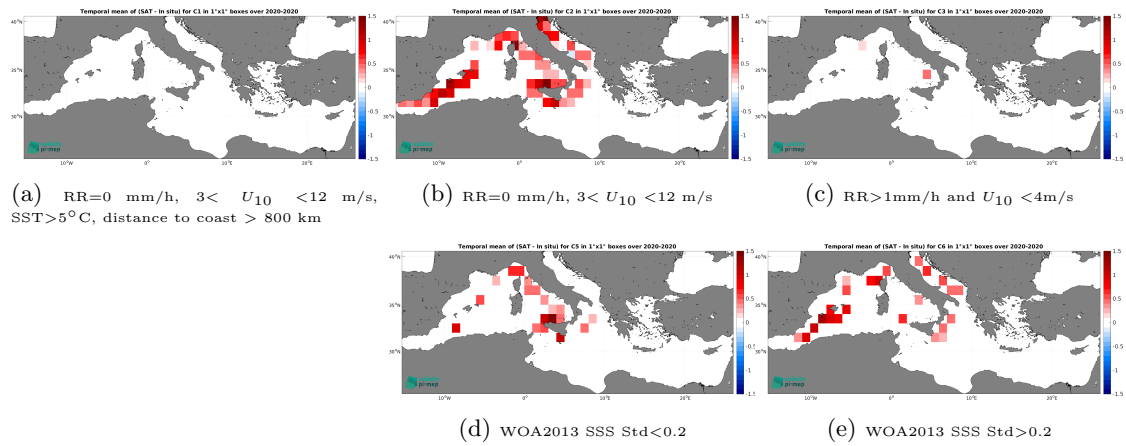
Figure 12: Temporal mean gridded over spatial boxes of size 1^\circ \times 1^\circ of \Delta SSS (SMOS SSS L3 v9 - 18 Days (CATDS-CEC-LOCEAN) - Saildrone) for 5 different subdatasets corresponding to:RR=0 mm/h, 3 < U_{10} < 12 m/s, SST >5^\circ\text{C} , distance to coast > 800 km (a), RR=0 mm/h, 3 < U_{10} < 12 m/s (b), RR >1 mm/h and U_{10} < 4 m/s (c), WOA2013 SSS Std <0.2 (d), WOA2013 SSS Std >0.2 (e).
