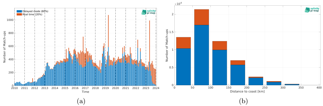
Figure 2: Number of match-ups between Argo and SMOS SSS L3 v9 - 18 Days (CATDS-CEC-LOCEAN) SSS as a function of time (a) and as function of the distance to coast (b) over the Mediterranean Sea Pi-MEP region and for the full satellite product period.
