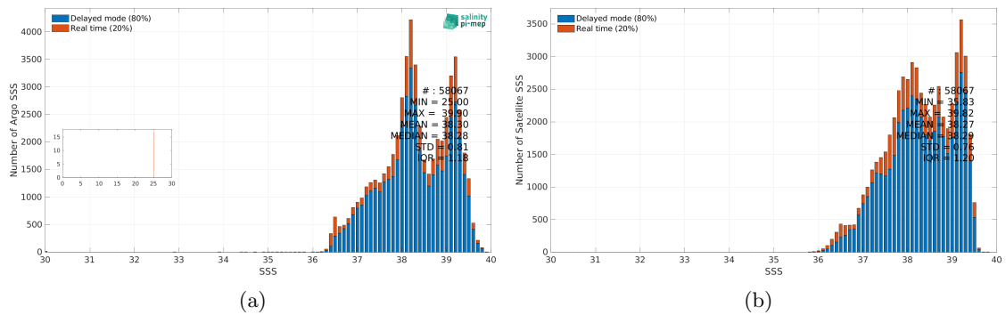
Figure 3: Histograms of SSS from Argo (a) and SMOS SSS L3 v9 - 18 Days (CATDS-CEC-LOCEAN) (b) considering all match-up pairs per bins of 0.1 over the Mediterranean Sea Pi-MEP region and for the full satellite product period.
